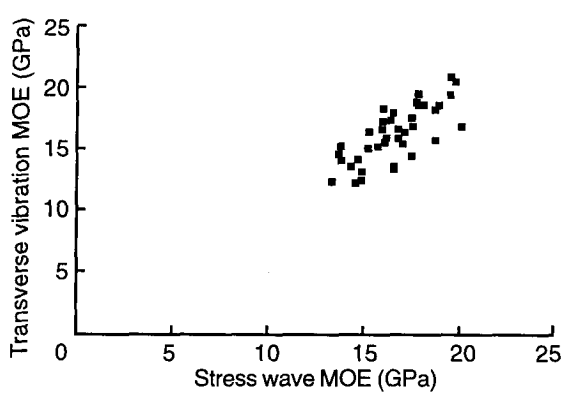
Figure 8—Relationship between stress wave and transverse vibration MOE for individual laminations. Note that the stress wave MOE was determined for the laminations after deck construction by a digital storage oscilloscope.
