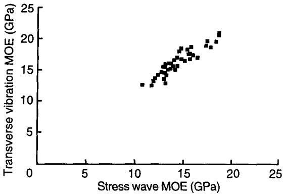
Figure 6—Relationship between stress wave and transverse vibration MOE for individual laminations prior to deck construction. Note that stress wave MOE was determined by an oscilloscope.
