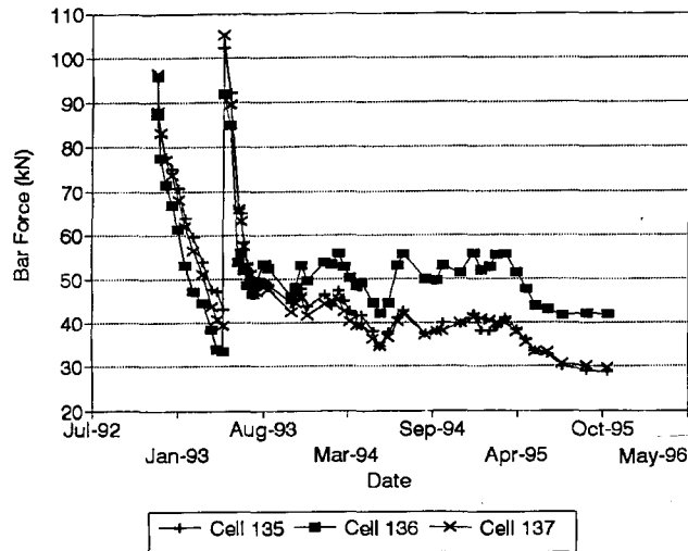
Figure 4—Average trend in bar tension force.
