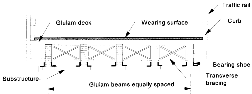
Roadway section
