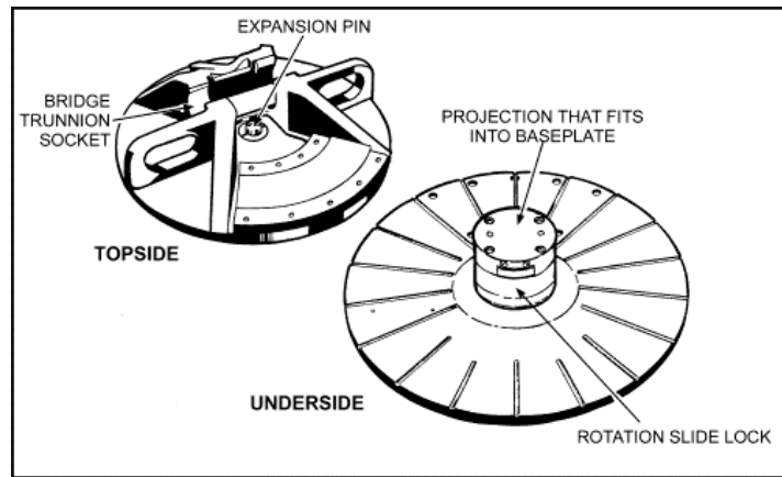
Figure 6-6. Rotator assembly.
