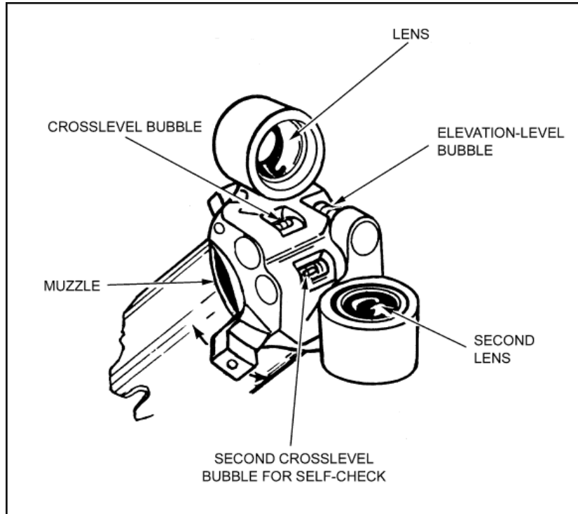
Figure 2-17. Boresight, M115.
