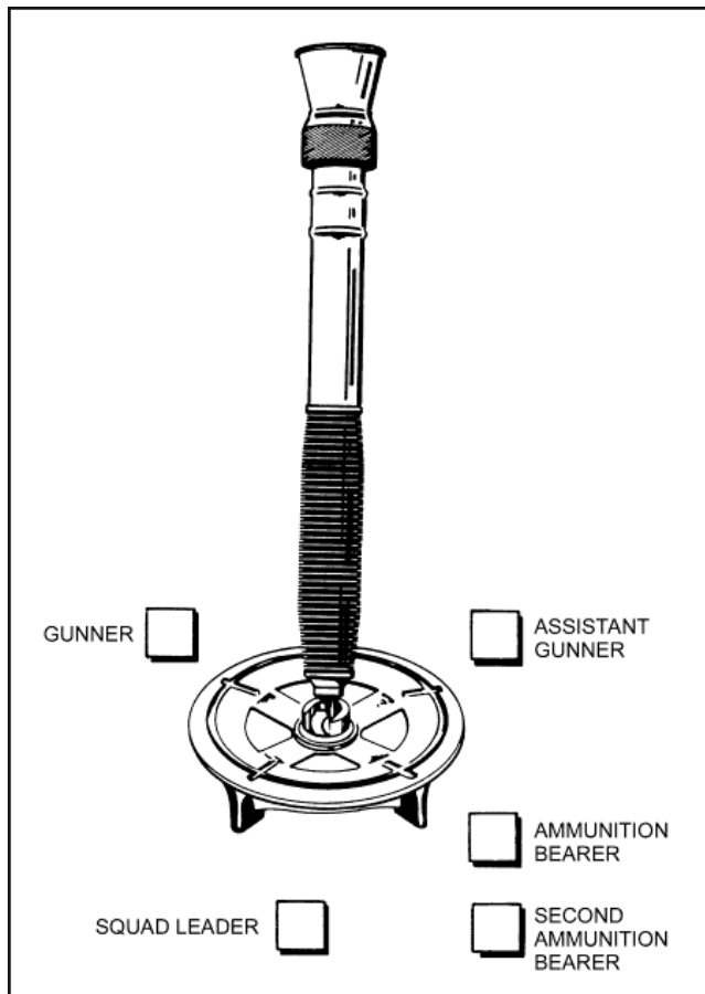
Figure 4-1. Position of squad members.
