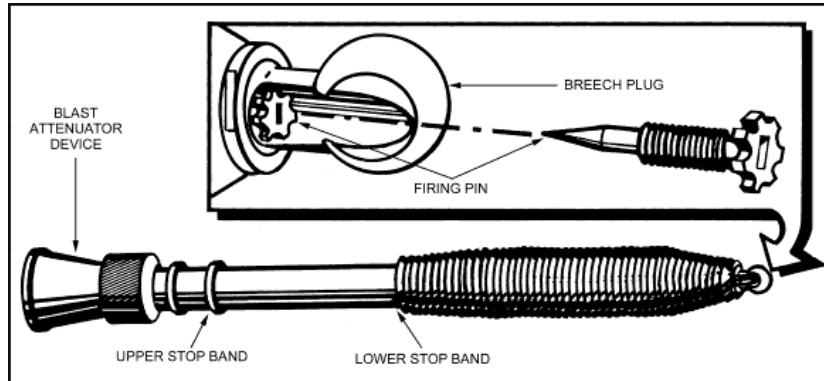
Figure 4-3. Cannon assembly, M253.
