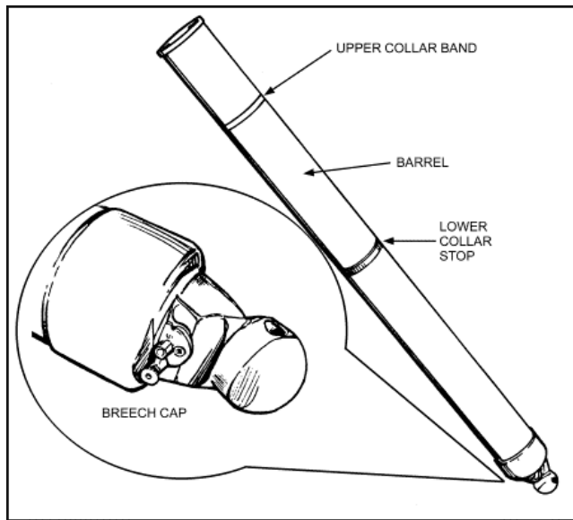
Figure 7-3. Barrel assembly, M298.
