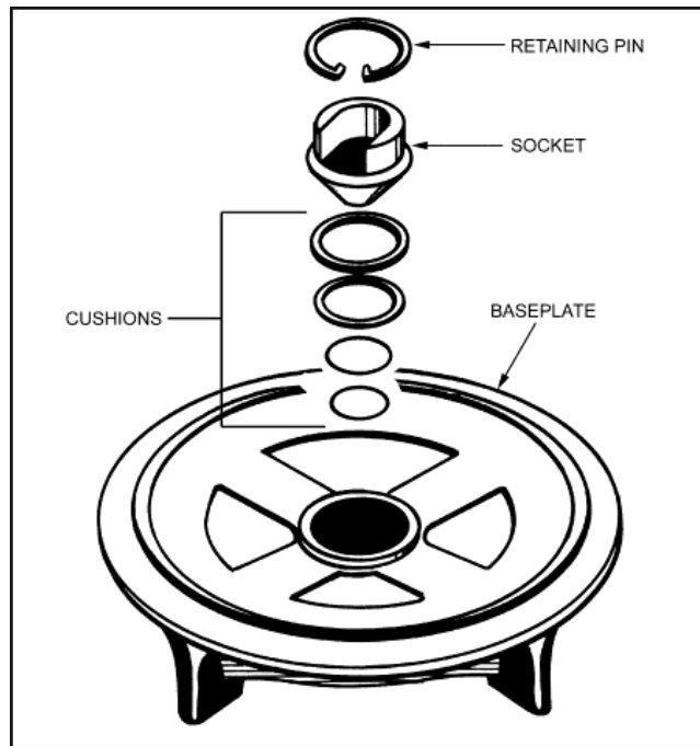
Figure 4-5. Baseplate, M3A1.
