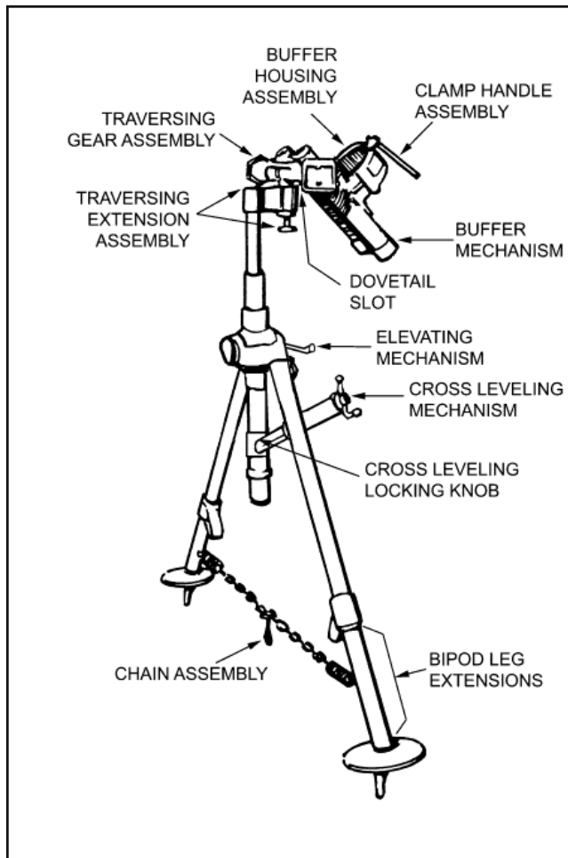
Figure 7-4. Bipod assembly, M191 (carrier/ground-mounted).
