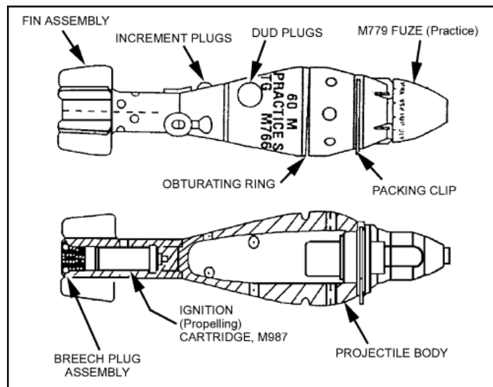
Figure 3-12. M766 (SRTR) cartridge.
