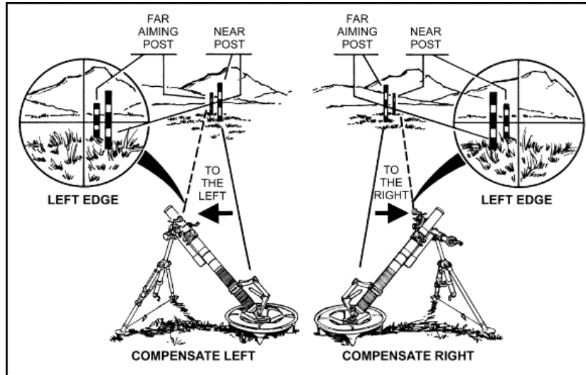
Figure 3-7. Compensated sight picture.
