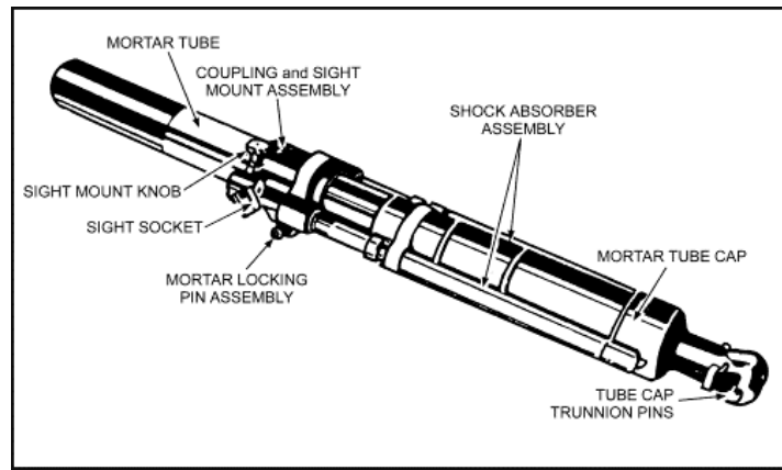
Figure 6-3. Cannon, M30.
