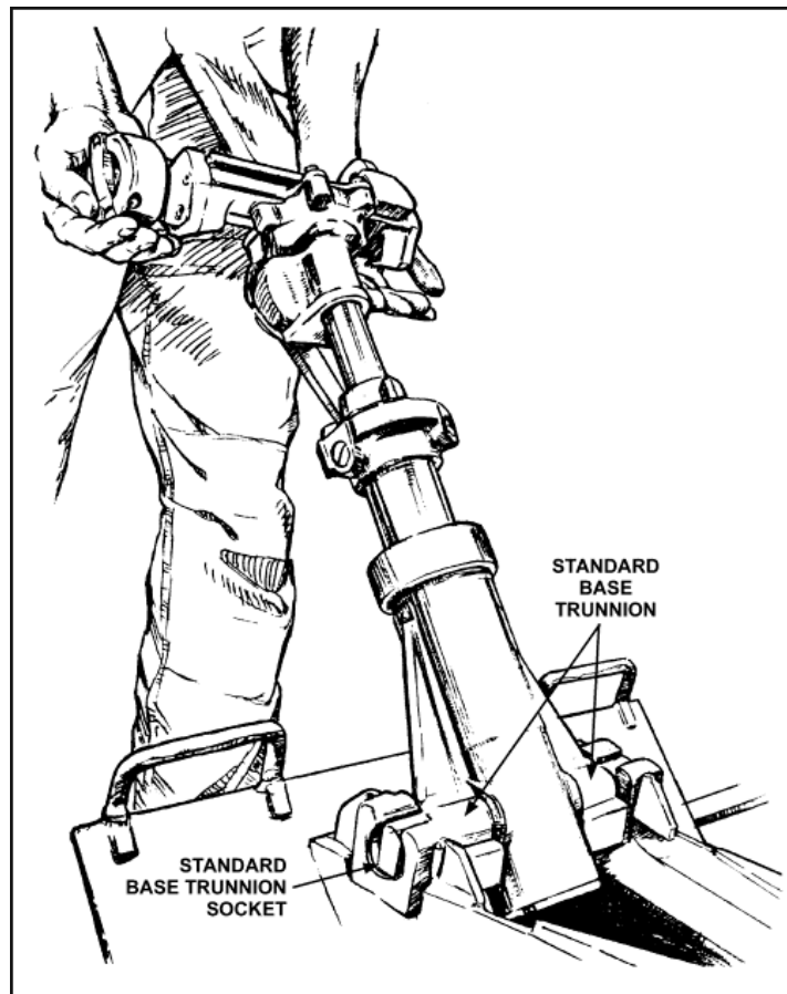
Figure 6-9. Installation of standard assembly.
