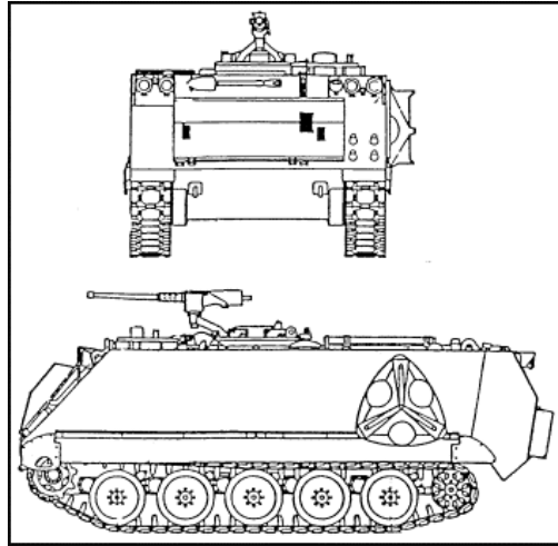
Figure 7-7. Mortar carrier M1064A3, front and side view.
