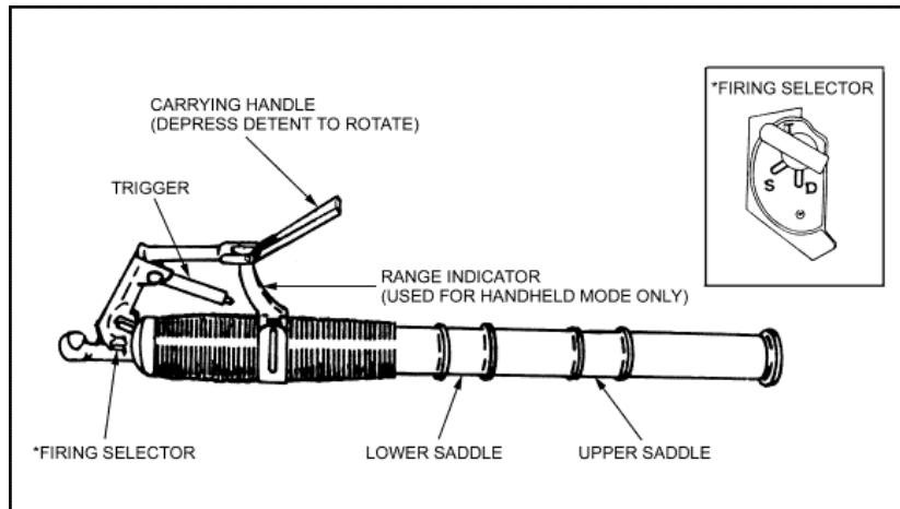
Figure 3-2. Cannon assembly, M225.
