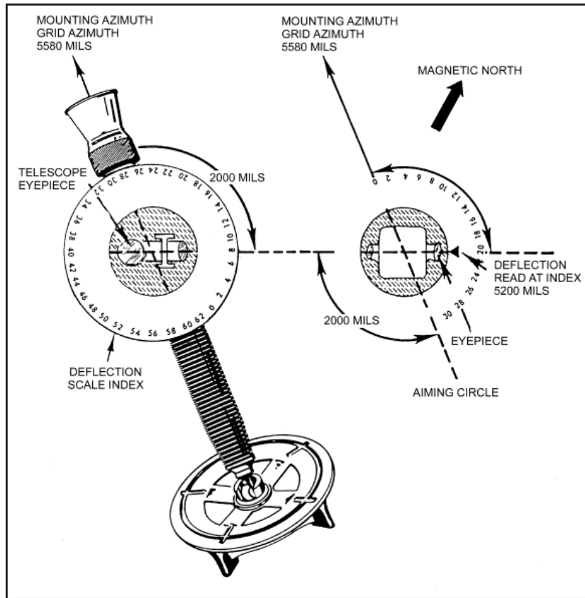
Figure 2-28. Mortar laid parallel with the aiming circle.
