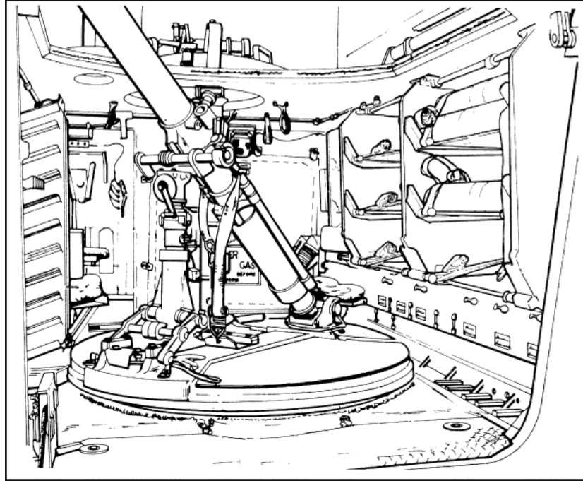
Figure 6-18. Vehicular mount.
