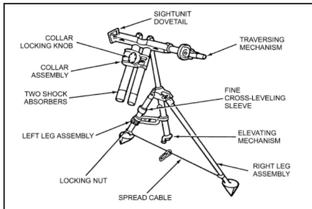
Figure 3-5. Bipod assembly, M170.
