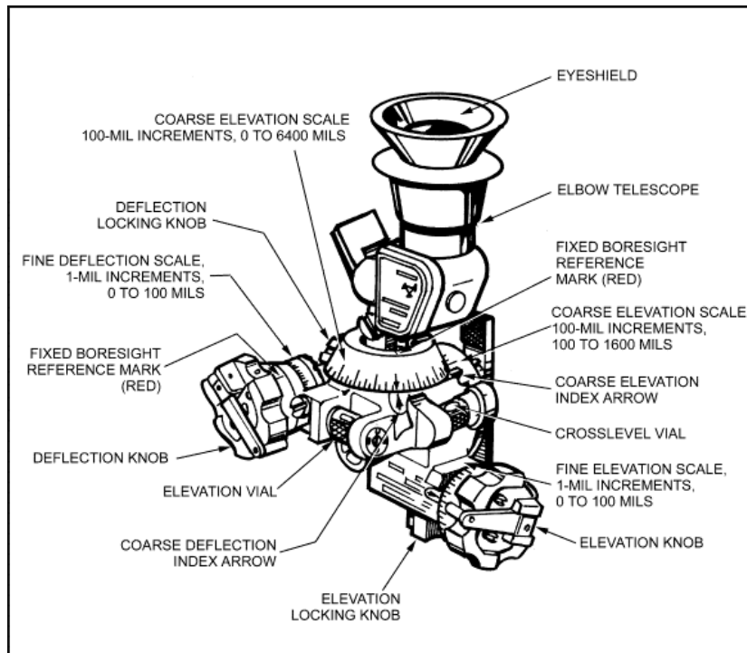
Figure 2-13. Sightunit, M64-series.
