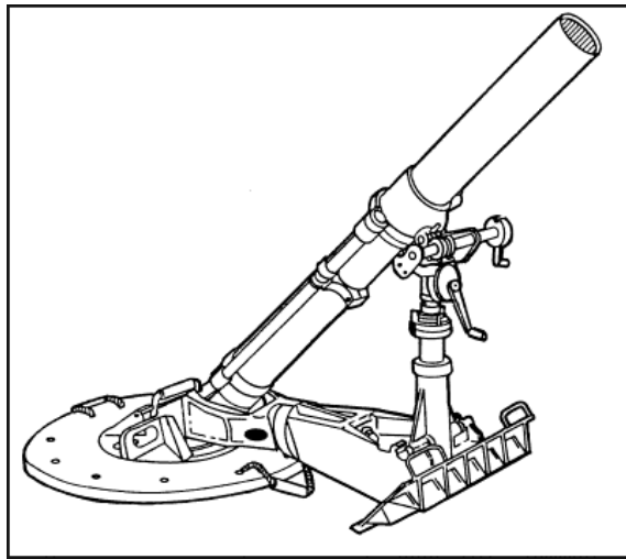
Figure 6-2. 4.2-inch mortar, M30.
