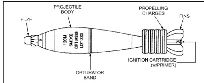
Figure 7-14. M929 smoke cartridge.
