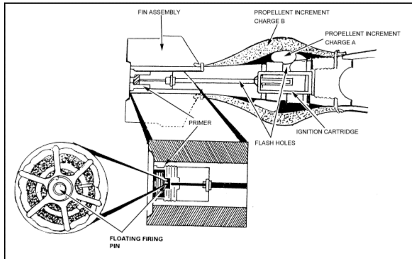
Figure 4-9. Floating firing pin.
