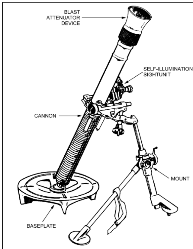
Figure 4-2. The 81-mm mortar, M252.
