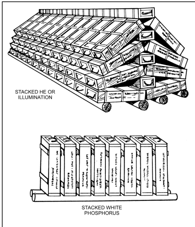
Figure 1-3. Stacked ammunition.
