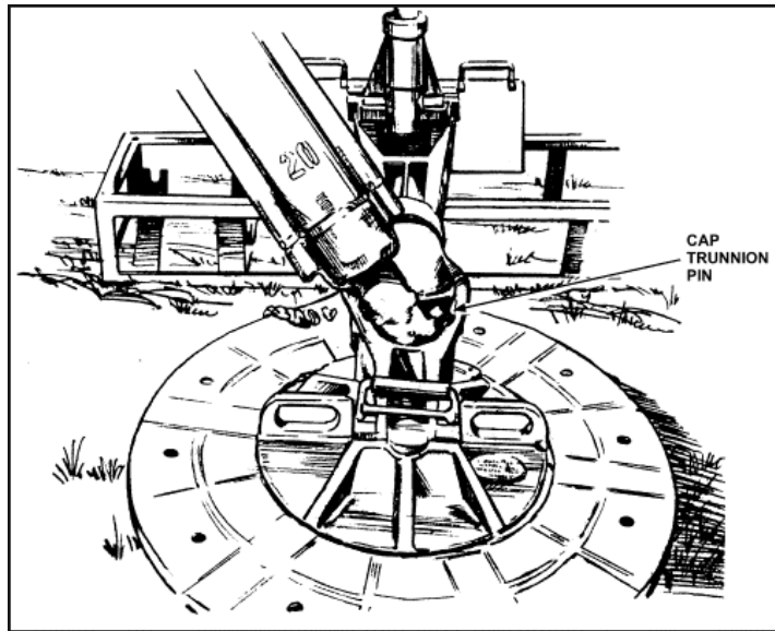
Figure 6-10. Barrel positioned into the bridge assembly.
