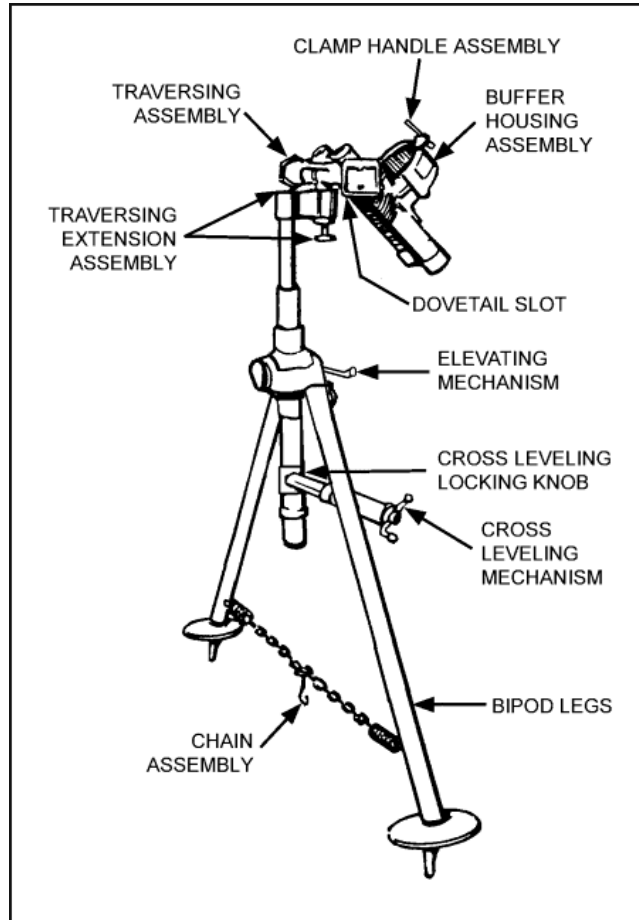
Figure 7-5. Bipod assembly, M190 (ground-mounted).
