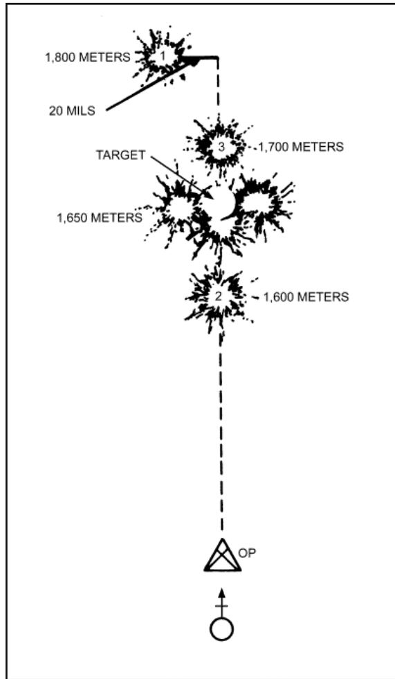
Figure 8-4. Bracketing method.
