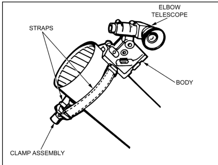
Figure 2-16. Boresight, M45.
