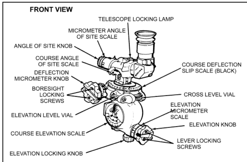
Figure 2-11. Sightunit, M53.
