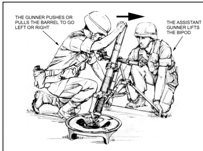
Figure 3-6. Large deflection and elevation changes.
