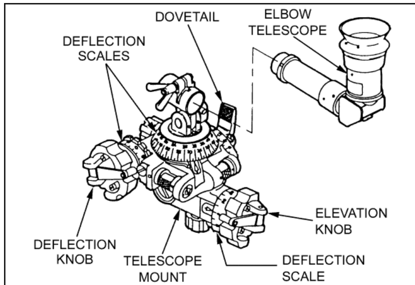
Figure 2-15. M67 sightunit.
