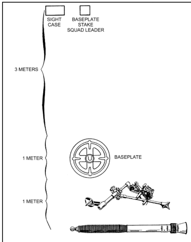
Figure 4-6. Layout of equipment.
