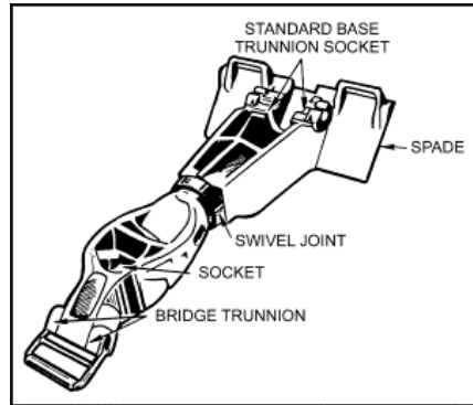
Figure 6-5. Bridge assembly.
