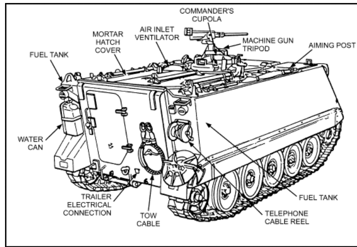
Figure 6-16. Mortar carrier, M106, top rear view.
