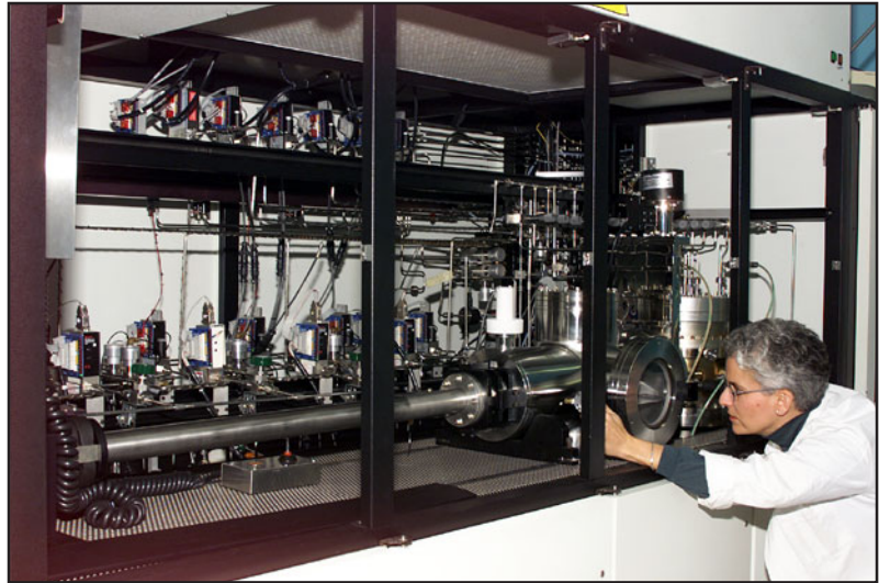
A MOCVD reactor in the MOCVD Laboratory
