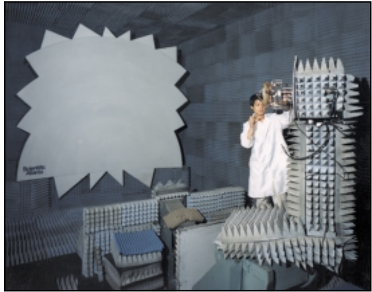
Compact Antenna Range Facility
