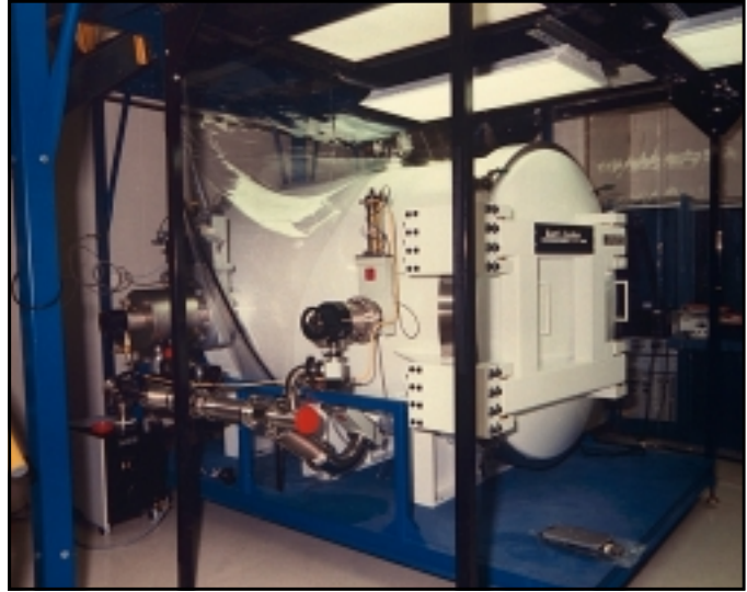
Vacuum Ultraviolet Calibration/Testing Facility
