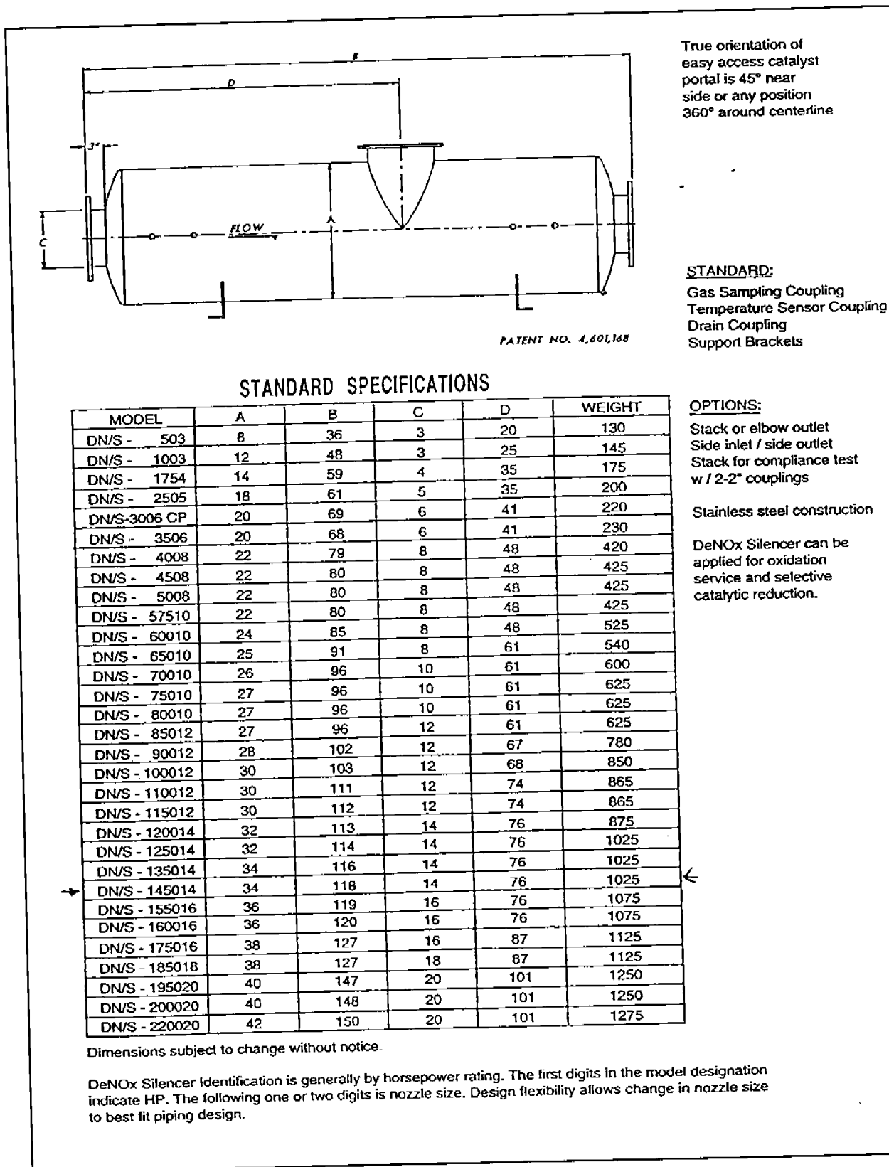
Figure 2C.4. DeNOx Silencer specifications.
