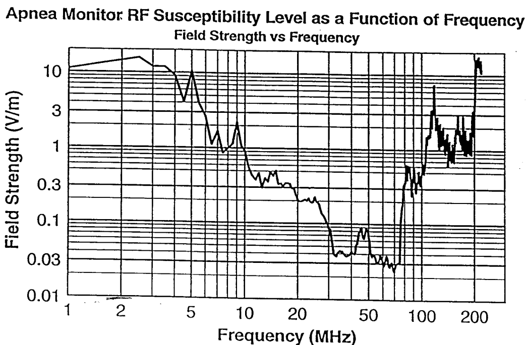
Figure 2. Susceptibility spectrum of an apnea monitor
