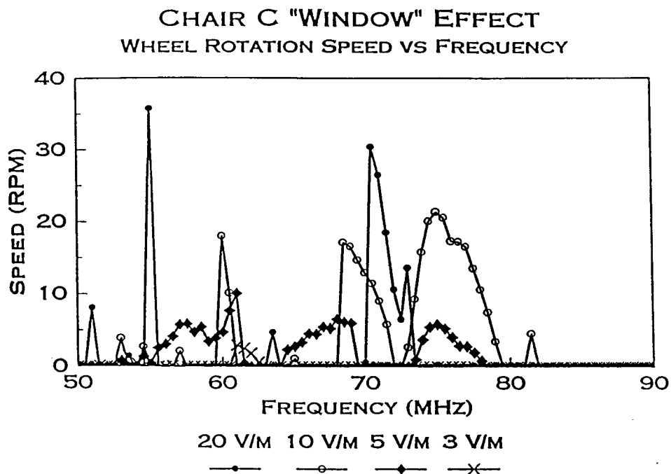
Figure 3. Susceptibility spectra, at various field strengths, of a powered wheelchair
