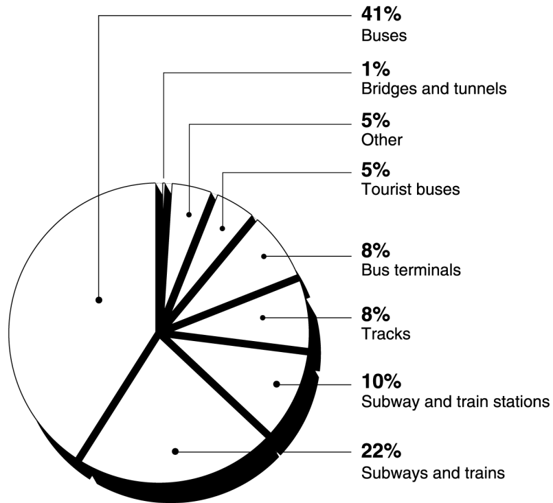
Figure 1: Targets of Attacks on Public Surface Transportation Systems Worldwide, 1997 to 2000
