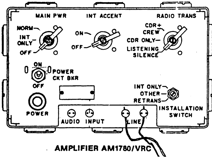
Figure D-6. AM/1780 AMPLIFIER.
