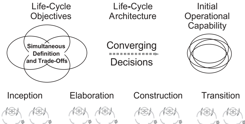
Figure 4: EPIC Phases
