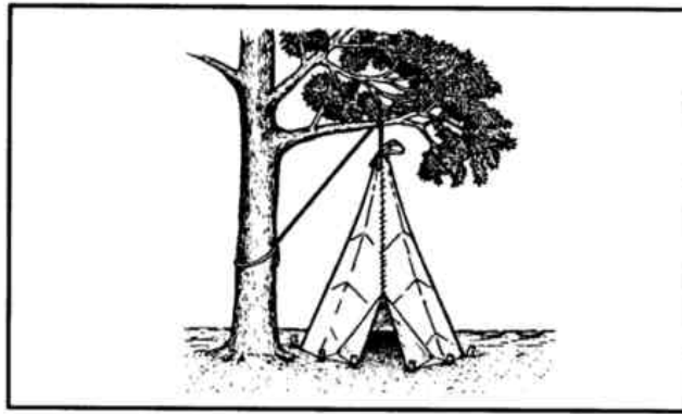
Figure 5-6. No-pole parachute tepee.
