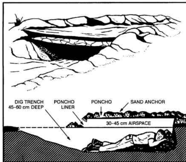
Figure 5-14. Belowground desert shelter.
