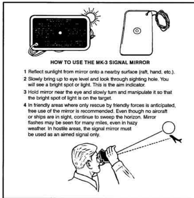
Figure 19-3. Signal mirror.
