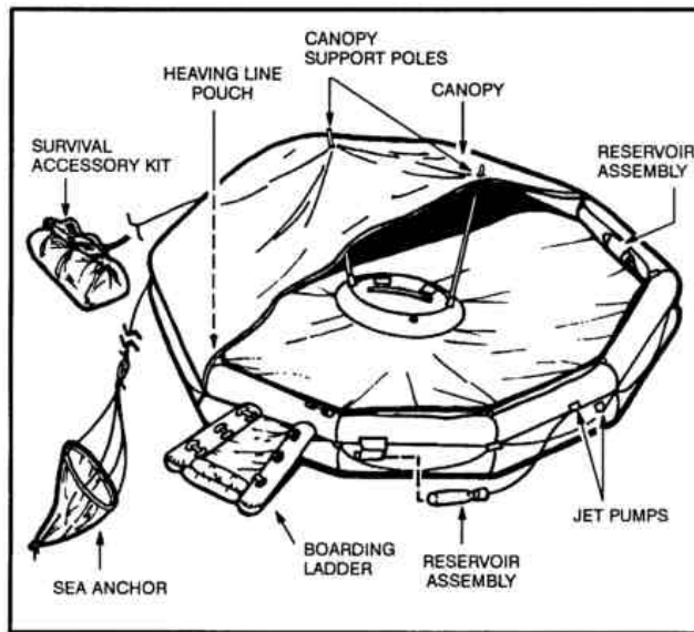
Figure 16-16. Twenty-five-man raft.
