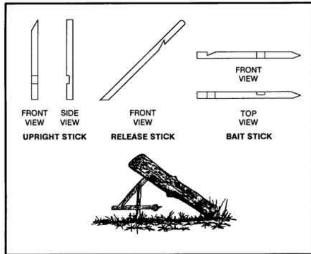
Figure 8-12. Figure 4 deadfall.
