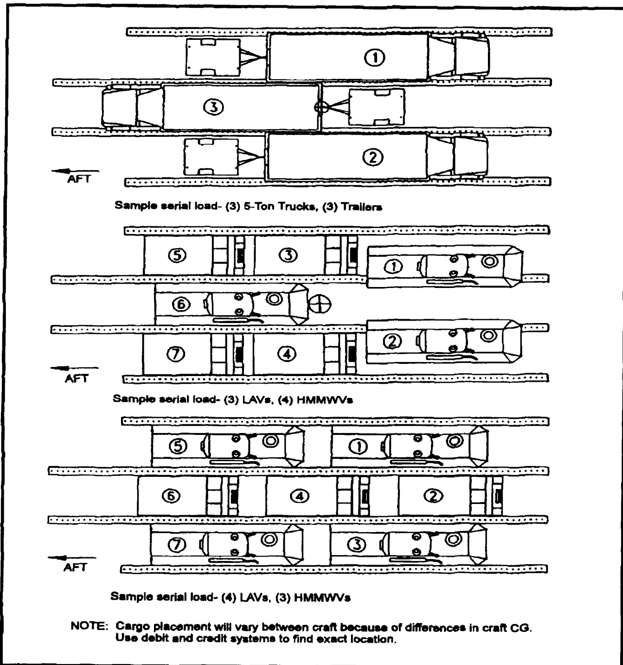
Figure C-7. LCAC Standard Loads and Standard Load Equivalents (Sheet 4 of 4)
