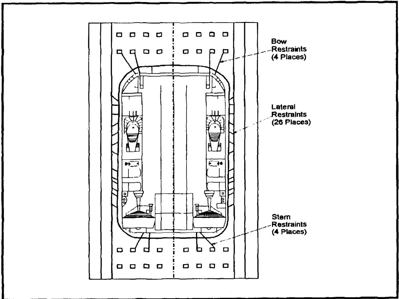
Figure A-7. LCAC Tiedown in Well Deck
