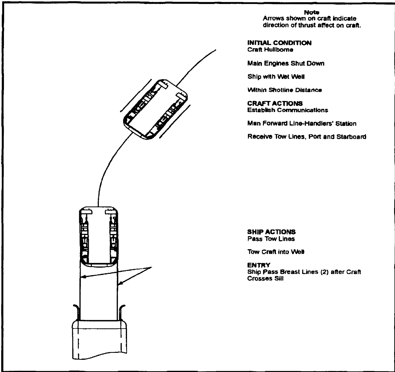
Figure A-6. LCAC Emergency Well Deck Recovery
