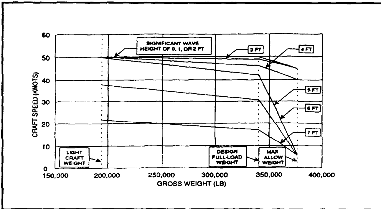
Figure 1-6. Maximum Allowable Speed to Avoid Structural Damage
