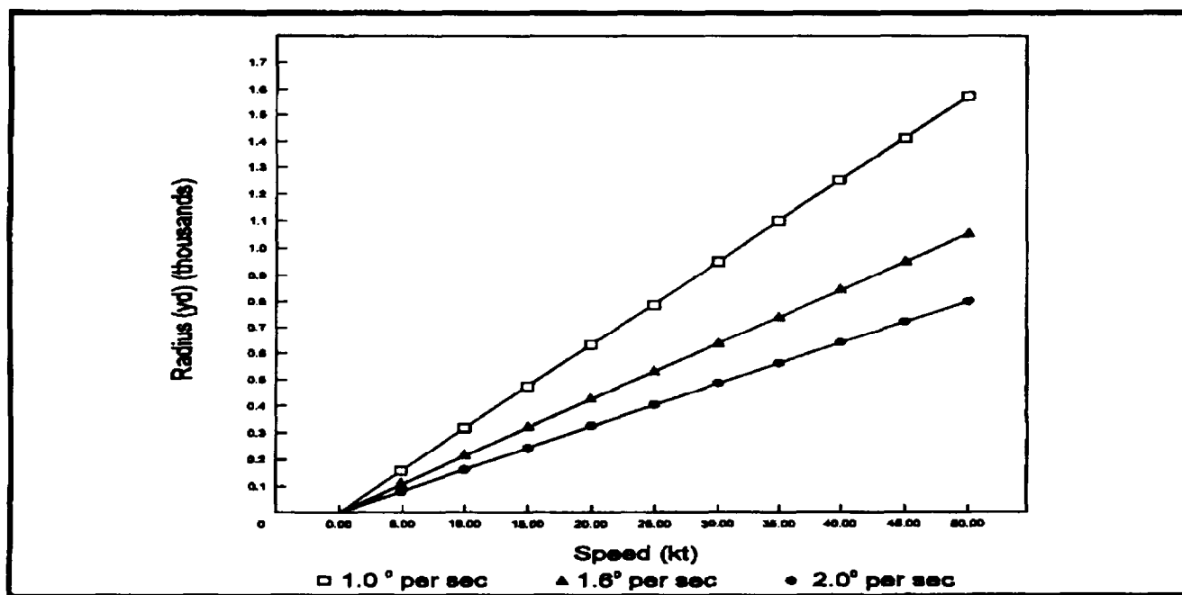
Figure 4-12. Estimated Turn Radii for Various Turn Rates (Sideslip Neglected)
