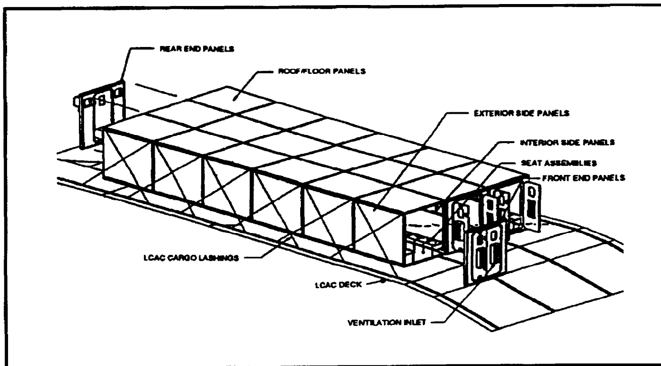
Figure 7-5. Six-Section PTM-Configured LCAC with Major Components
