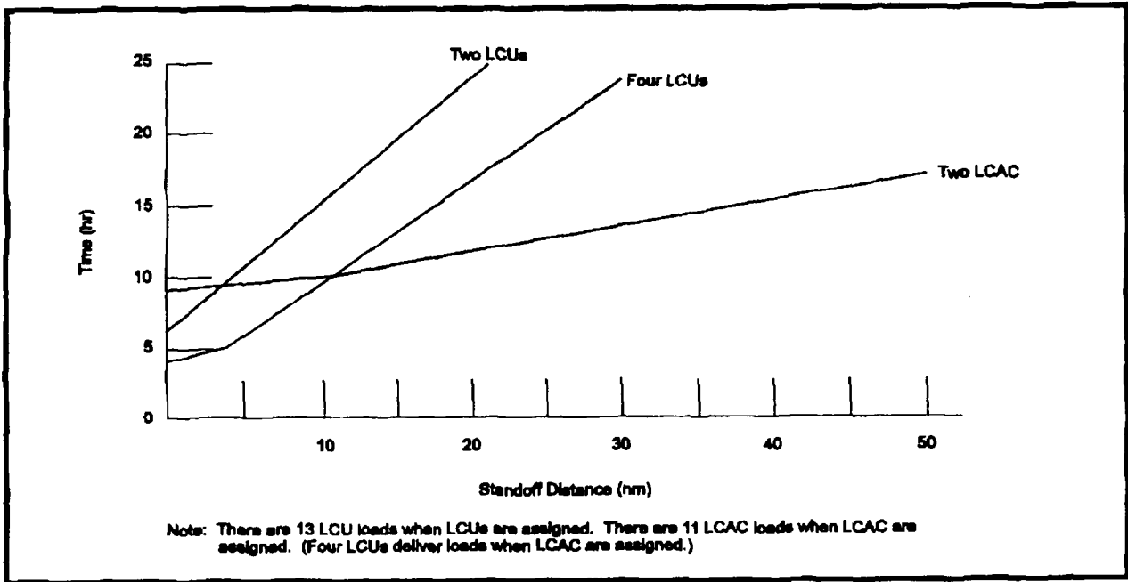
Figure B-8. Estimated Time to Offload an LHA by LCU or LCAC (LCU Deliver LCU Preloads When LCAC Assigned)
