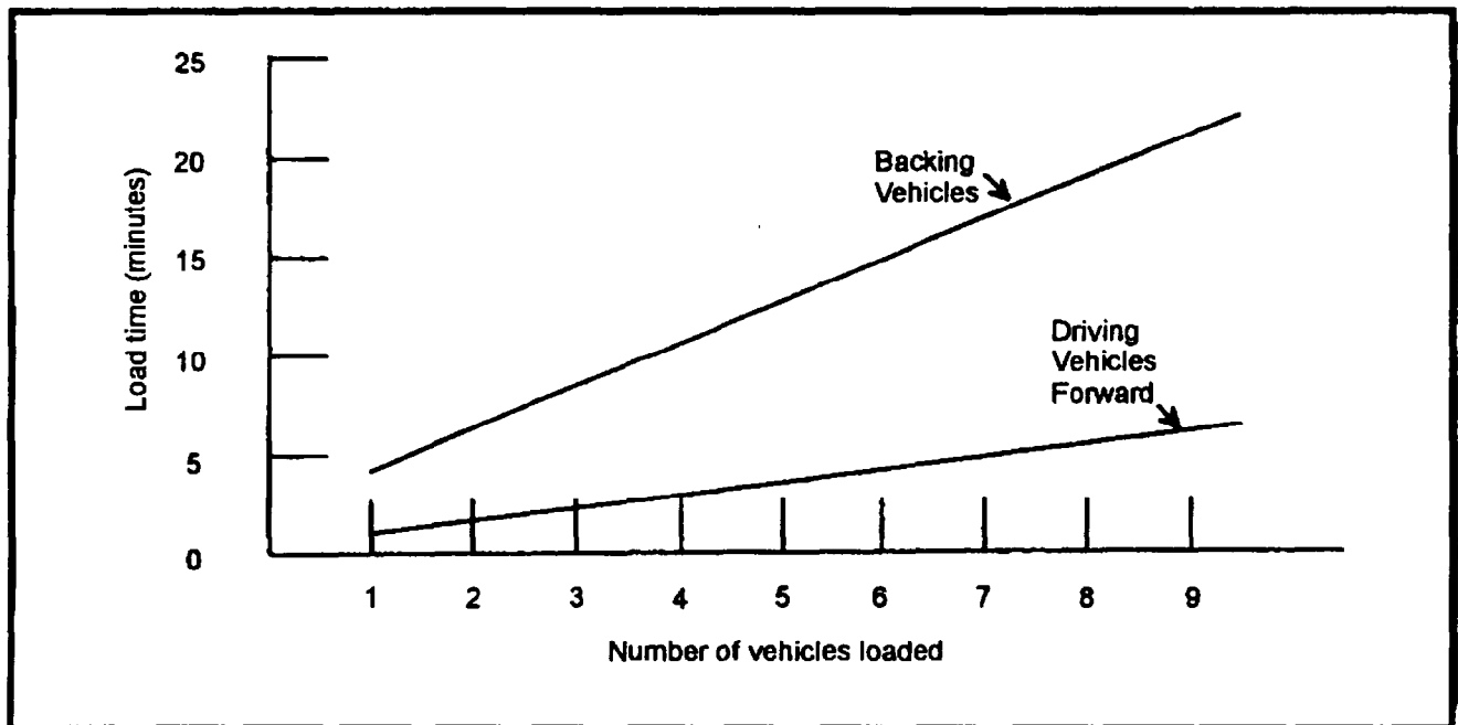
Figure C-5. Estimating Times for Backing Versus Driving Vehicles Forward onto LCAC
