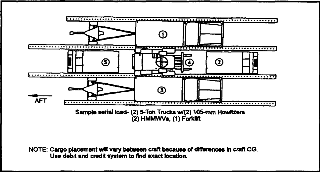
Figure C-7. LCAC Standard Loads and Standard Load Equivalents (Sheet 1 of 4)
