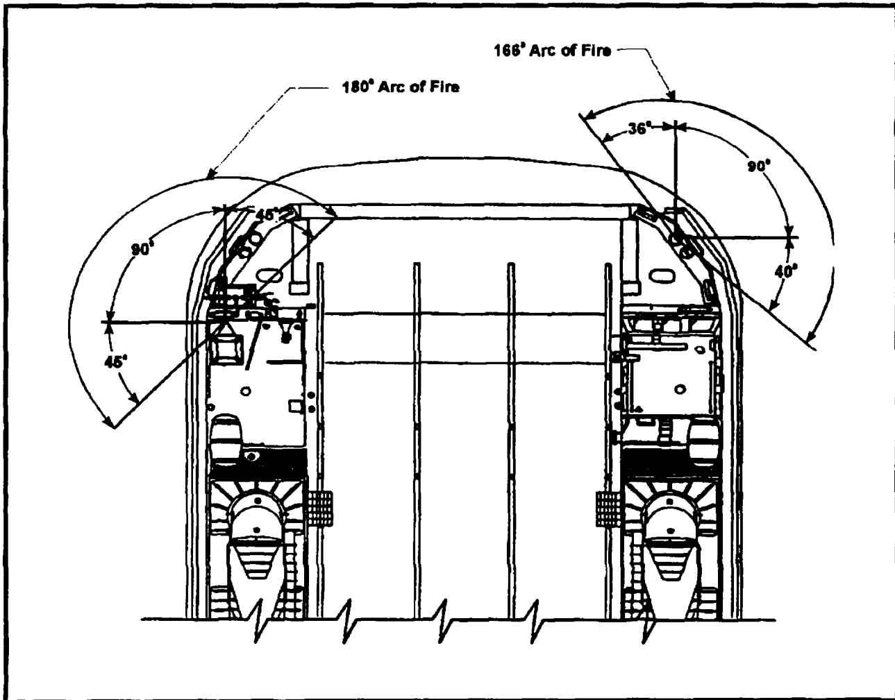
Figure 5-2. LCAC 1 Through 33 Firing Arcs
