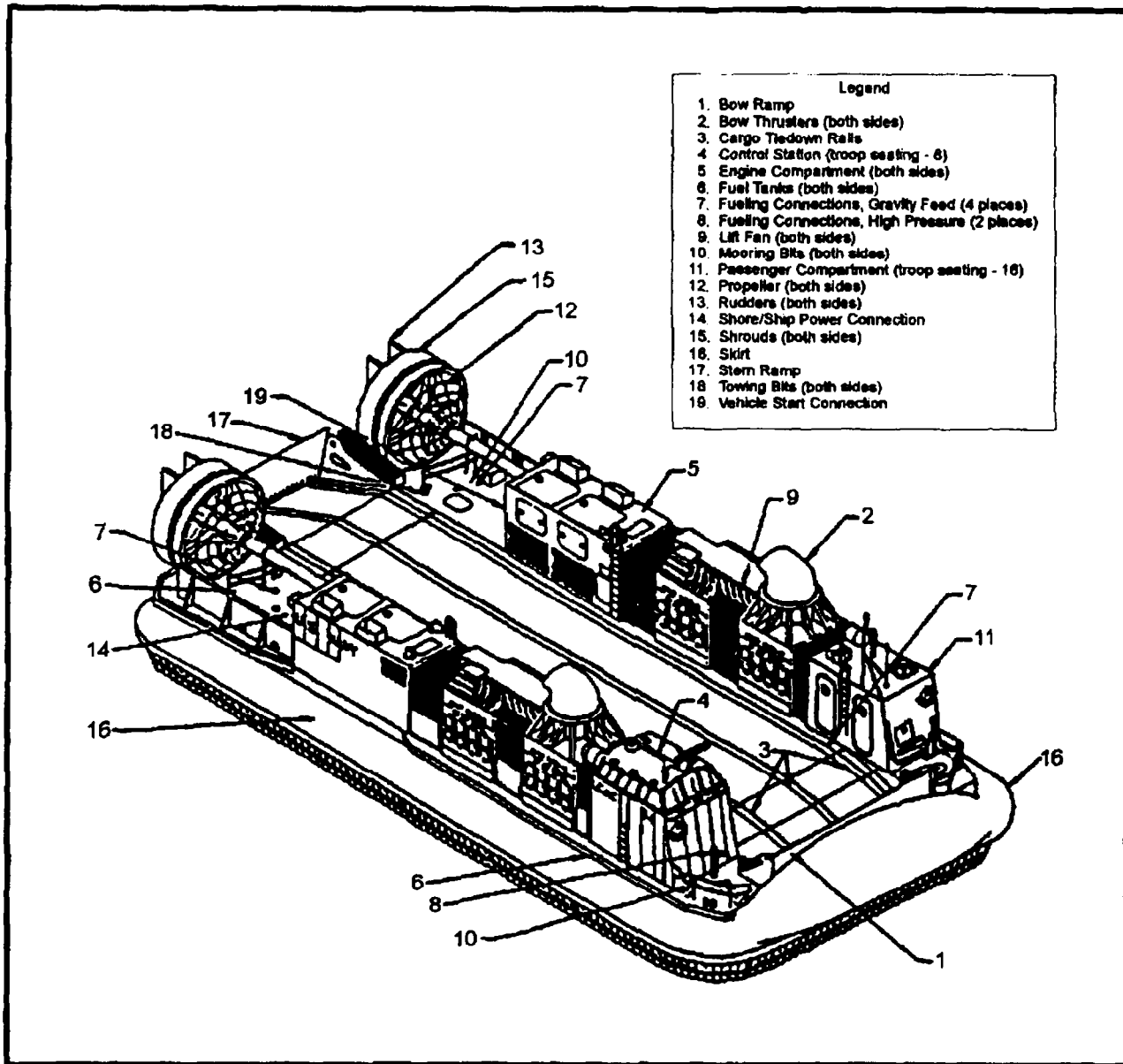
Figure A-1. LCAC Primary Features
