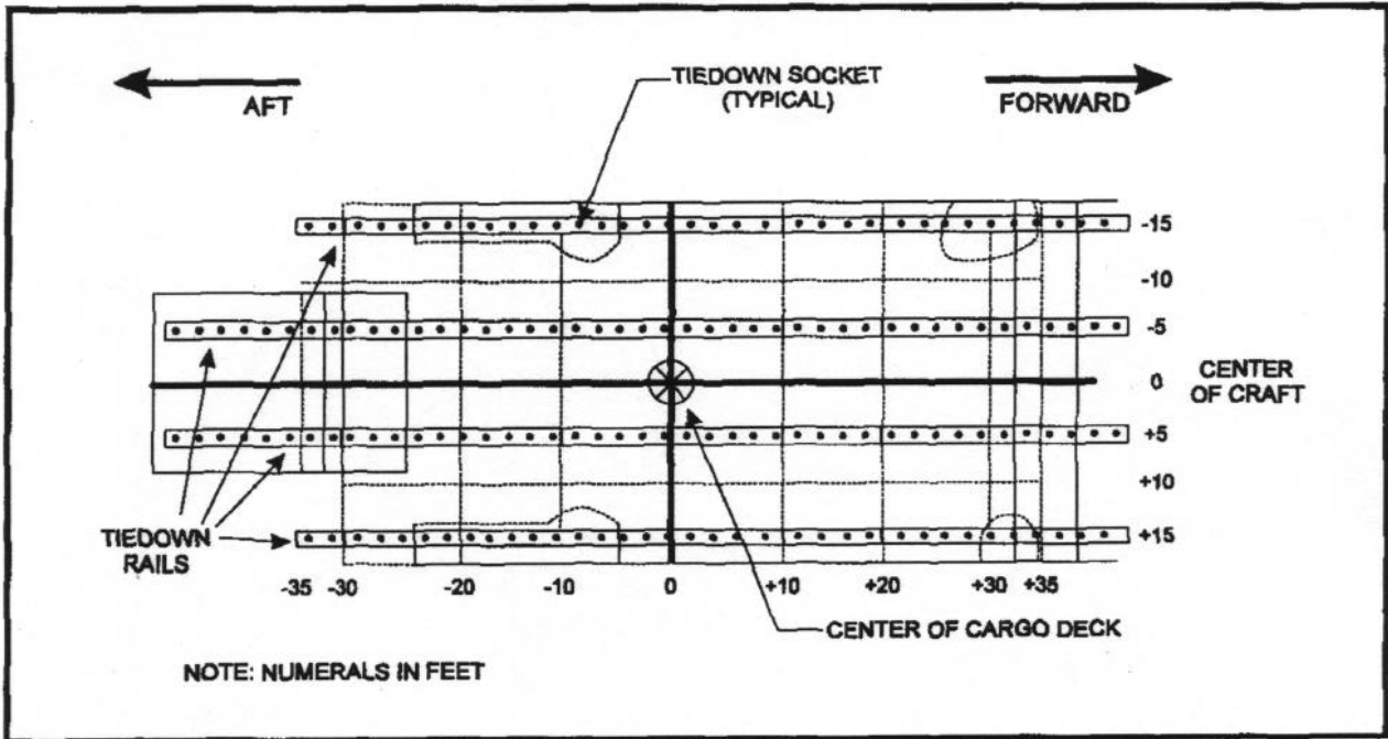
Figure C-2. LCAC Cargo Deck Grid
