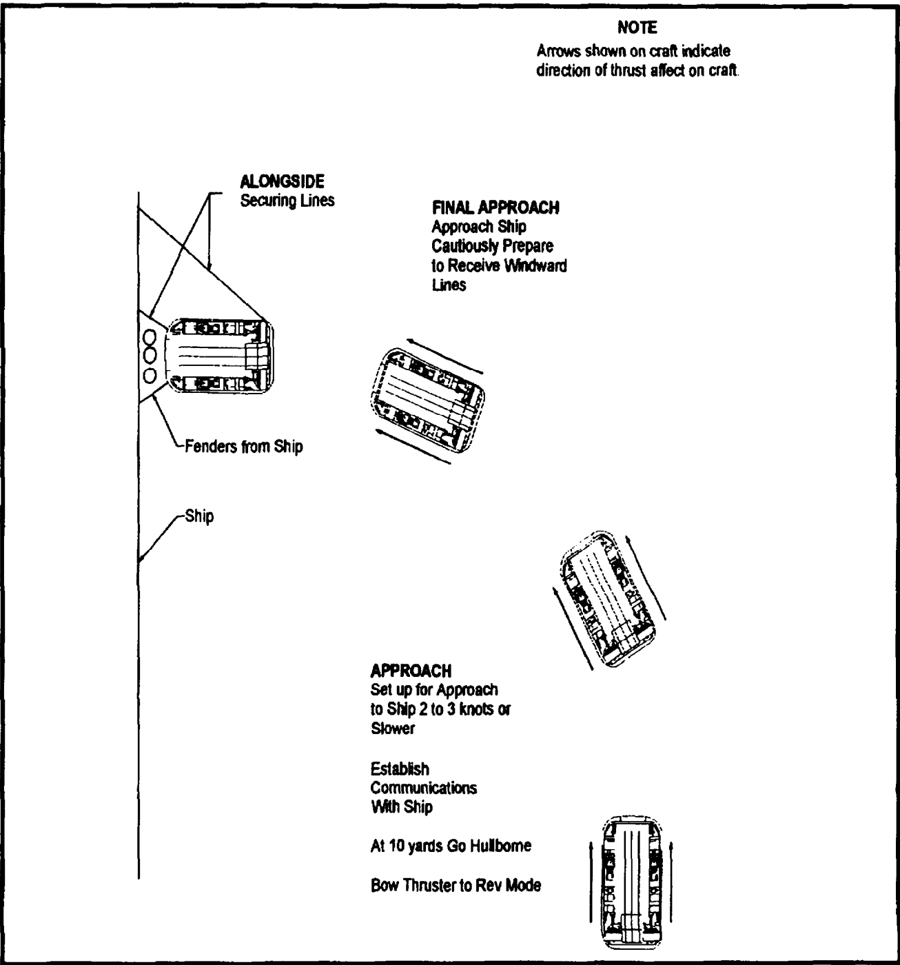
Figure A-8. LCAC Mooring to a Ship
