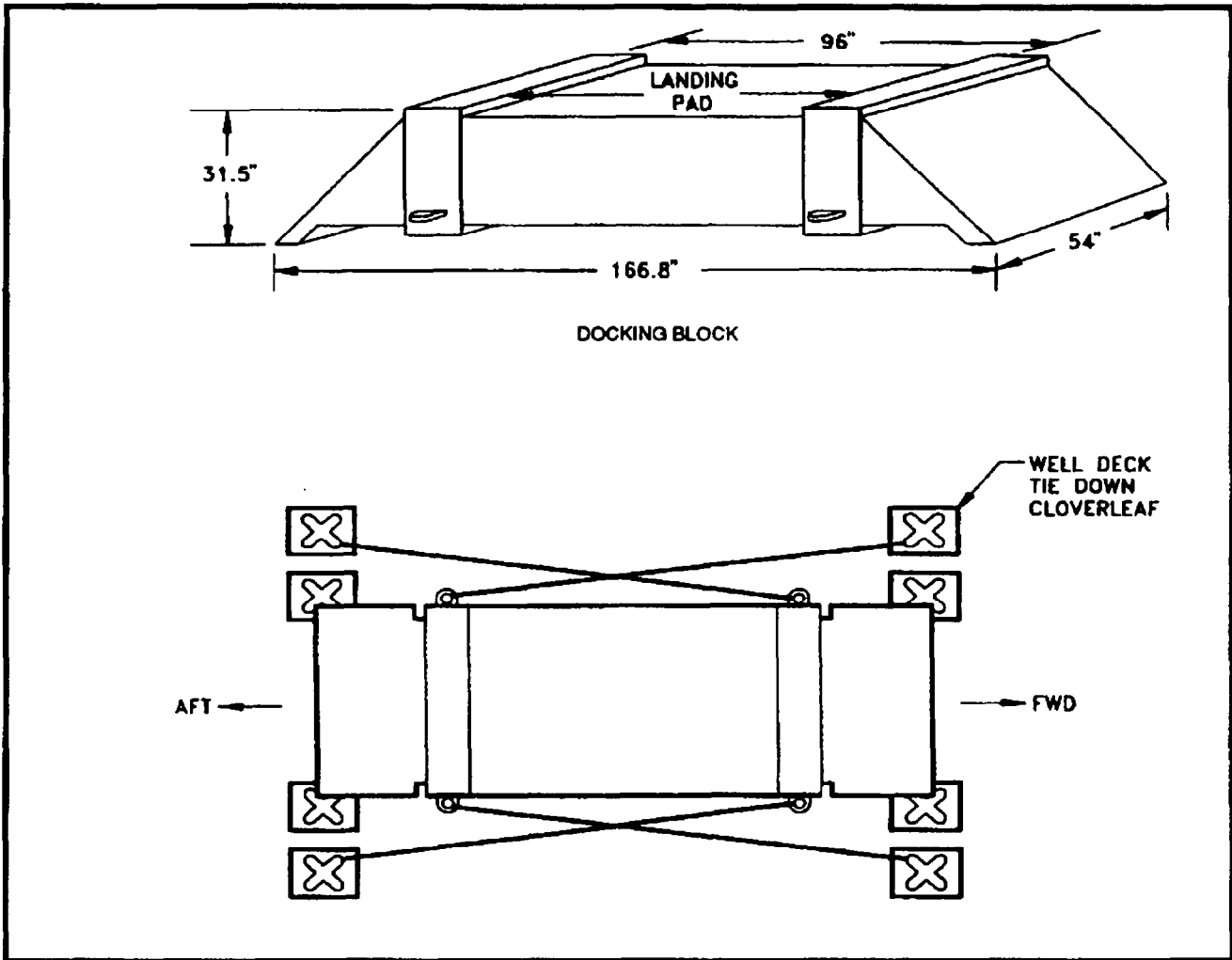
Figure A-5. LCAC Docking Block and a Typical Tiedown Configuration
