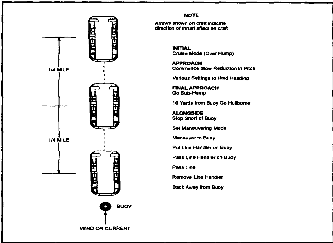
Figure A-10. LCAC Mooring to a Buoy
