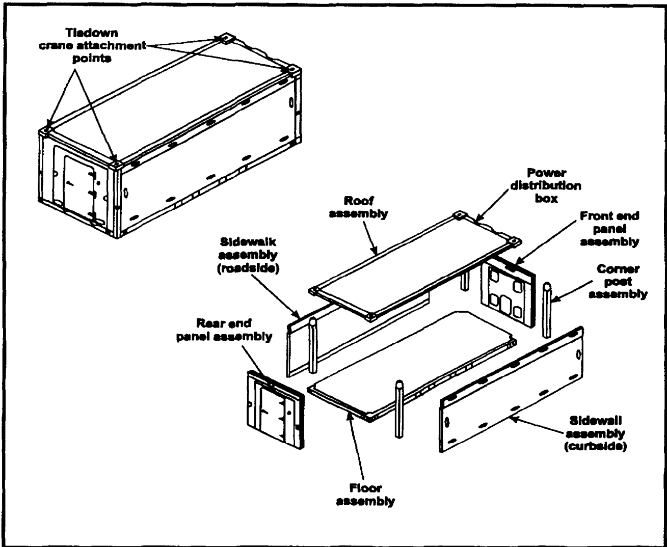
Figure 7-2. Knockdown MCESS Shelter and Major Components
