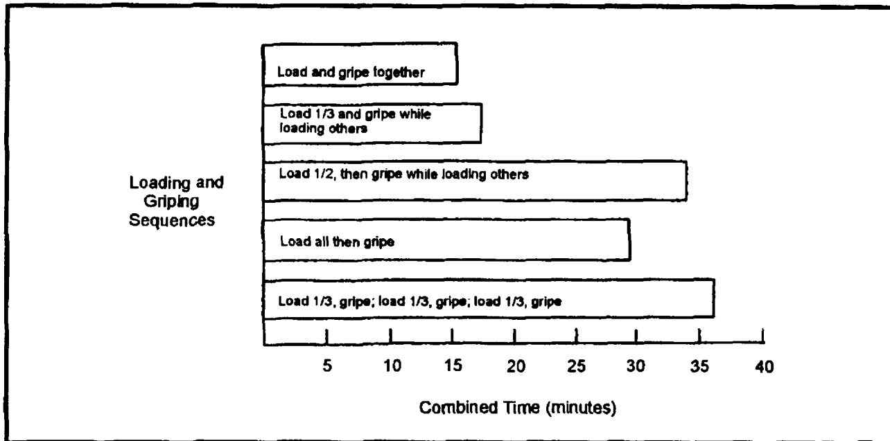
Figure C-6. Combined Times for Various LCAC Loading and Gripping Sequences
