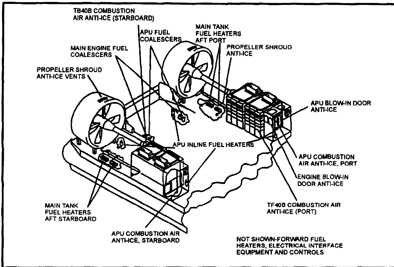
Figure A-3. LCAC Cold Weather Kit Component Location
