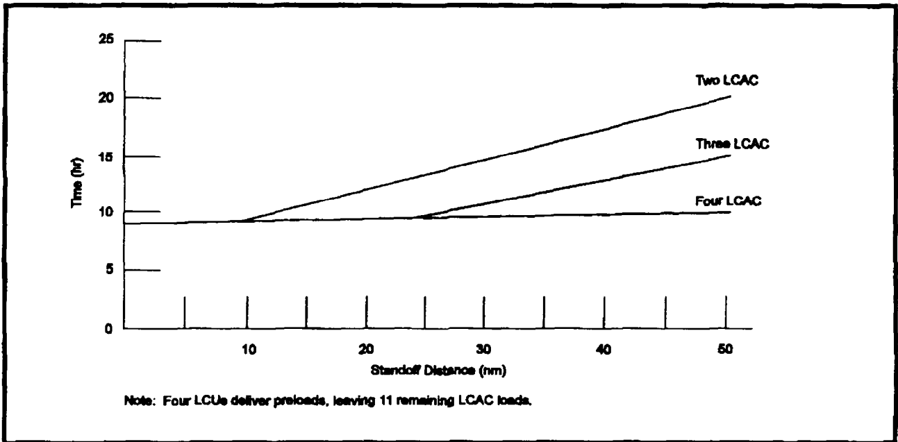
Figure B-7. Estimated Time to Offload an LHA by LCAC (LCU Deliver LCU Preloads)
