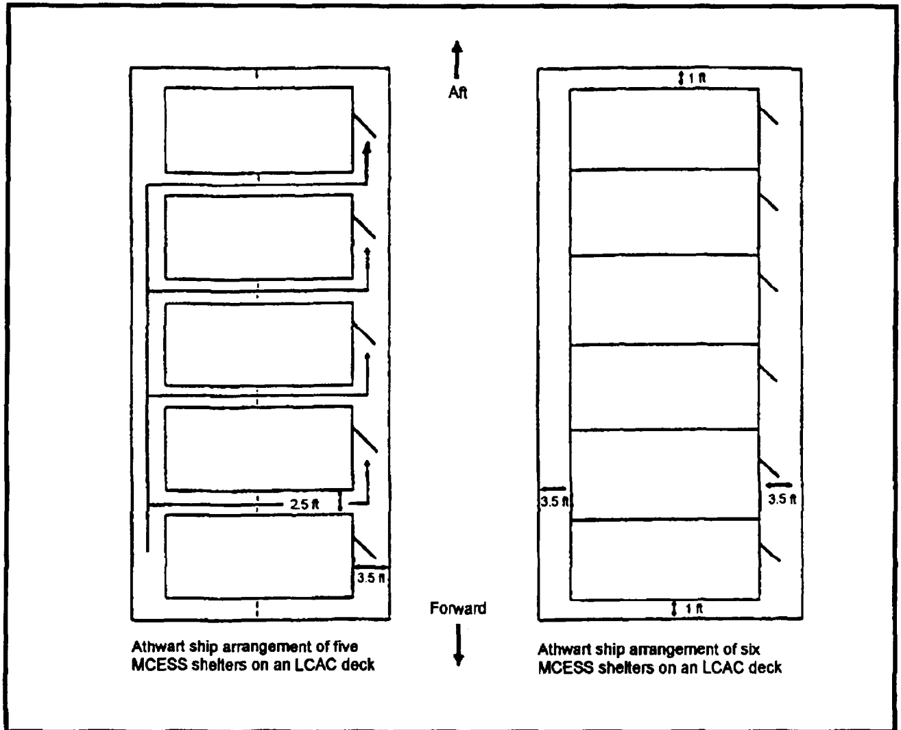
Figure 7-4. MCESS Shelter Configurations (Sheet 2 of 3)
