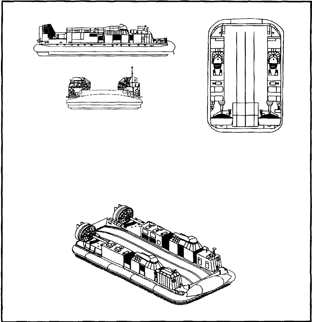
Figure 1-1. LCAC
