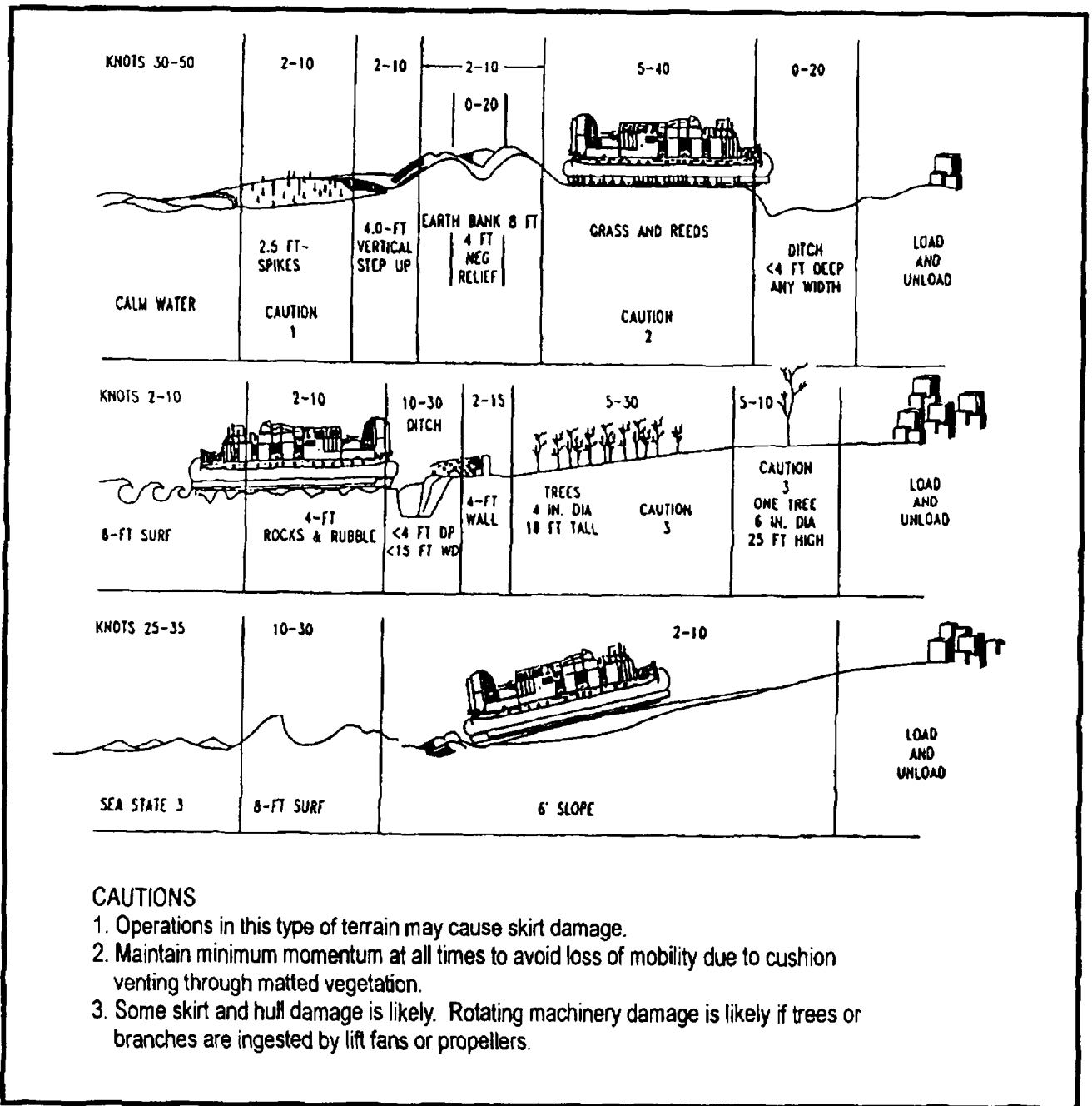
Figure 1-5. Rough Terrain Capabilities
