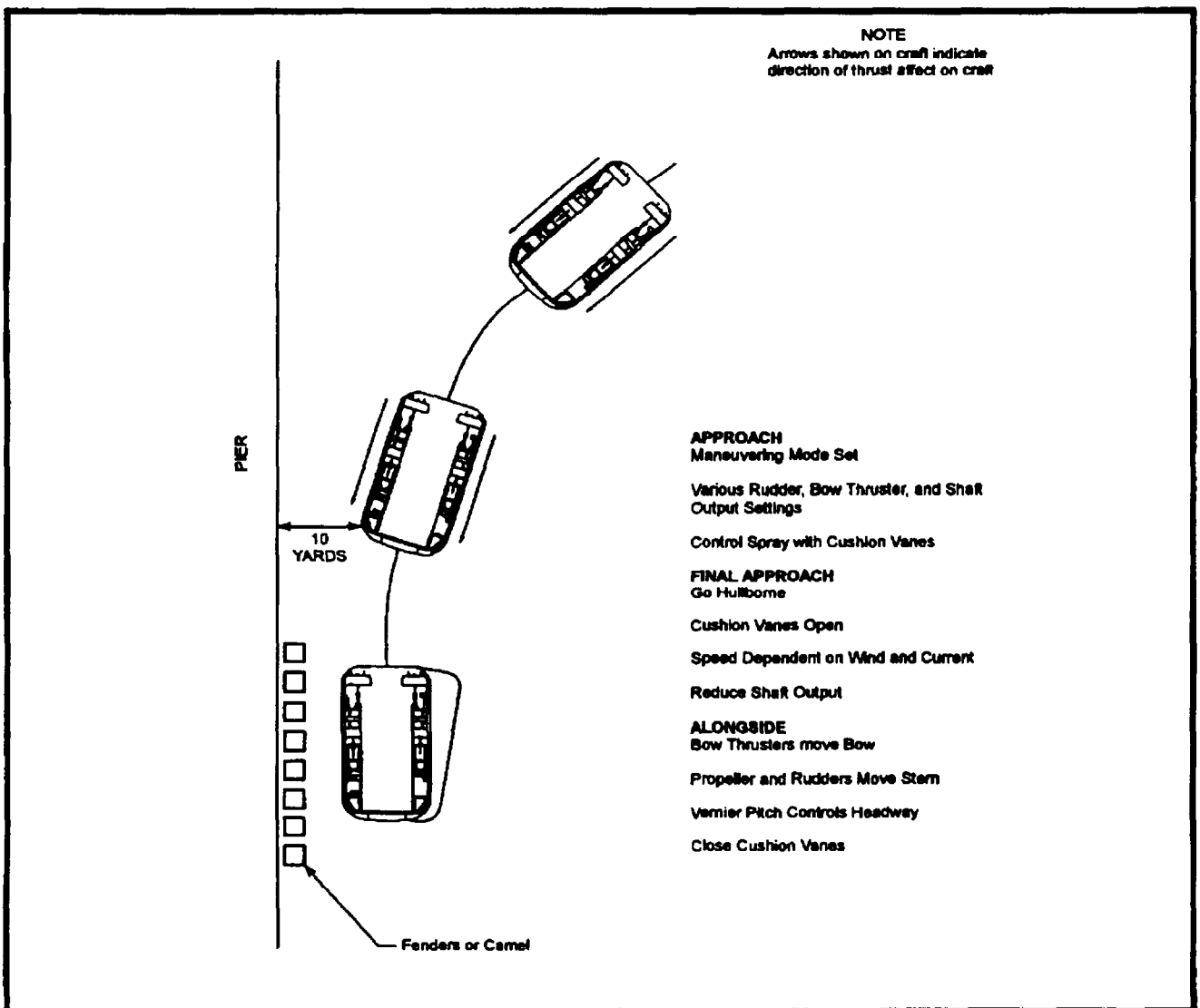
Figure A-9. LCAC Mooring to a Pier
