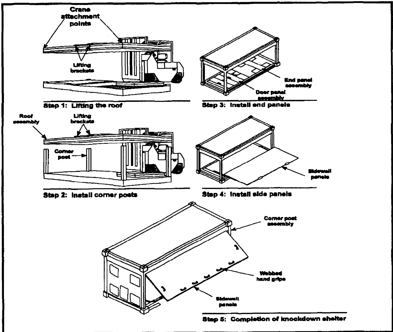
Figure 7-3. MCESS Shelter Assembly Process
