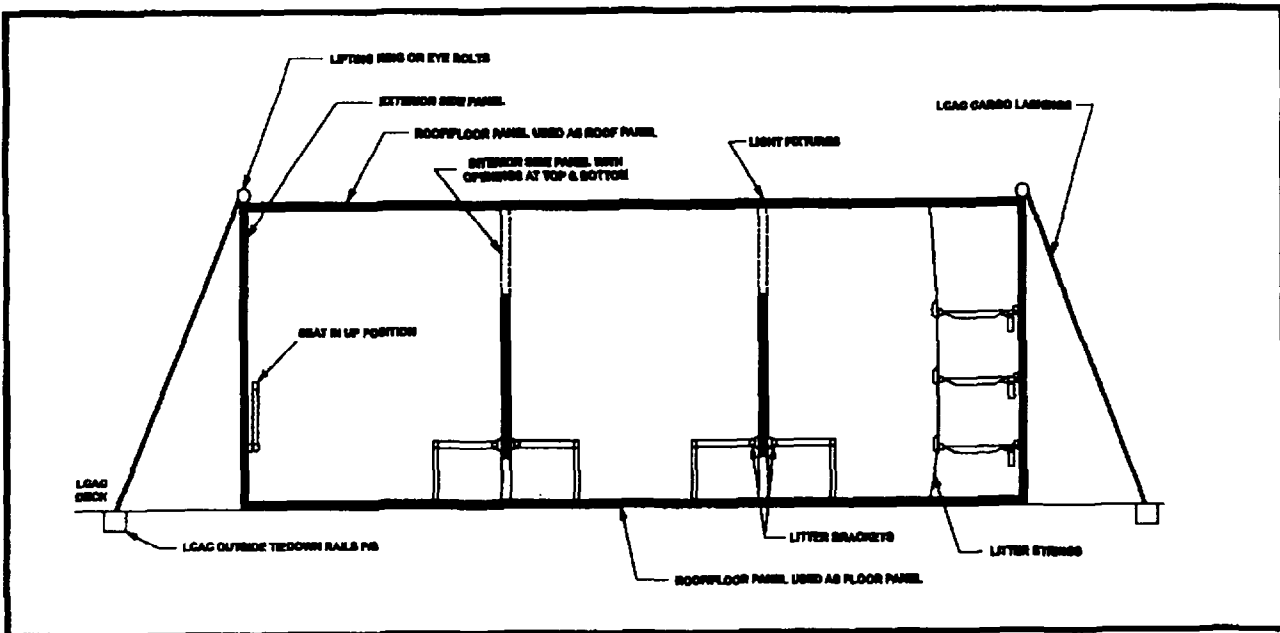
Figure 7-7. LCAC PTM Cross Sectional View
