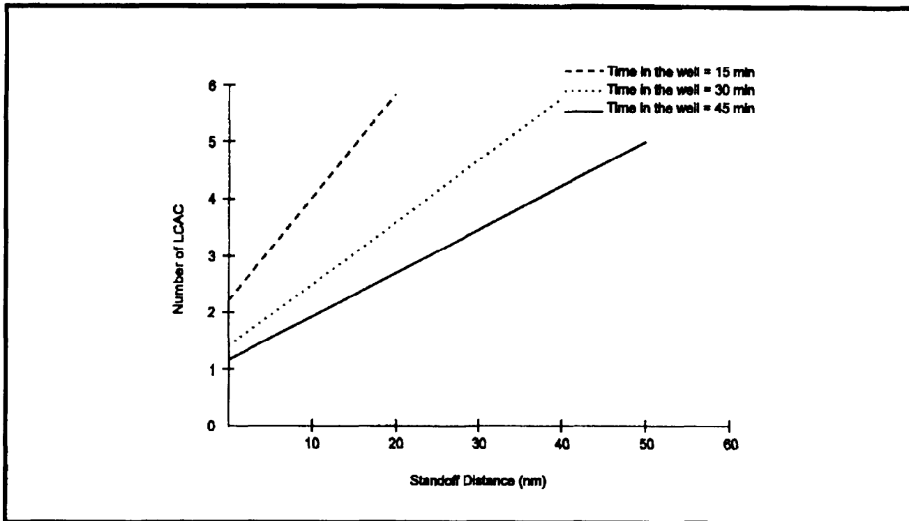
Figure 2-5. Maximum Number of LCAC to Assign to a Ship for Unloading
