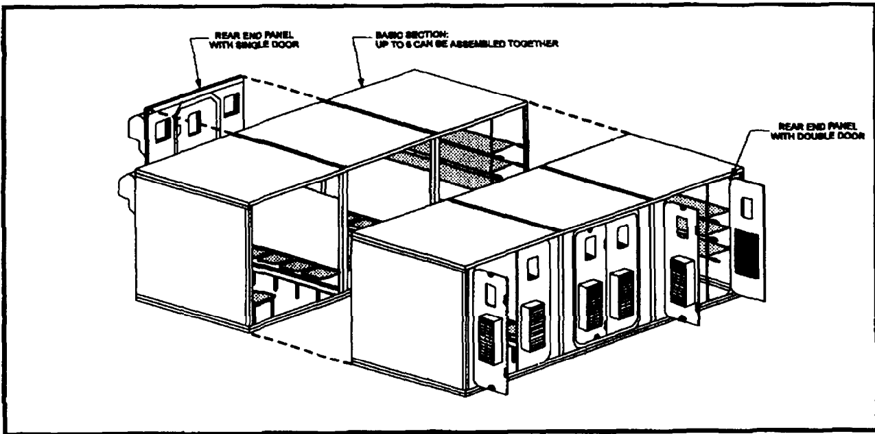
Figure 7-6. PTM-Configured LCAC Assembly
