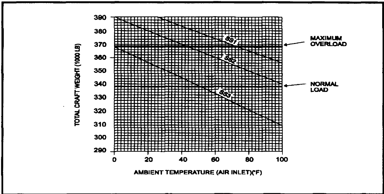
Figure 8-3. LCAC Load as a Function of Ambient Temperature
