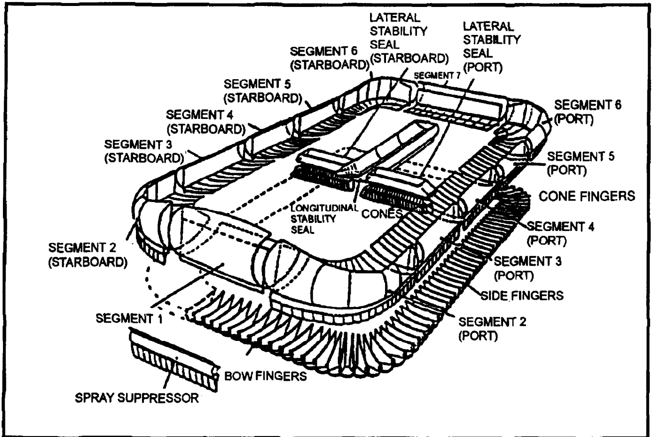
Figure A-2. 3-Dimensional LCAC Skirt Component Drawing
