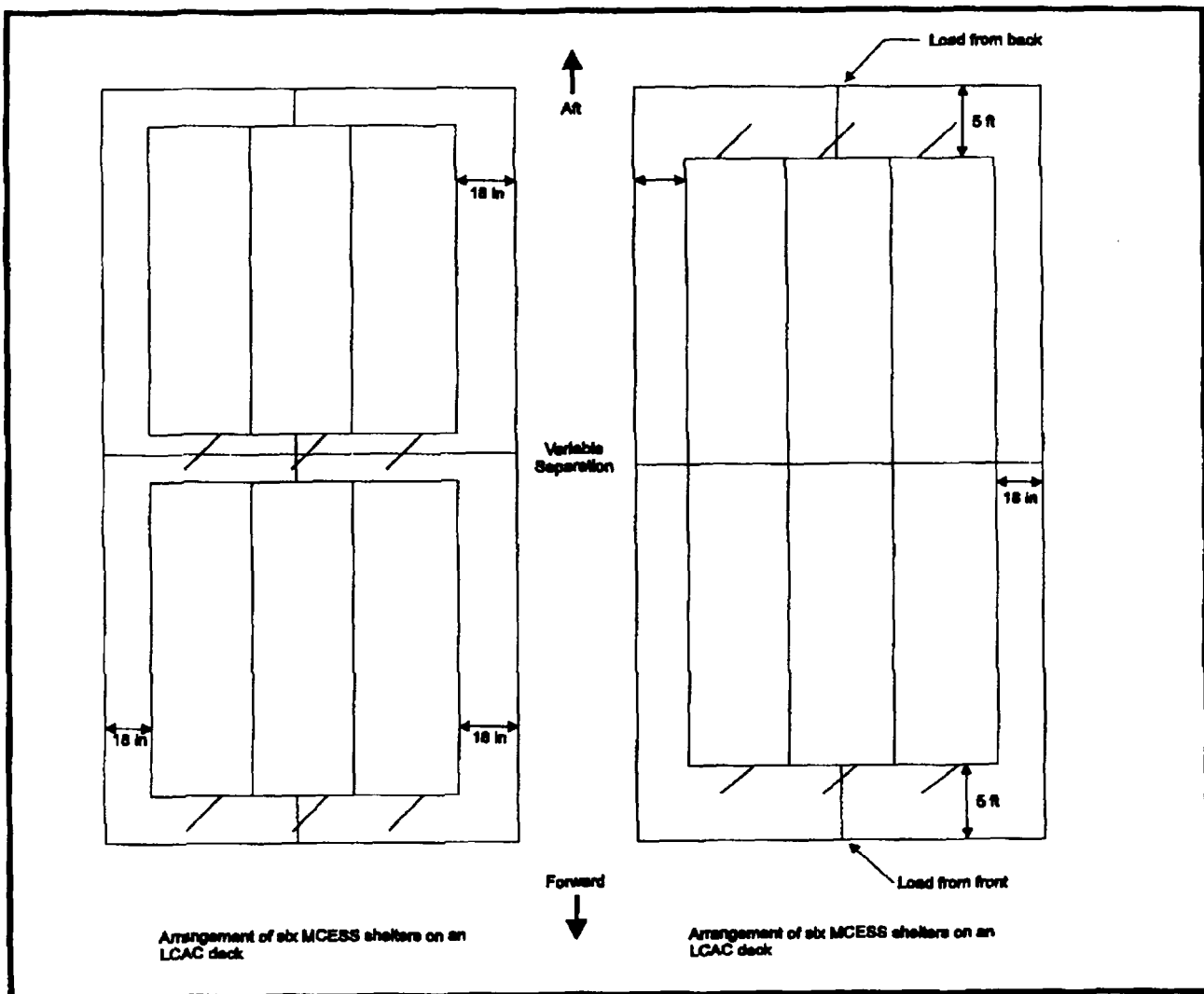
Figure 7-4. MCESS Shelter Configurations (Sheet 3 of 3)
