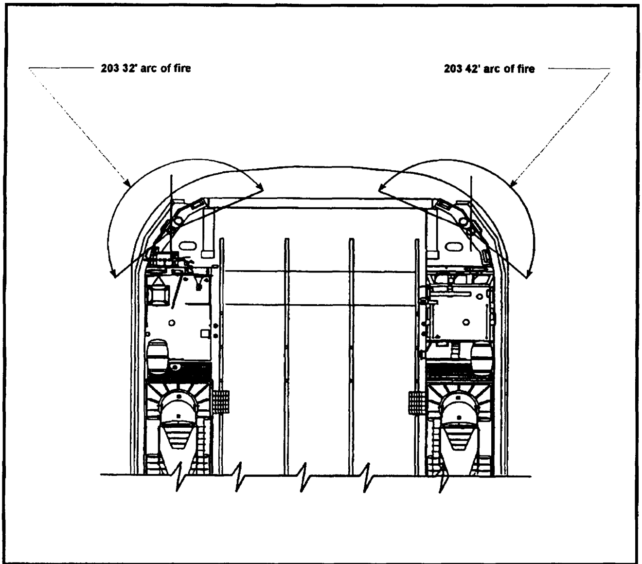
Figure 5-3. LCAC 34 Through 84 Firing Arcs
