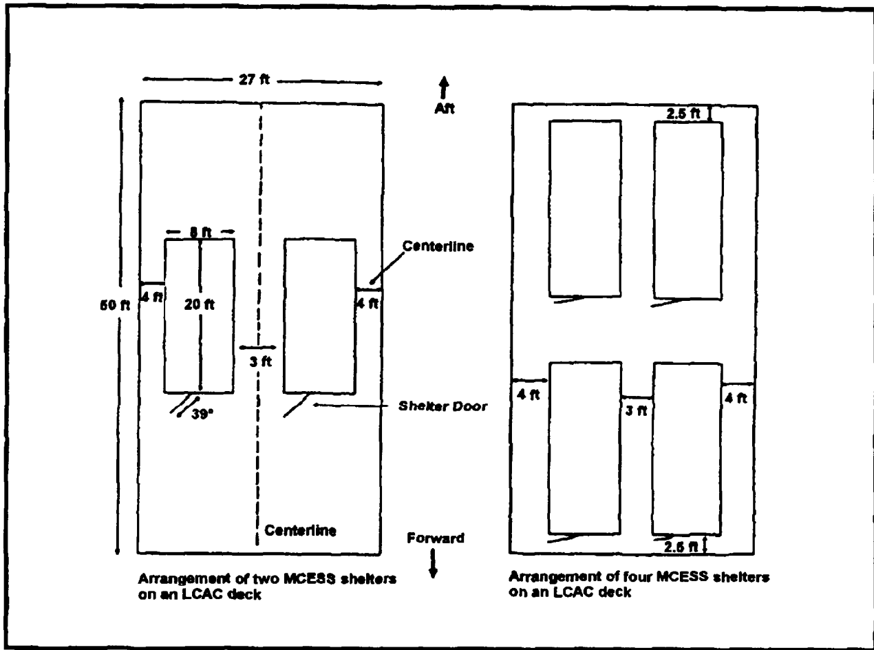
Figure 7-4. MCESS Shelter Configurations (Sheet 1 of 3)
