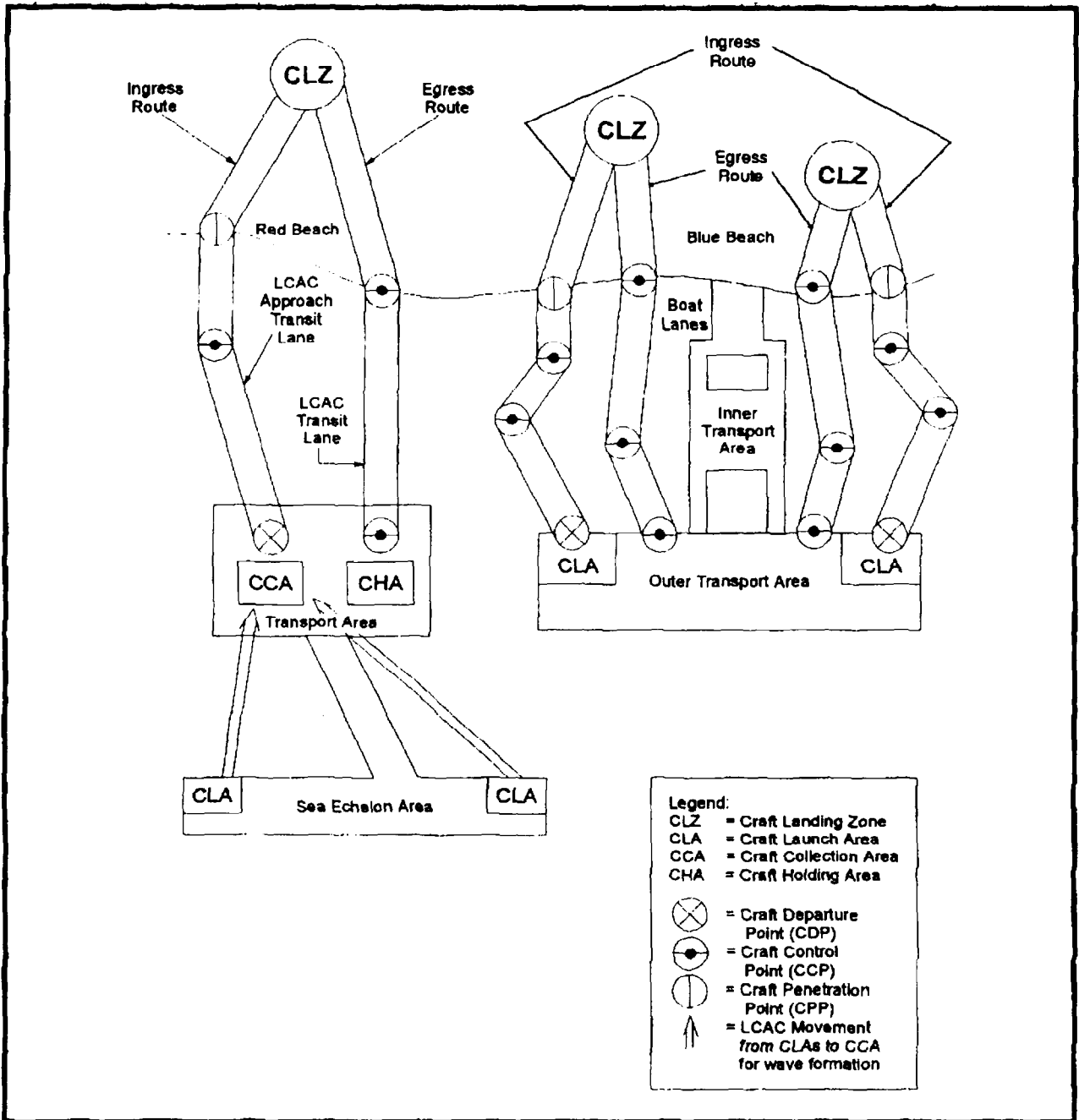
Figure 2-2. LCAC Operating Areas in the Landing Area
