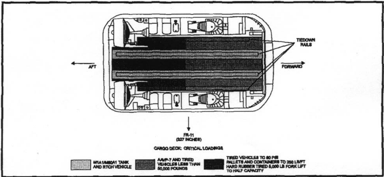
Figure C-1. LCAC Deck Load Diagram
