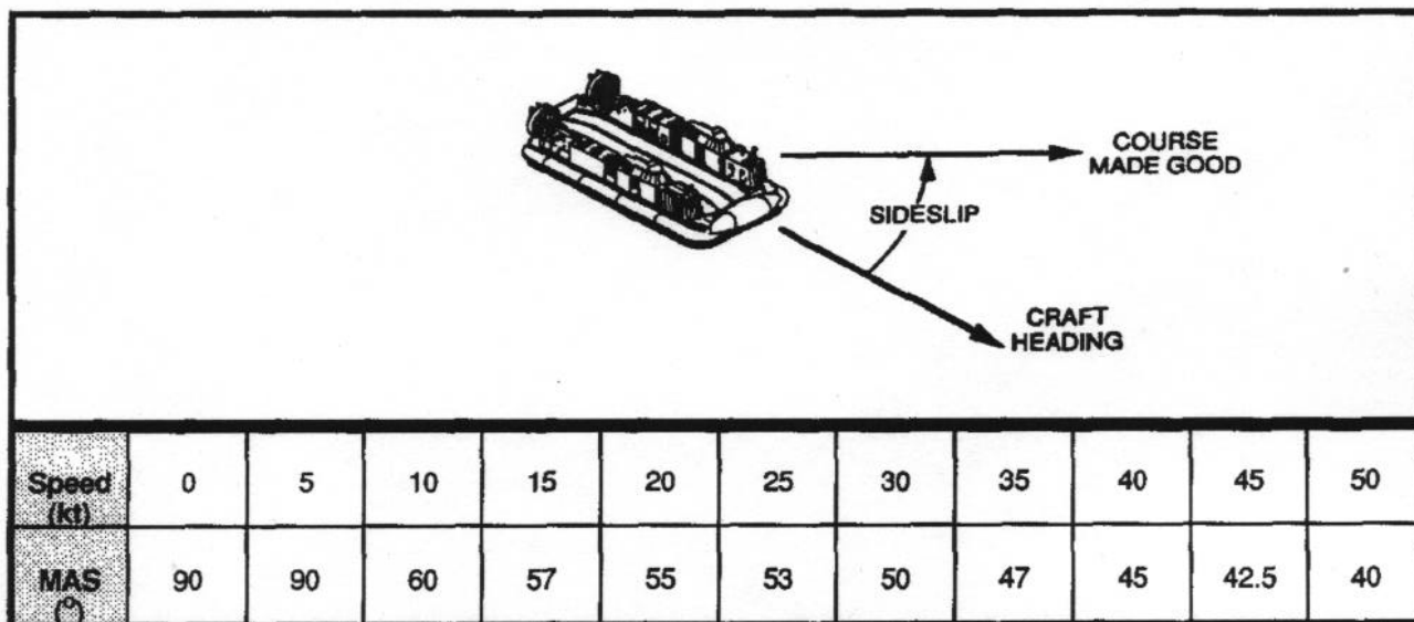
Figure 4-8. Maximum Allowable Slideslip
