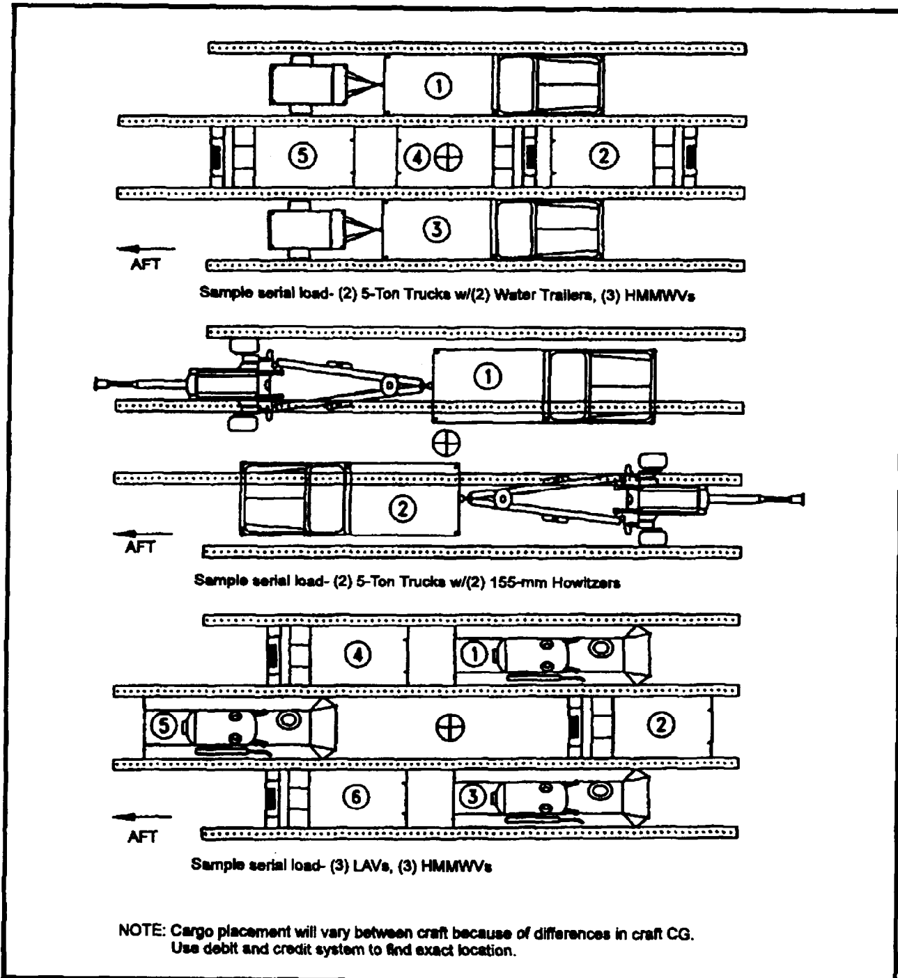
Figure C-7. LCAC Standard Loads and Standard Load Equivalents (Sheet 2 of 4)
