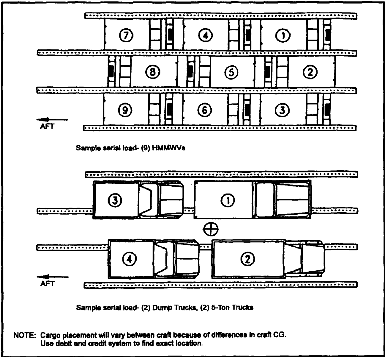
Figure C-7. LCAC Standard Loads and Standard Load Equivalents (Sheet 3 of 4)
