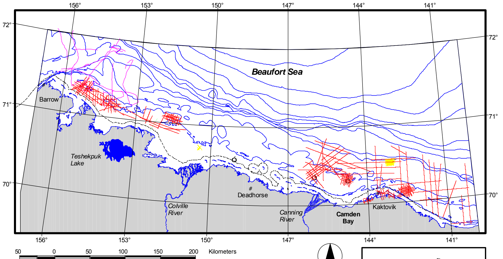
Figure 12a. 1985 - Fall Migration Period, A significant amount of additional activities have uncertain dates and may also have occurred during this period.
