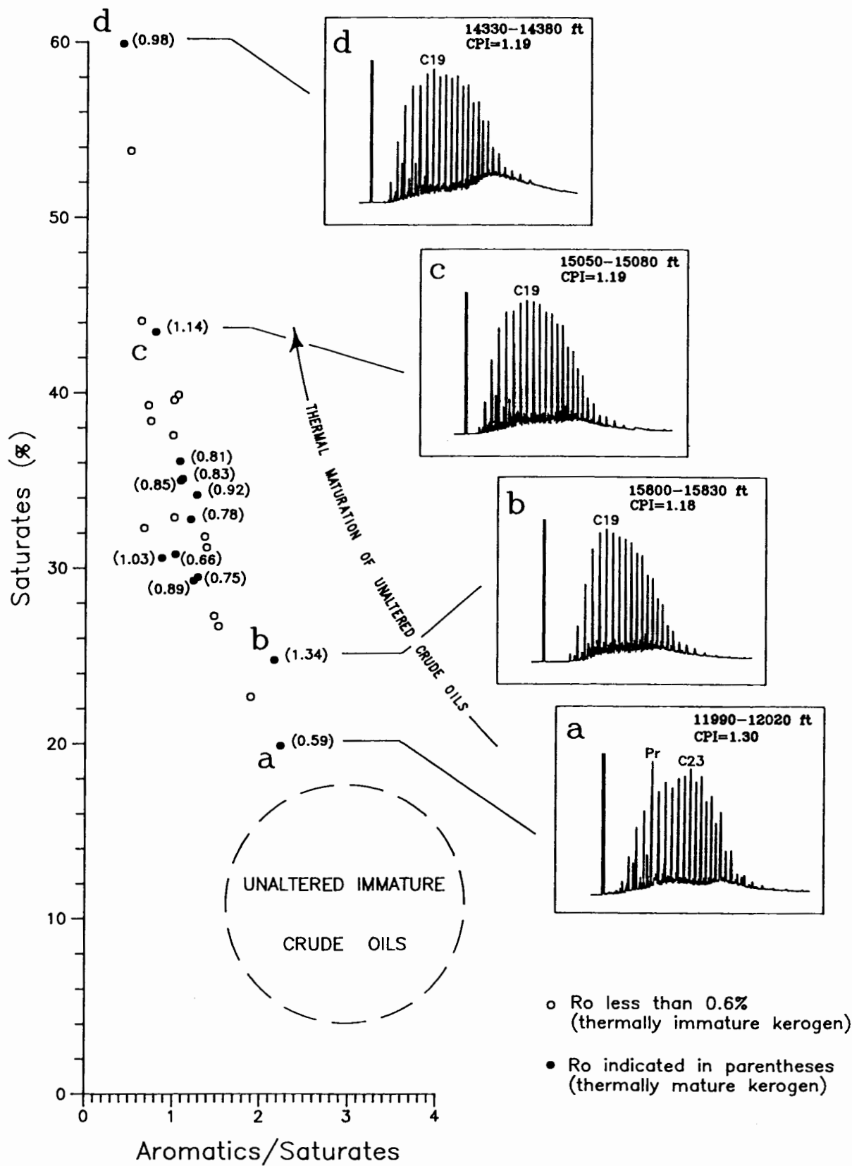
Figure 5.3. Thermal alteration of C_{15+} extractable hydrocarbons from the Canning Formation in the Aurora well. The saturate content of these hydrocarbons is unrelated to depth or to R_o . (Diagram adapted from Connan and others, 1975.)
