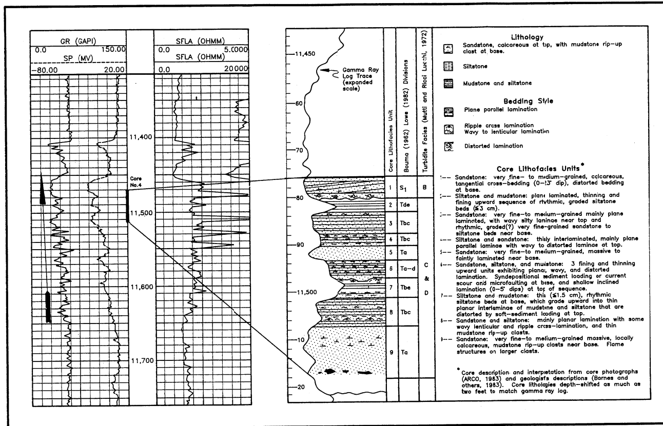
Figure 48. Log and core data from the basal part of the upper Kulthiedh sandstone unit in the OCS Y-0211 No. 1 well that is interpreted to be a depositional lobe of a submarine fan sequence. The large-scale coarsening- and thickening-upward log profile indicates an overall progradational depositional sequence. At the bed-form scale, the conventional core and logs indicate that the sequence was built by fining- and thinning-upward aggradational bedding units. The lower cored beds (core lithofacies units 2-9, 11,481 to 11,521 feet) are interpreted to be low-density turbidite deposits as indicated by evidence of density flow and both traction and suspension deposition: thin graded beds, abundant plane-parallel lamination, abundant mica and carbonaceous detritus, soft sediment deformation, and partial Bouma sequences (fig. 49). The upper bed (core lithofacies unit 1, 11,450 to 11,481 feet), which was cored at the base, is interpreted to be a sandy, high-density turbidite that was probably deposited in a submarine channel near the intersection point of the middle and lower fan (fig. 49). Evidence for this is its stratigraphic position at the top of the lobe sequence, the characteristic channel-like log profile (abrupt base and gradational top), and the large-scale tangential cross-bedding near the base of the bed that indicates traction sedimentation and turbulent flow.
