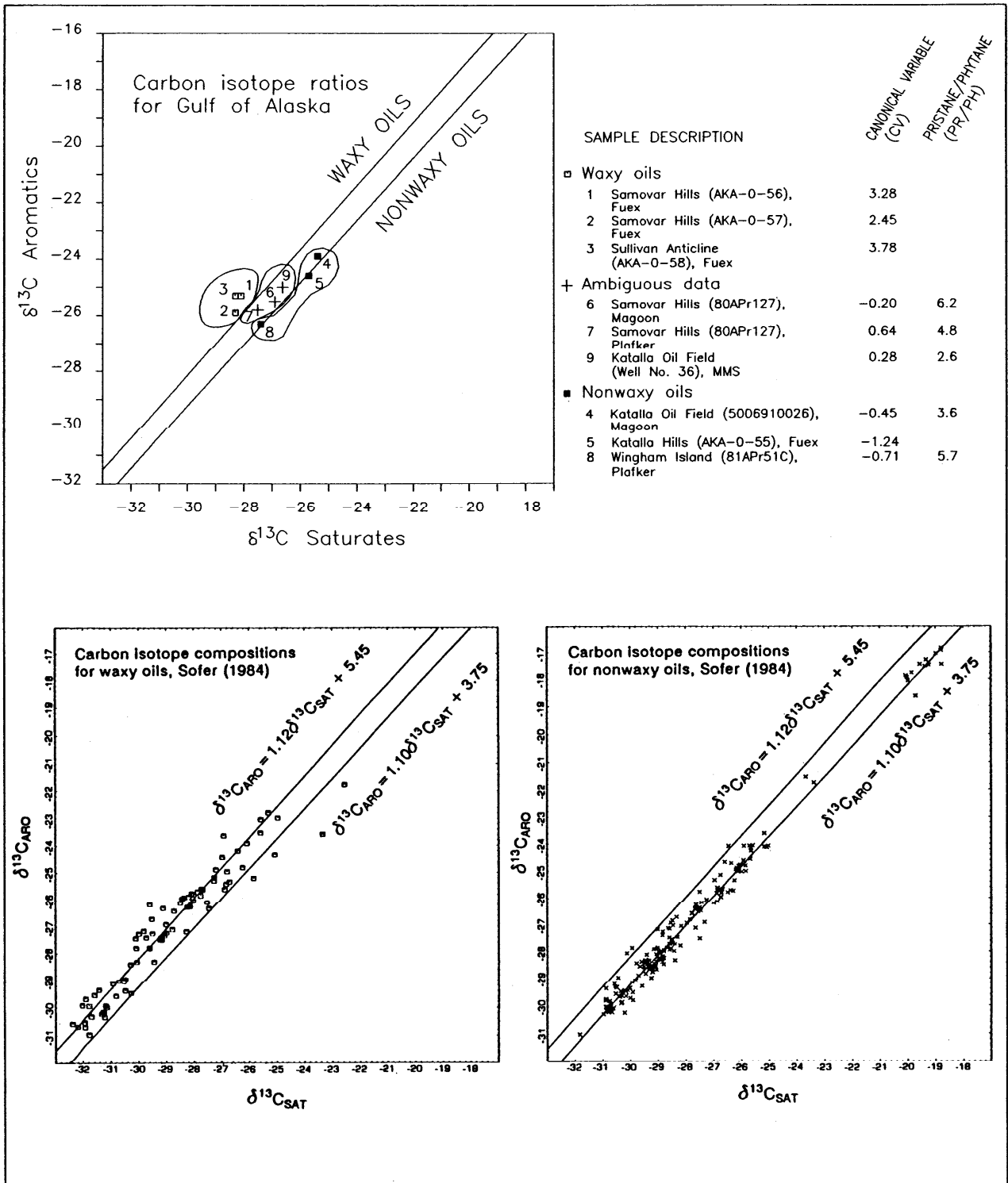
Figure 112. Carbon isotope compositions of C 15 + aromatic versus saturate fractions of Gulf of Alaska crude oil samples with Sofer's (1984) statistical analysis of waxy versus nonwaxy crude oils.
