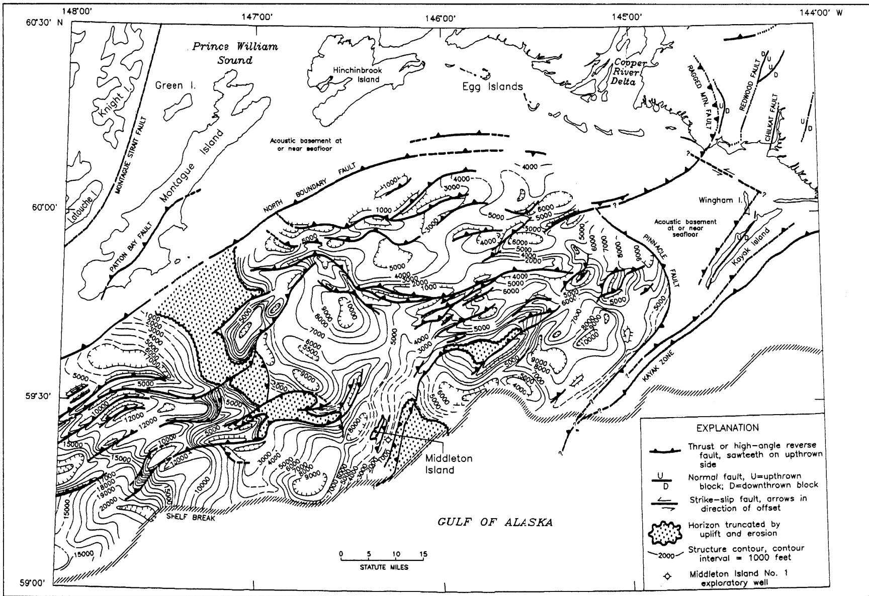
Figure 7. Structure contour map on horizon M6, a regional unconformity that in the vicinity of the Middleton Island No. 1 well represents the base of the late Miocene to Pleistocene glaciomarine Yakataga Formation. Strata immediately underlying horizon M6 consist of siltstone and shale that are tentatively correlated to the Sitkinak Formation on the Kodiak shelf. Onshore geology adapted from Plafker (1967, 1974) and Winkler and Plafker (1981).
