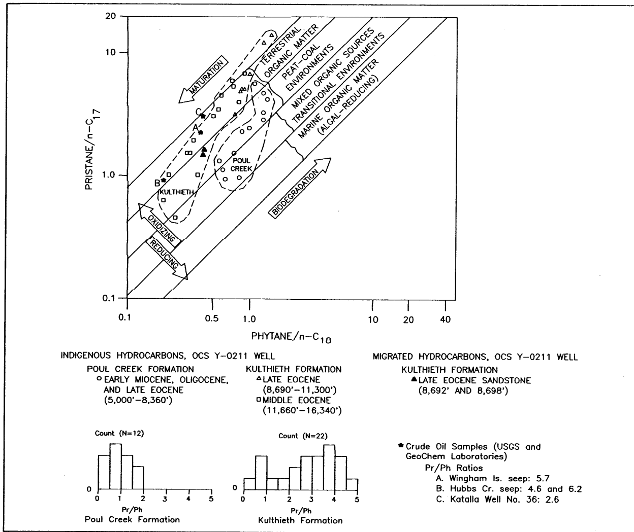
Figure 110. Plot of pristane/ n-C_{17} versus phytane/ n-C_{18} for Poul Creek and Kulthieth samples from the ARCO OCS Y-0211 No. 1 well. Two USGS oil seep samples and a crude oil sample from the Katalla No. 36 well provided by Phillips Petroleum are also shown. This diagram is adapted from a plot constructed by W. L. Orr in Shanmugam (1985) and is based on concepts proposed by Lijmbach (1975).
