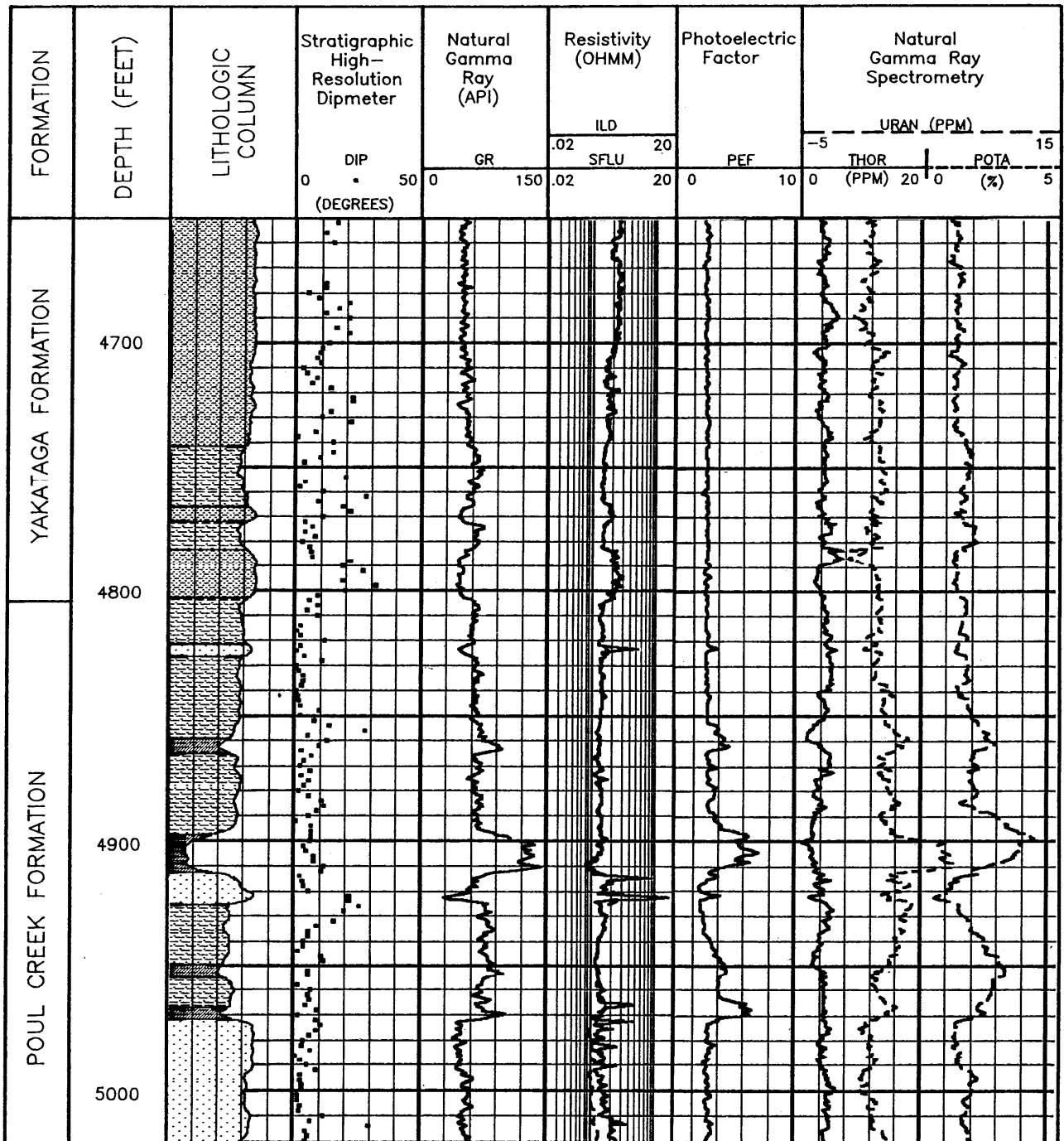
Figure 41. Lithologic interpretation of OCS Y-0211 No. 1 well logs at the Yakataga-Poul Creek formational contact. The base of the Yakataga Formation at 4,805 feet is marked by a change from widely scattered dip magnitudes in the poorly stratified glaciomarine sediment to more consistent dips in the Poul Creek marine sediments. In the Poul Creek section, four glauconitic beds are apparent between 4,850 and 5,000 feet. Glauconitic beds are indicated by zones of higher radioactivity on the gamma ray (GR), uranium (URAN), and potassium (POTA) log traces, and higher values on the photoelectric factor (PEF) log trace. The glauconitic zones represent condensed sections formed when clastic deposition was very slow and sedimentation was dominated by slowly accumulating authigenic glauconite.
