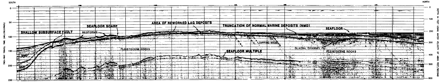
Figure 123. A high-resolution seismic-reflection profile across a portion of the Icy Bay structure southeast of Cape Yakataga showing sedimentary units in the upper Yakataga Formation, truncation of Holocene sediments, and an area of lag deposits. The upper sedimentary units are defined as Holocene normal marine deposits (NMD), Pleistocene glacial marine deposits (GMD), and older Pleistocene rocks. (Shot by BBN Geomarine Services, 1975.)
