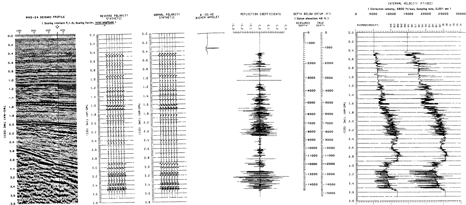
FIGURE 7. Synthetic Seismogram of ARCO's Norton Sound COST No. 2 Well.
