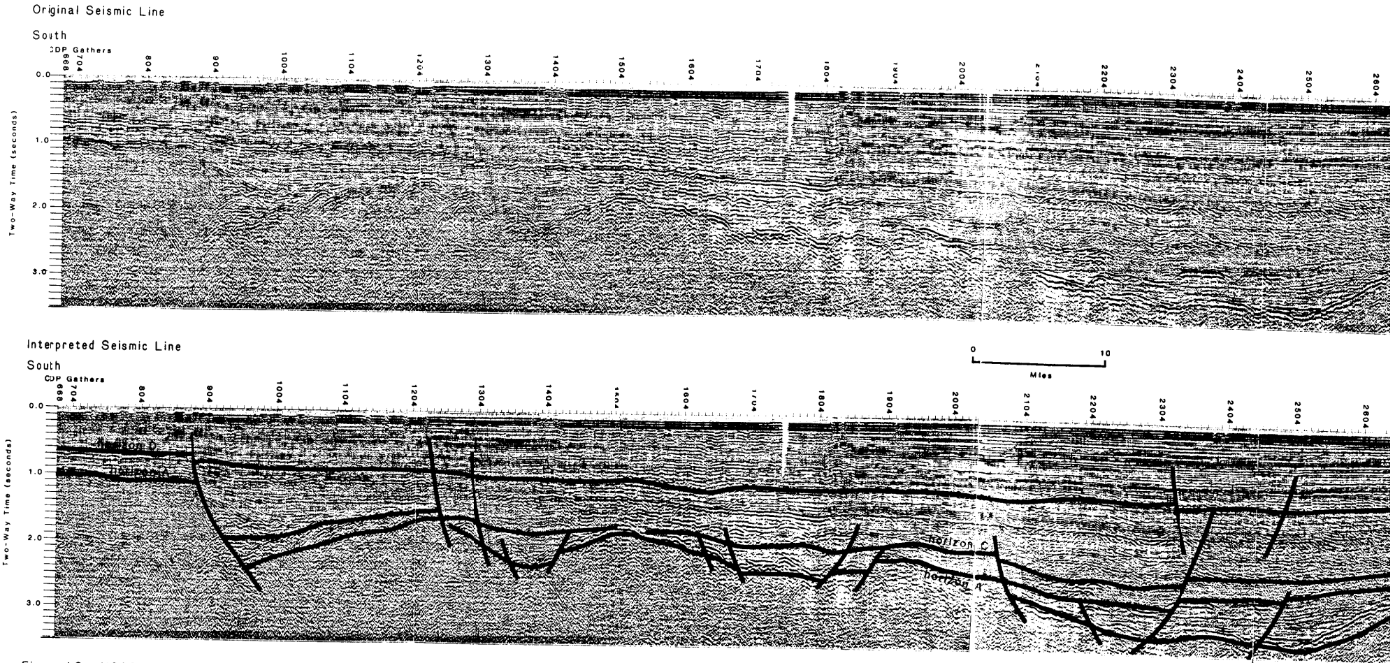
Figure 10. USGS Seismic Line 802.
