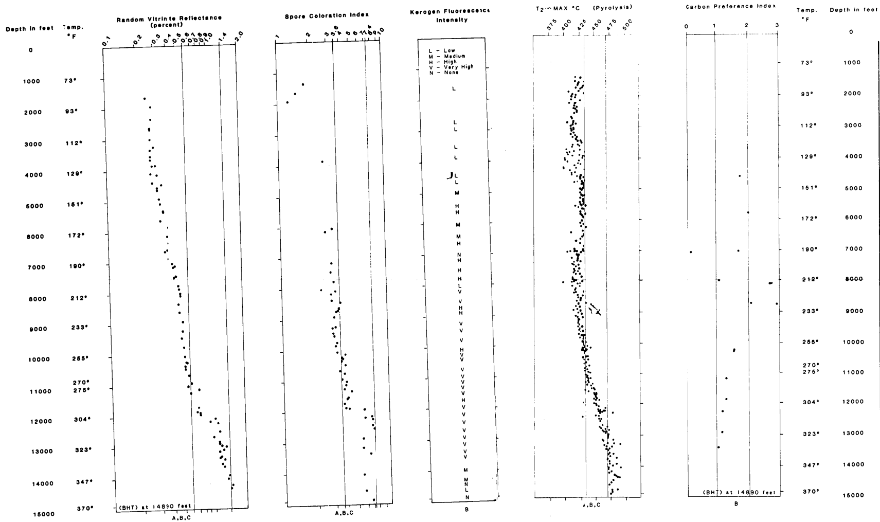
Figure 40. Selected indicators of Thermal Maturation. [Sample Sources: A-Guttinas, B-Sidewall Cores, C-Conventional Cores]
