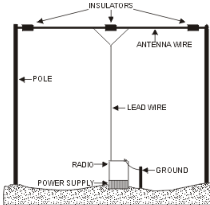
Figure 4-3. Doublet Antenna.
