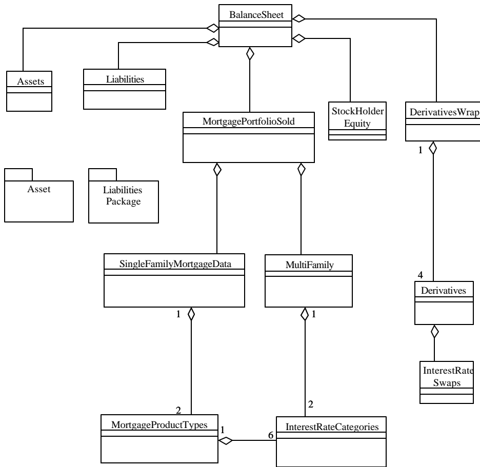
Figure 3-7: Balance Sheet Class Diagram
