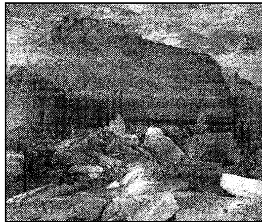
Figure 4. - If the roof is not reinforced properly with rock bolts, the beams can progressively fail higher into the roof until a stable roof beam is encountered. Here the roof fall has assumed an elliptical shape.
