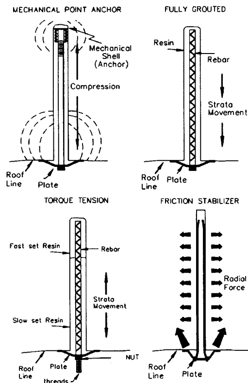
Figure 7. - Four common roof support systems: mechanical point-anchor, fully grouted resin, torque tension resin, and friction stabilizer bolts.
