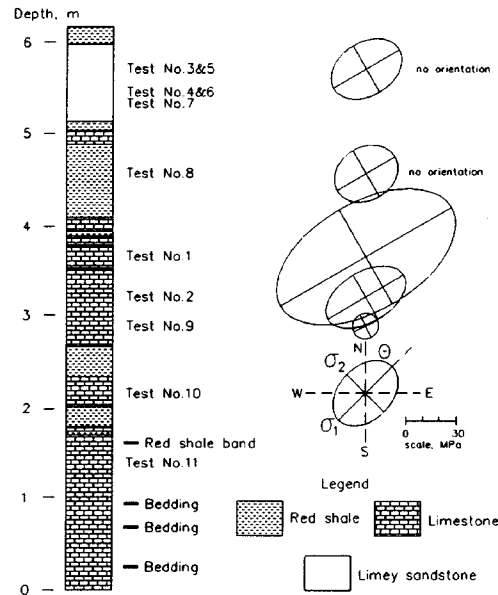
Figure 9. - Stress ellipses from six successful hydraulic fracturing tests within the roof of a Loyalhanna Limestone Mine.
