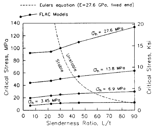
Figure 6 - Potential stability to buckling failure of differently shaped roof beams with a varying horizontal stress field, ranging from 3.45 to 27.6 MPa.
