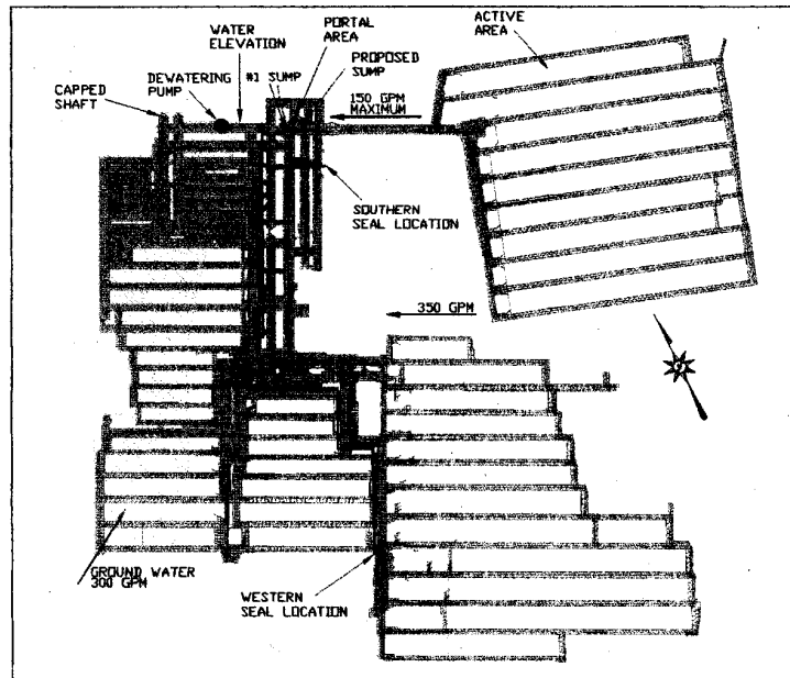
Figure 1 Mine Map With Flow Diagram
