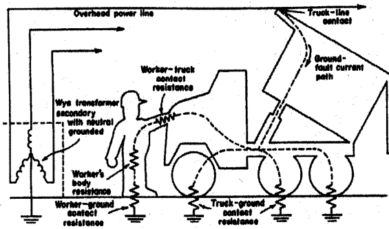
Fig. 1. Schematic of a power line contact.
