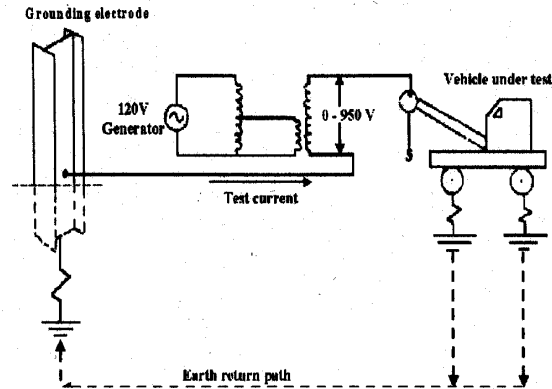
Fig. 2. Schematic representation of the tests done at LLL.
