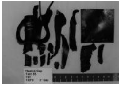
HGT-65. TNT, 3-inch gap, 100°C.
