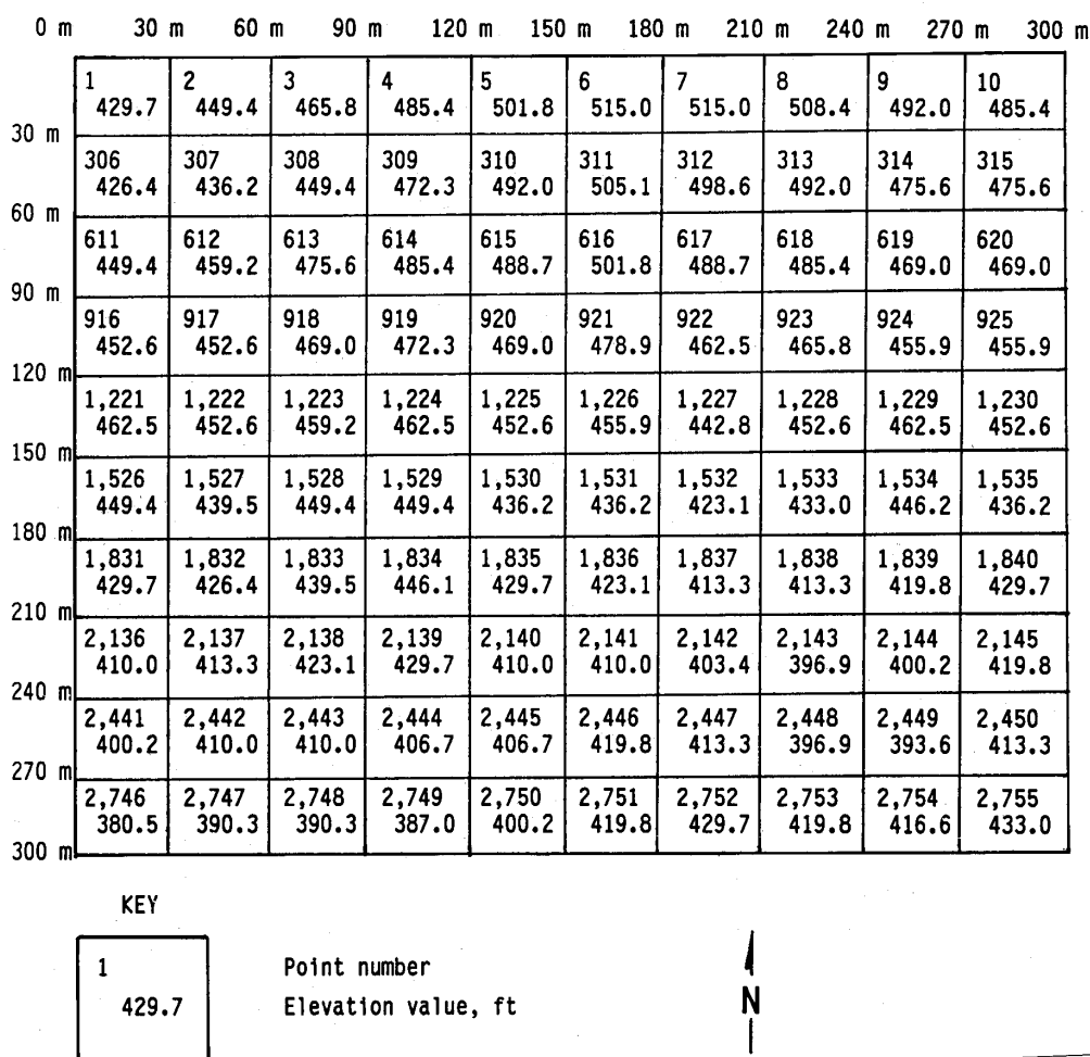
Figure 7.—Format of input file containing topographic elevations.
