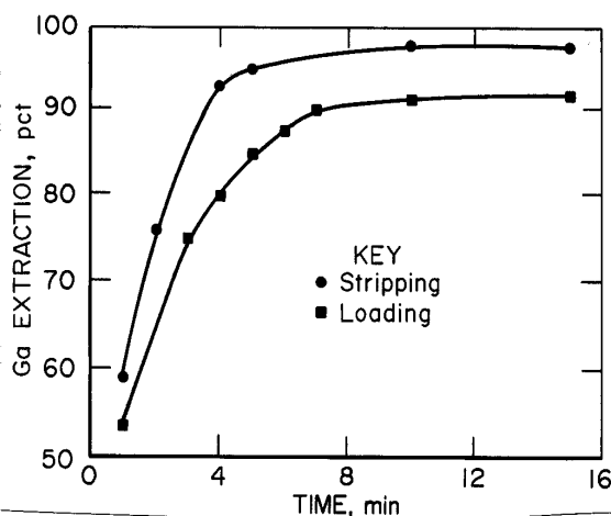
Figure 21.—Gallium equilibrium loading and stripping on 0.3M OPAP.
