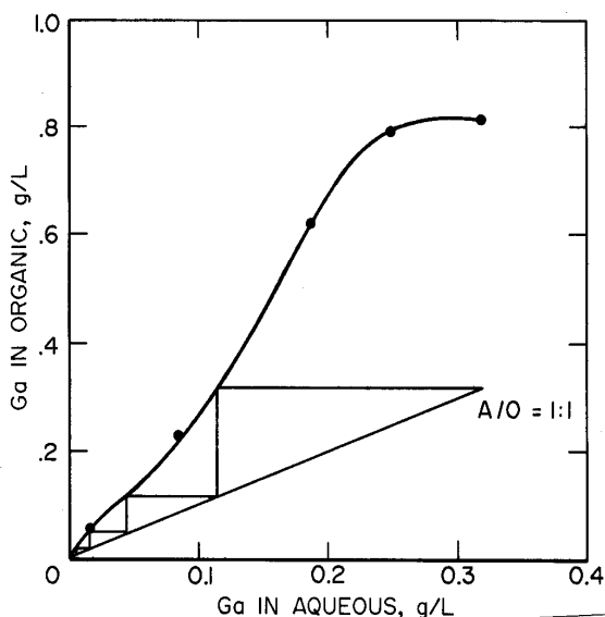
Figure 22.—McCabe-Thiele analysis loading 0.32-g/L-Ga aqueous on 0.3M OPAP. (A/O = aqueous-to-organic ratio)
