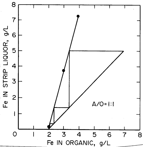
Figure 29.—McCabe-Thiele analysis stripping Iron with 3M H 2 SO 4 . (A/O = aqueous-to-organic ratio)
