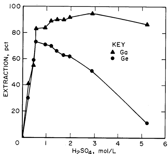
Figure 7.—Effect of H_2SO_4 molarity on gallium and germanium extraction from zinc residue (4 h, 80° C).
