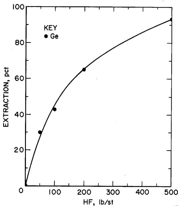
Figure 13.—Effect of HF concentration on germanium extraction from H_2SO_4 -leached residue (2 h, 80° C, 10 pct solids).
