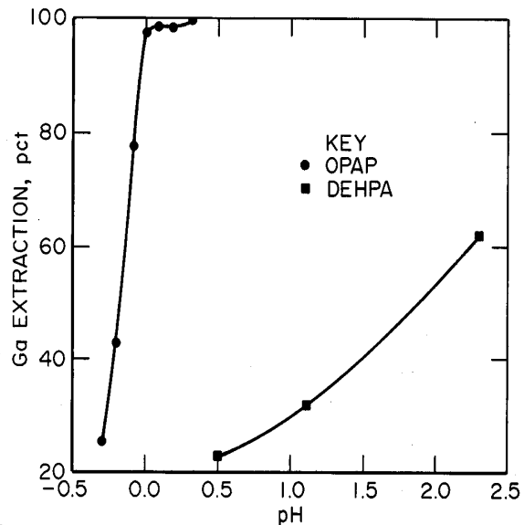
Figure 20.—Effect of pH on gallium extraction using the solvents OPAP and DEHPA.
