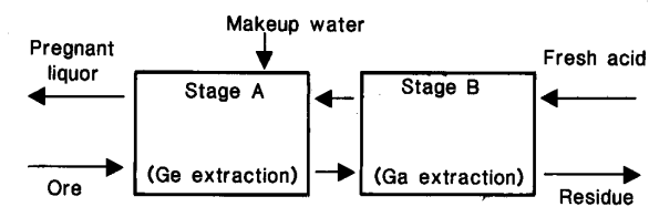
Figure 17.—Proposed two-stage leach system.
