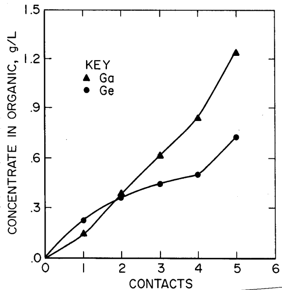
Figure 30.—Effect of multiple contacts in the coextraction of germanium and gallium from zinc processing liquors.
