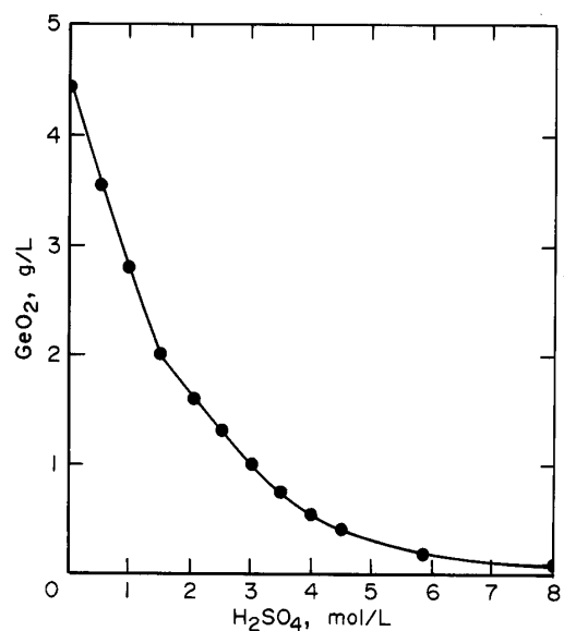
Figure 8.—Solubility of GeO_2 in H_2SO_4 .
