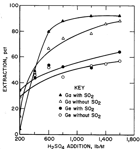
Figure 6.—Effect of adding SO_2 to H_2SO_4 leach on gallium and germanium extraction from zinc residue (4 h, 80° C, 20 pct solids).
