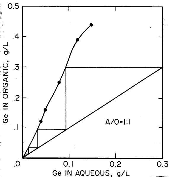
Figure 26.—McCabe-Thiele analysis of germanium-loading isotherm, 40-g/L-H 2 SO 4 solution. (A/O = aqueous-to-organic ratio)
