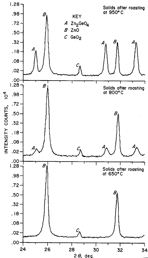
Figure 9.—XRD printouts of ZnO-GeO 2 mixtures at 650°, 800°, and 950° C.
