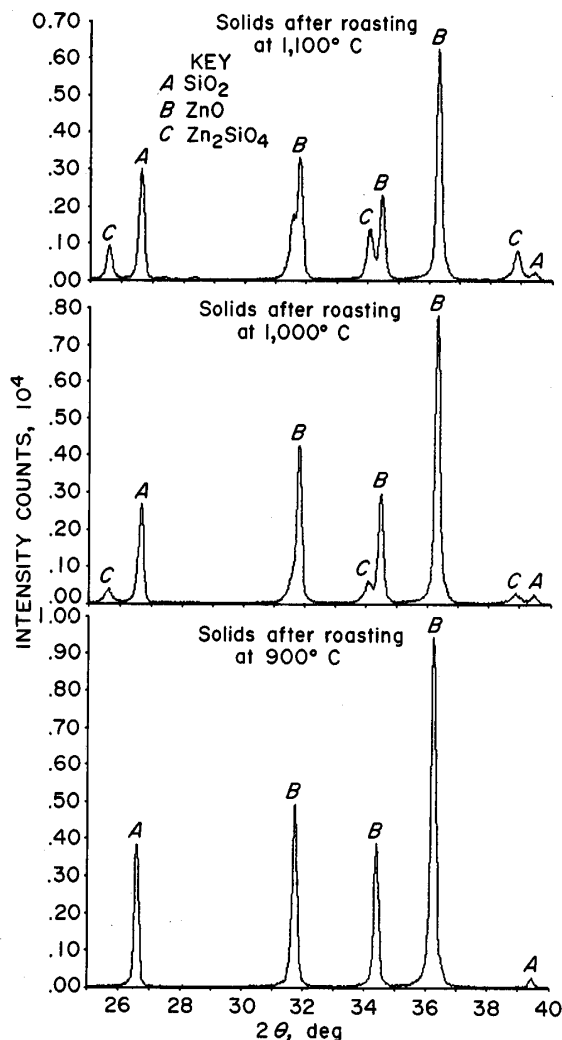
Figure 10.—XRD printouts of ZnO-SiO 2 mixtures at 900°, 1,000°, and 1,100° C.
