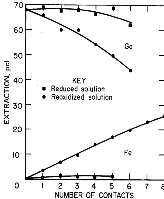
Figure 19.—Gallium and iron extraction from reduced and reoxidized solutions.
