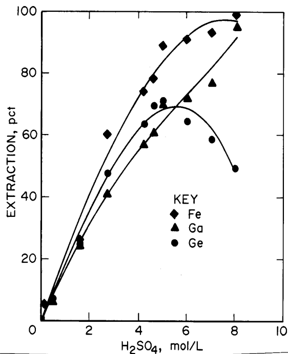
Figure 14.—Effect of H_2SO_4 concentration on metal extraction from gallium-germanium ore (2 h, 80° C, 20 pct solids).
