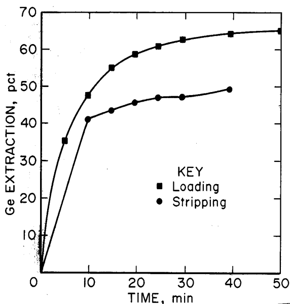
Figure 25.—Germanium equilibrium loading and stripping on 0.2M OPAP-30 pct LIX 63.
