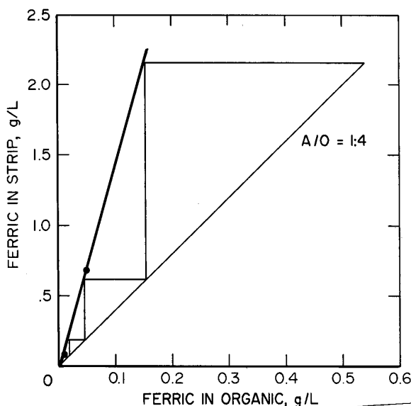
Figure 24.—McCabe-Thiele analysis stripping ferric iron with 50 pct H_3PO_4 . (Additional data point x = 0.68 , y = 7.09 ; A/O = aqueous-to-organic ratio)
