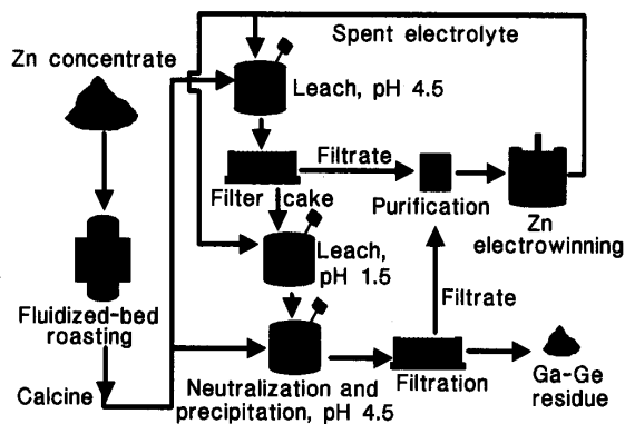
Figure 1.—Stages of zinc processing.
