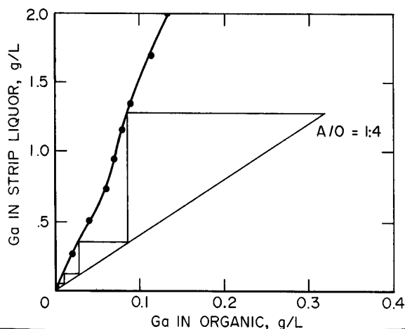
Figure 23.—McCabe-Thiele analysis stripping 0.32-g/L-Ga loaded organic using 1.5M H_2SO_4 . (A/O = aqueous-to-organic ratio)
