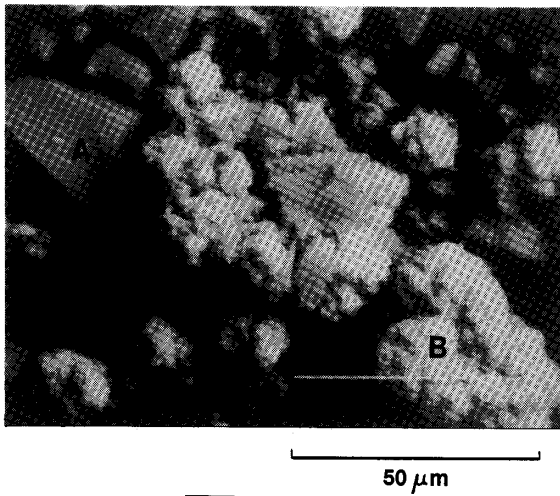
Figure 12.—SEM photograph of SiO_2-GeO_2 solid solution. (A = SiO_2 , B = GeO_2 , scale = 50 \mu m )
