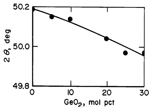
Figure 11.—Shift of 2θ quartz angle with increasing amounts of GeO 2 .
