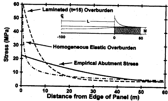
Figure 3. Comparison of the longwall abutment stress computed from the homogeneous elastic model, the laminated model and the empirical formula.
