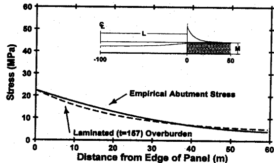
Figure 4. Plot of the laminated abutment stress fitted to the empirical formula.
