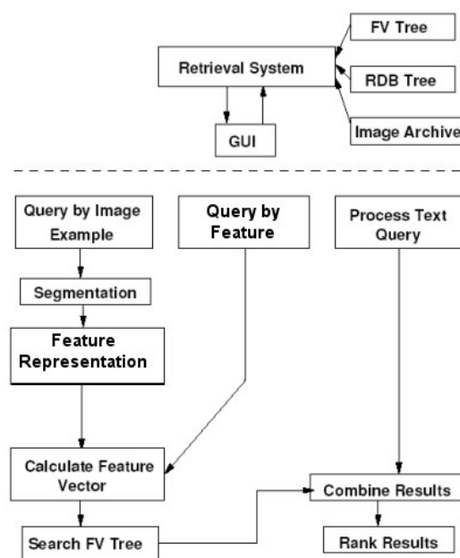
Figure 5 - CBIR Retrieval Trail
