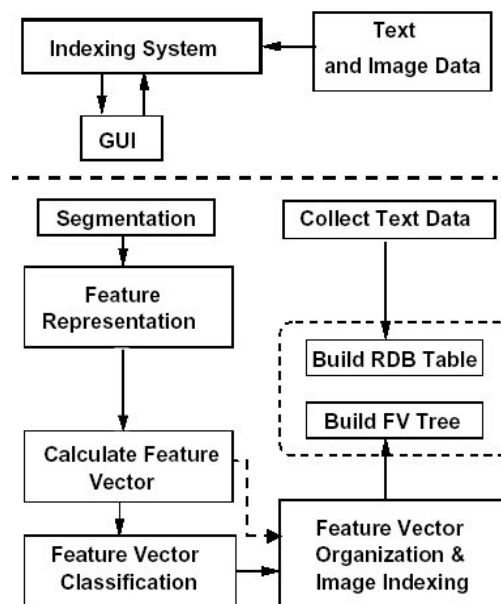
Figure 2 - CBIR Indexing Trail
