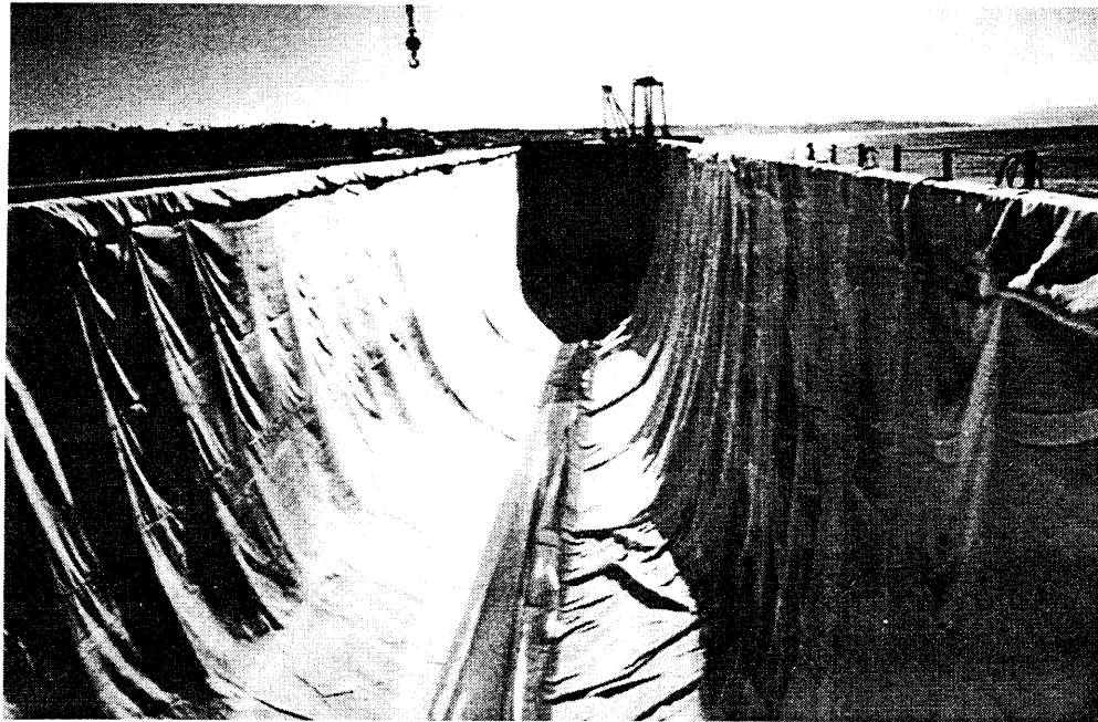
Figure 7. Geotextile liner inside a split-hull scow used in the Marina del Ray contaminated material containerization project
