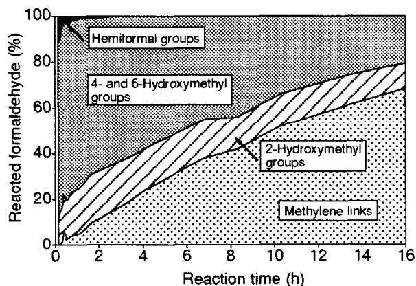
Figure 7 Summary plot of changes in the distribution of formaldehyde-derived species in HMR with time (acquisition of data started several minutes after the reaction began).
