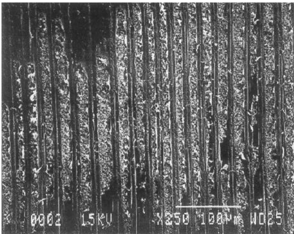
Fig. 9. SEM of leached HQA-treated latewood at 10% HQA/5 % crosslinker loading (250 ×).
