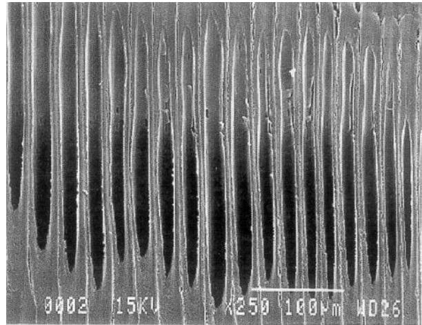
Fig. 6. SEM of leached latewood control (150 ×).
