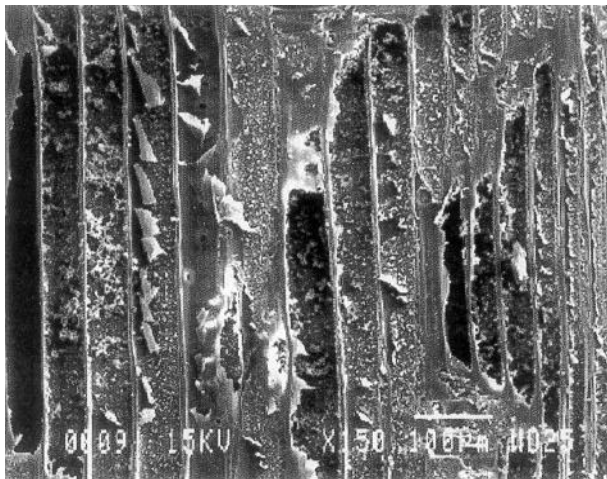
Fig. 11. SEM of leached DBHQA-treated earlywood at 5 % DBHQA/5 % crosslinker (150 ×).
