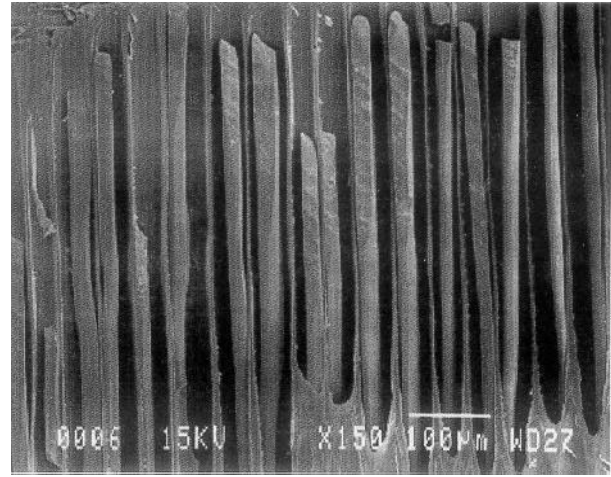
Fig. 8. SEM of leached TBTA-treated earlywood at 20% TBTA/5 % crosslinker loading (150 ×).
