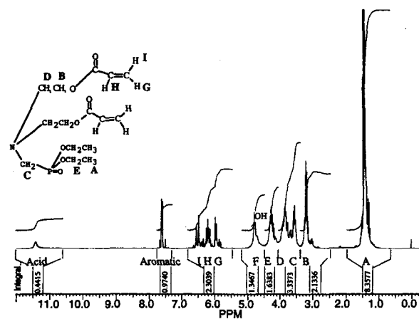
Fig. 2. 1 H NMR spectrum of Fyrol 6 acrylate.
