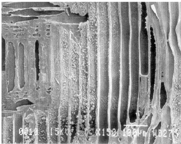
Fig. 7. SEM of leached PCAP-treated earlywood at 20% PCPA/5 % crosslinker loading (150 ×).
