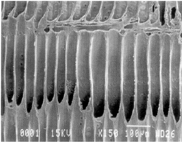
Fig. 5. SEM of leached earlywood control (150 ×).
