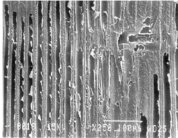
Fig. 10. SEM of leached F6A-treated latewood at 10% F6A/5 % crosslinker loading (250 ×).
