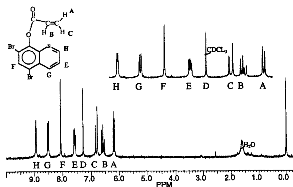
Fig. 3. ^1\text{H} NMR spectrum of 5,7-dibromo-8-hydroxyquinolyl acrylate.
