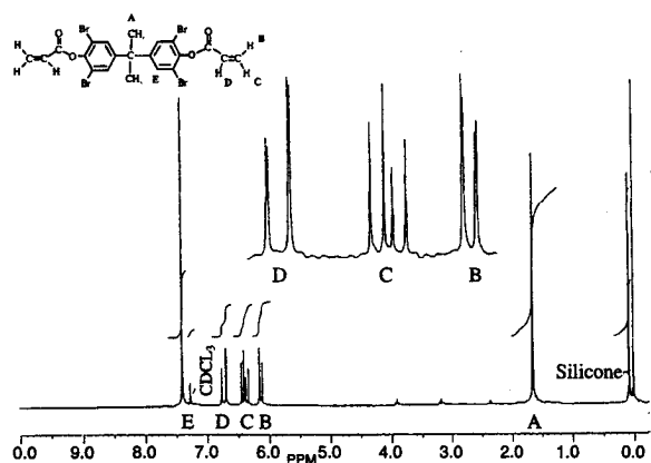
Fig. 4. ^1\text{H} NMR spectrum of tetrabromobisphenol A acrylate.
