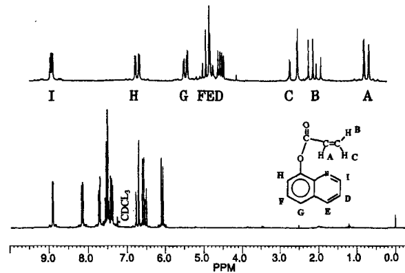
Fig. 1. 1 H NMR spectrum of 8-hydroxyquinolyl acrylate.
