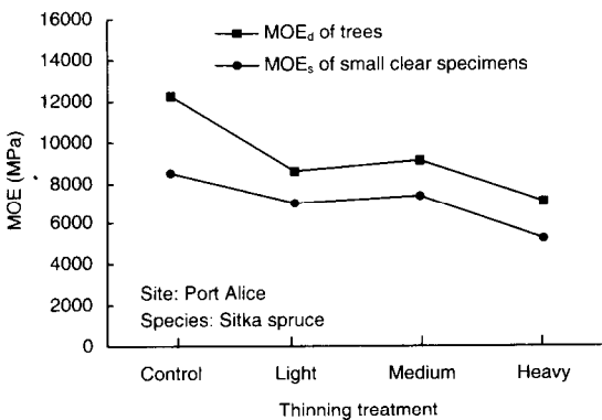
FIG. 10. Modulus of elasticity (MOE) of Sitka spruce as a function of thinning treatment (control, light, medium, heavy).
