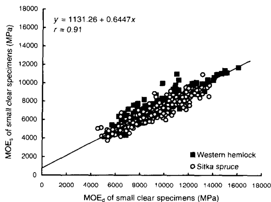
FIG. 5. Relationship of MOE_d to MOE_s for small, clear specimens.
