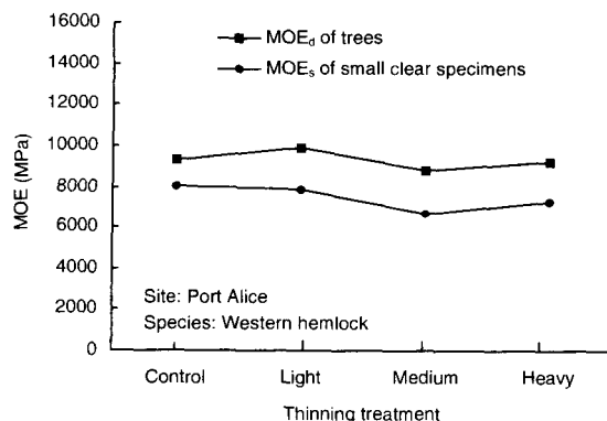
FIG. 11. Modulus of elasticity (MOE) of western hemlock as a function of thinning treatment (control, light, medium, heavy).
