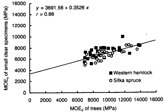
FIG. 8. Relationship of MOE d of trees to MOE s of small, clear specimens.
