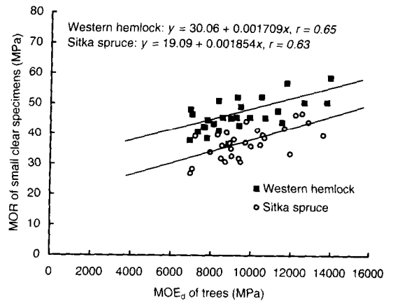
FIG. 9. Relationship of MOE d of trees to MOR of small, clear specimens.
