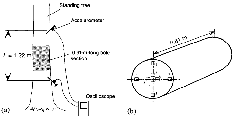
FIG. 2. (a) Experimental setup used in field test, and (b) cutting pattern for small, clear wood specimens.
