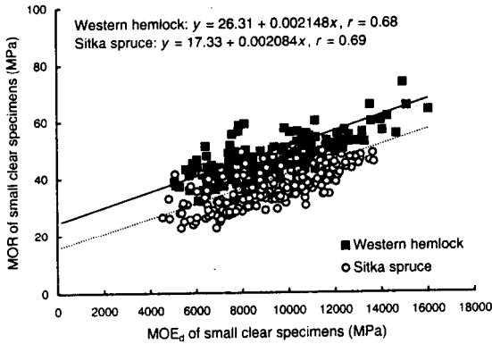
FIG. 6. Relationship of MOE d to MOR for small, clear specimens.
