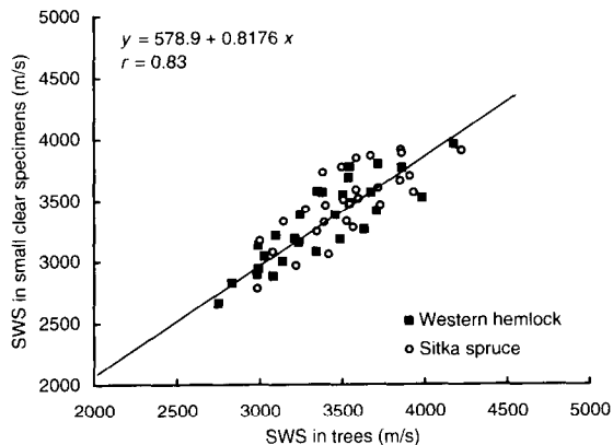
FIG. 4. Relationship of stress wave speed (SWS) measured in trees to SWS measured in small, clear specimens obtained from trees.
