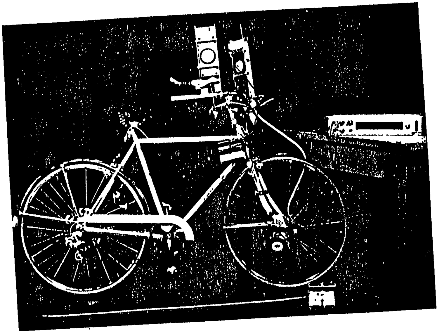
Figure 19. Bicycle Brake Performance Test Equipment-Installed
