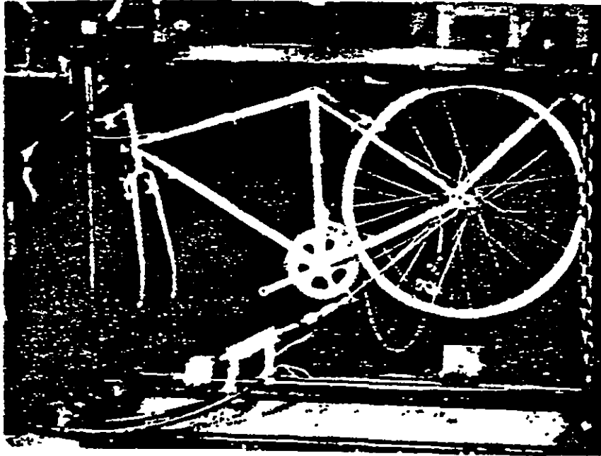
Figure 23. Rear Hub Retention Test
