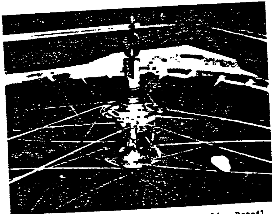
Figure 34. Rim Test Fixture-Axle Coupling Detail
