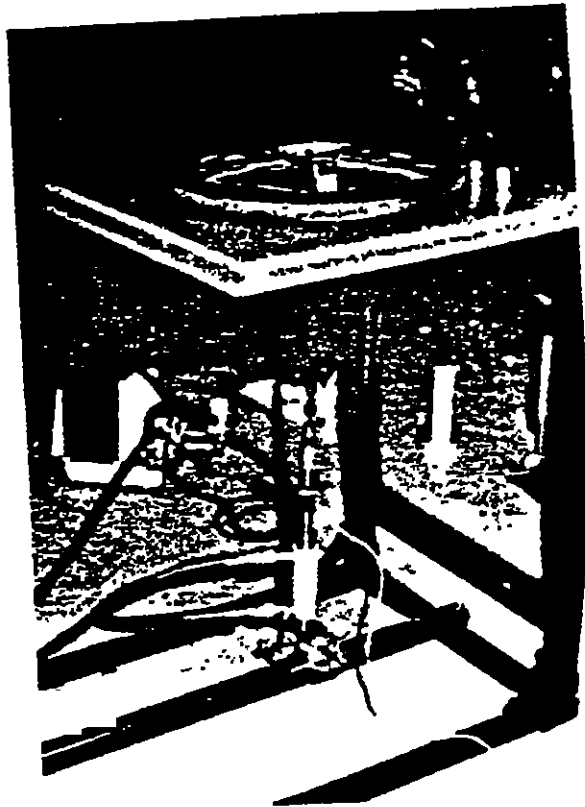
Figure 33. Rim Test Fixture
