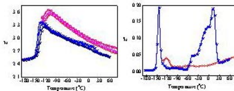
Figure 3. Temperature dependence of ε' and ε'' of PDMS-di-NH 2 (star symbols) and fullerene/PDMS composite film formed at a molar ratio of OH/NH 2 = 2:1 (solid symbols). ε': 0.3 kHz (square), 3 kHz (up triangle), and 30 kHz (circle). ε'': 0.3 kHz.
