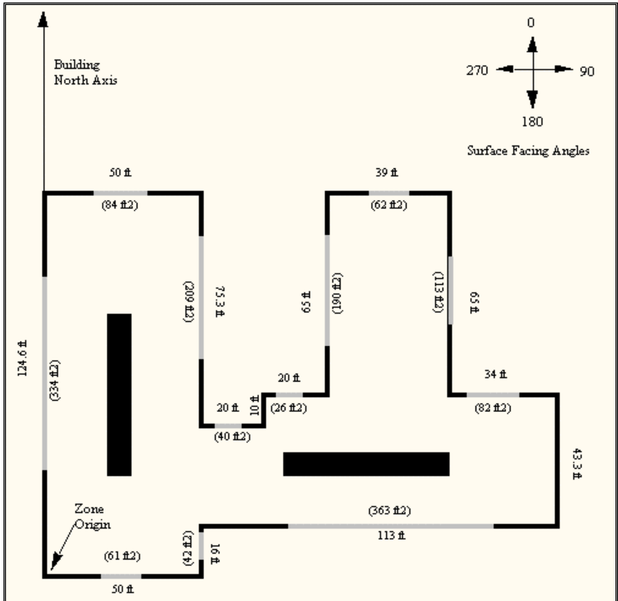
Figure 9. Schematic of One Zone Model with Surface Information.
