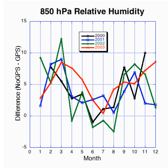
Fig. 3. Percent reduction of 3-h relative humidity forecast error from the 60 km RUC (as in Table 2) due to the inclusion of GPS-IPW data at 850 hPa averaged by month for years 2000 – 2003.
