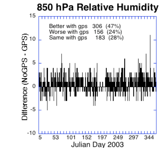
Fig. 4. Percent reduction of 3-h relative humidity forecast error from the 60 km RUC (as in Table 2) due to the inclusion of GPS-IPW data for 850 hPa over calendar year 2003.
