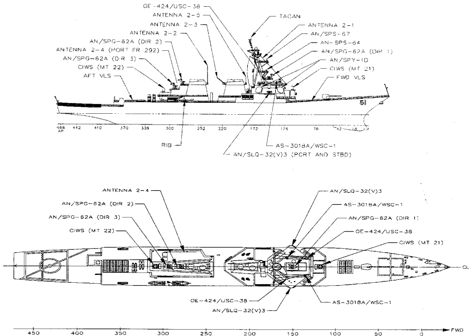
Figure 1. DDG 51 Class Flight I and II Profile and Plan Views
