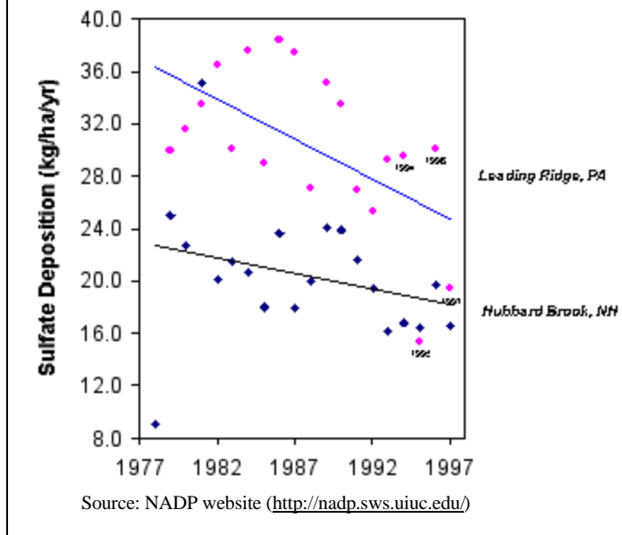
Figure 11. Sulfate Deposition at Two NADP Sites from 1978 to 1997.
