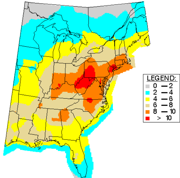
Annual Oxidized Nitrogen (NOx) Deposition in 1990 (kg-N/ha/yr)
