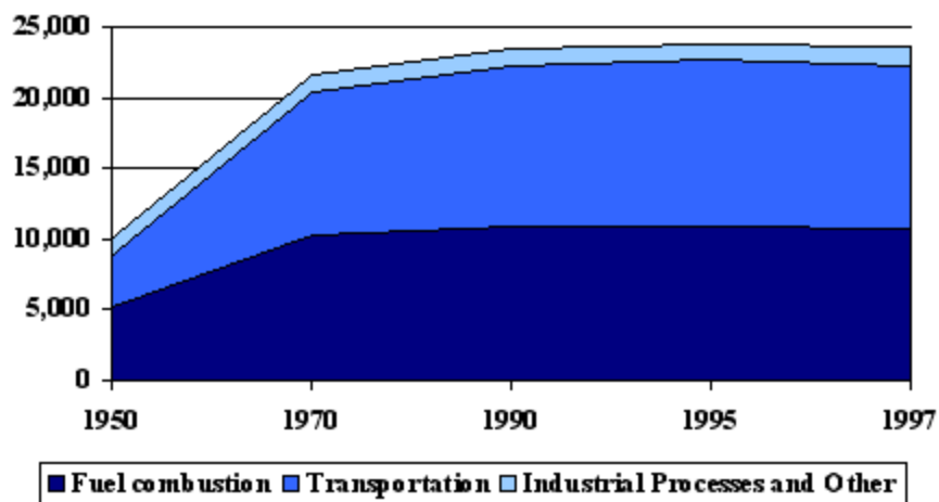
Figure 4. National Emissions of Nitrogen Oxide (in thousand tons).
