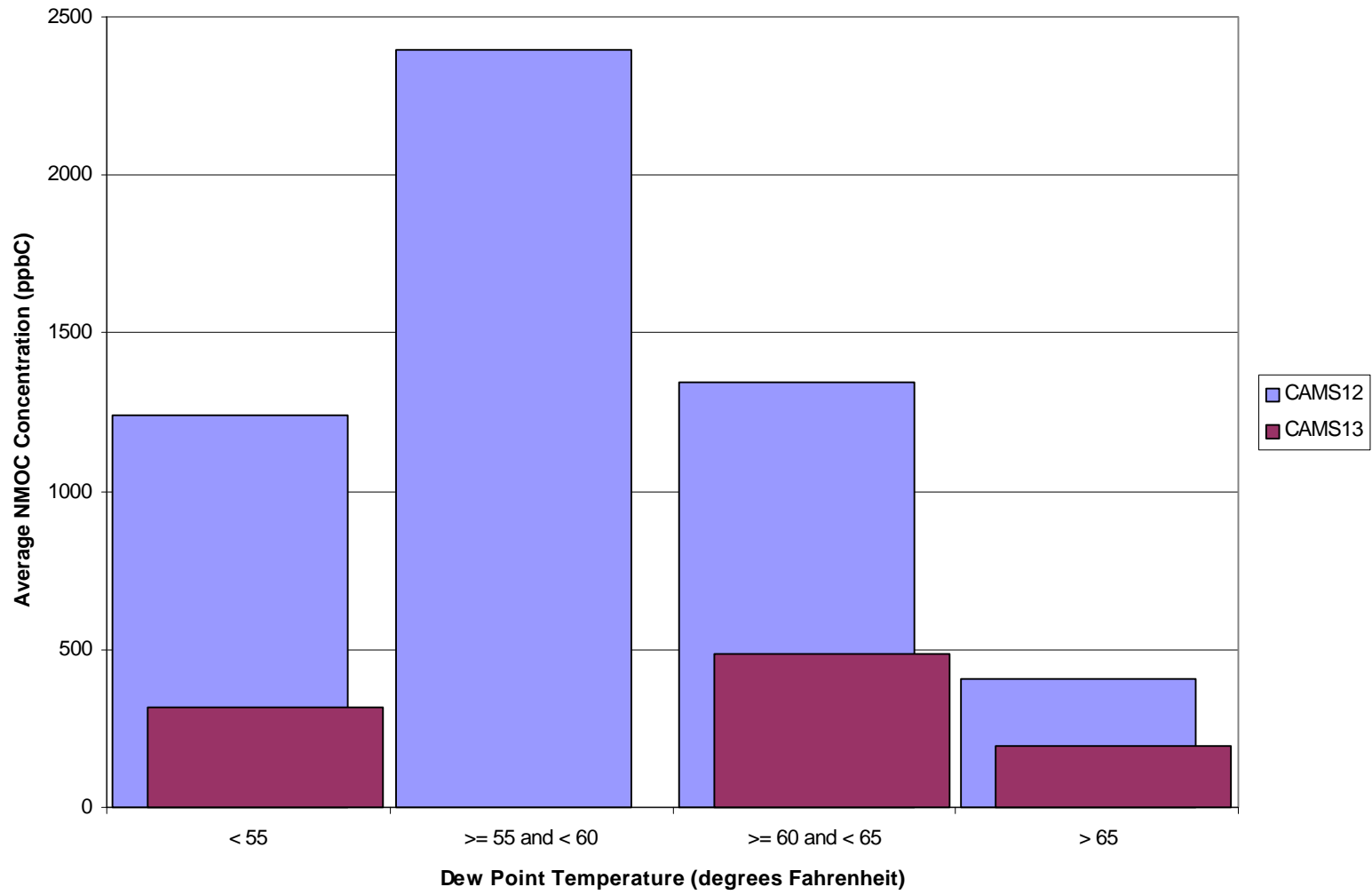
Figure 4-2 Average Dew Point and NMOC Concentrations
