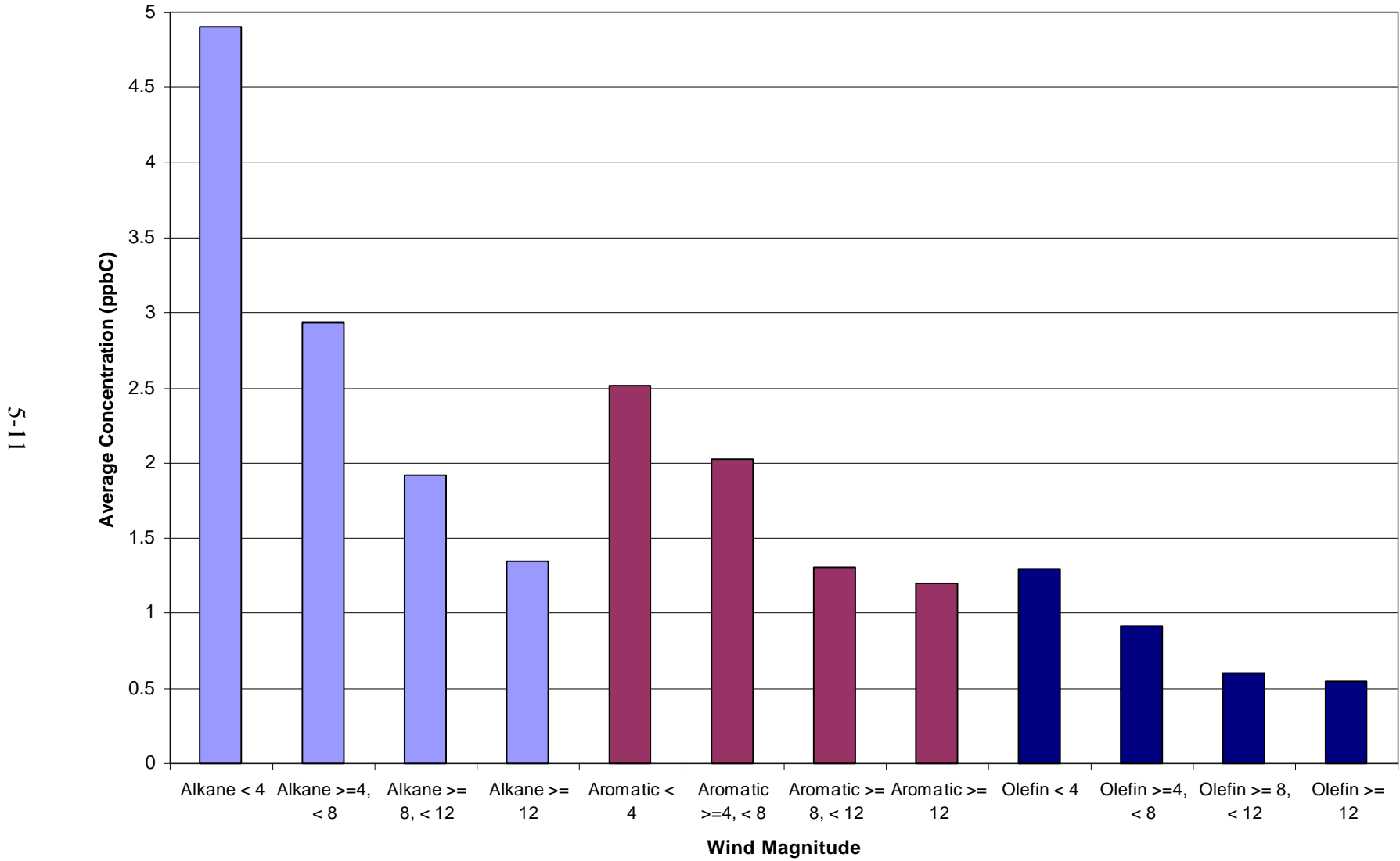
Figure 5-5 CAMS13 (Fort Worth, TX): Average Concentration Compared with Wind Magnitude
