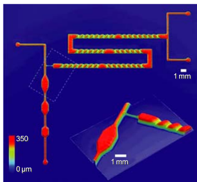
Figure 1: Profilometry image of a fluidics device master prepared by patterning an optical resin. 3-D channel structure is possible due to the frontal polymerization mechanism of the resin.
