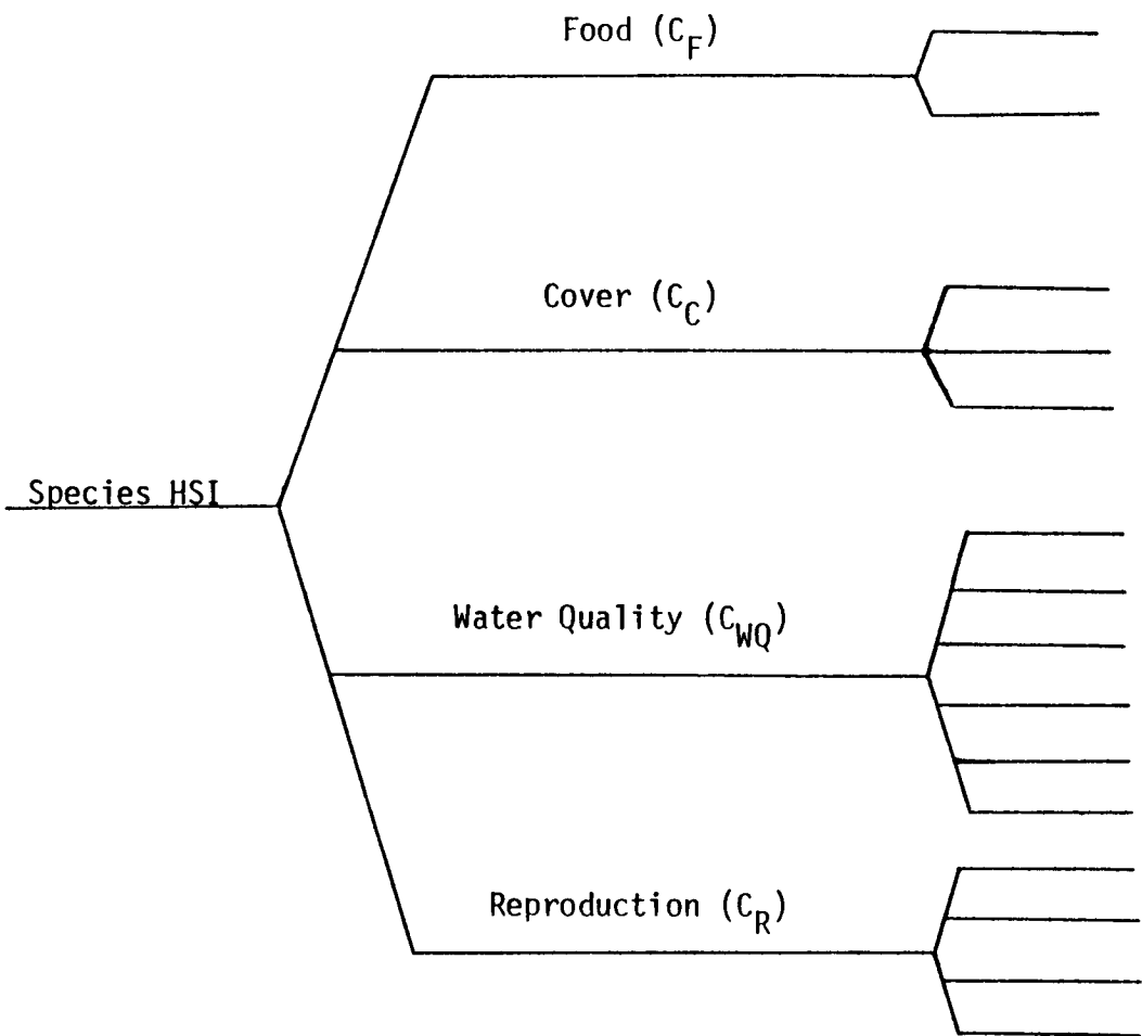
Figure D-1. Schematic diagram of channel catfish habitat model.
