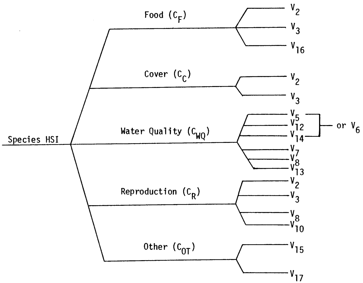
Figure D-2. Variables for each component of the lacustrine version of the channel catfish model.
