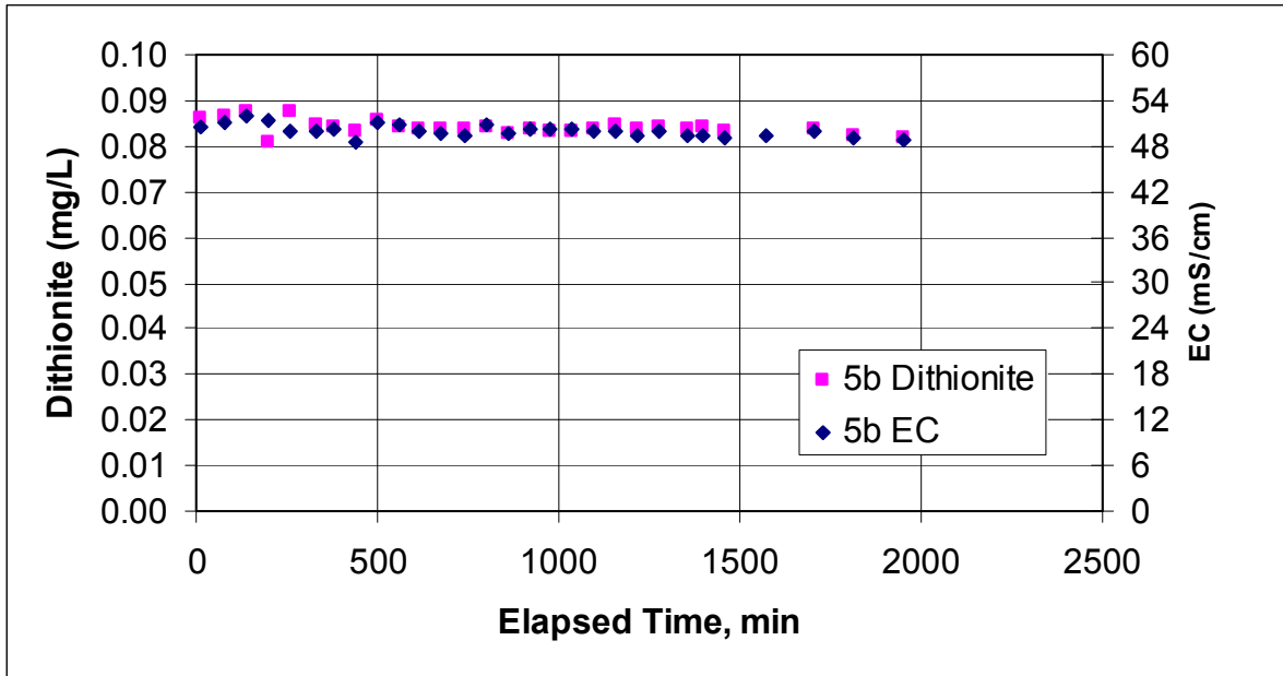
Figure E.18. Dithionite and EC Measurements at Well RA-IW-5b and Injection Stream During the Dithionite Injection Test at the RA-IW-5a/5b Well Pair
