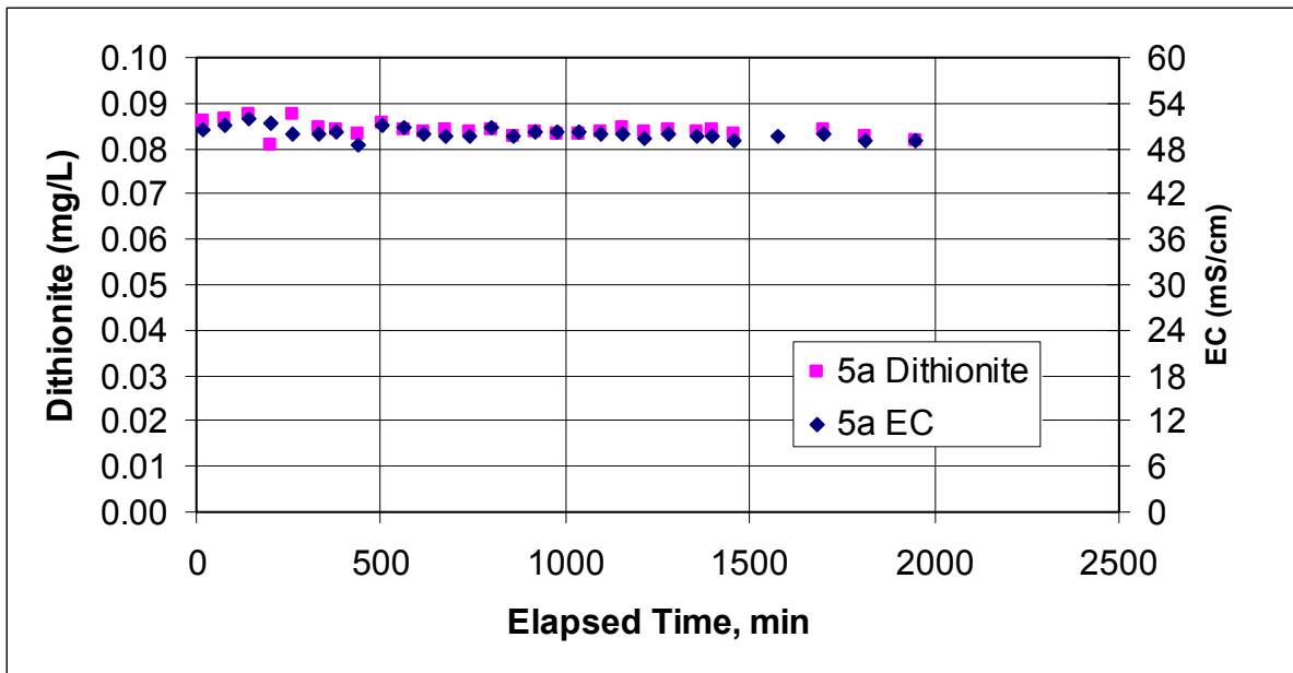
Figure E.17. Dithionite and EC Measurements at Well RA-IW-5a and Injection Stream During the Dithionite Injection Test at the RA-IW-5a/5b Well Pair
