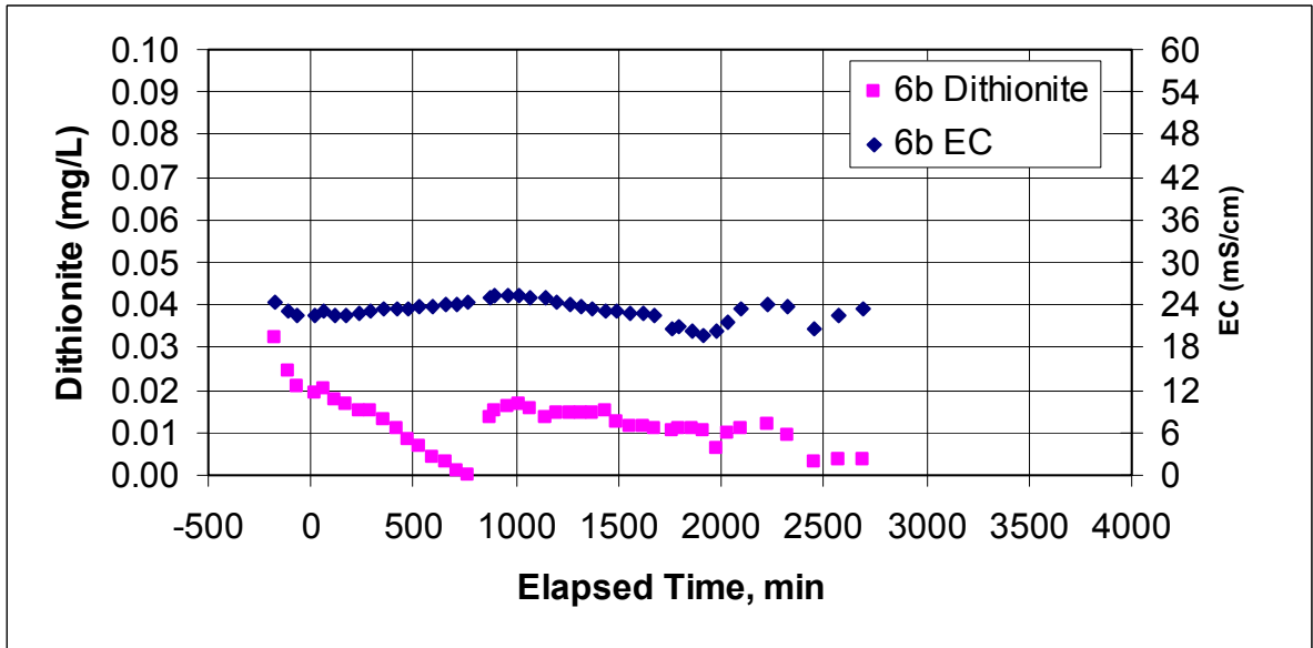
Figure E.37. Dithionite and EC Measurements at Well RA-IW-6b During the Dithionite Injection Test at the RA-IW-7a/7b Well Pair
