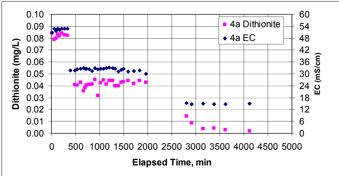
Figure E.9. Dithionite and EC Measurements at Well RA-IW-4a and Injection Stream During the Dithionite Injection Test at the RA-IW-4a/4b Well Pair
