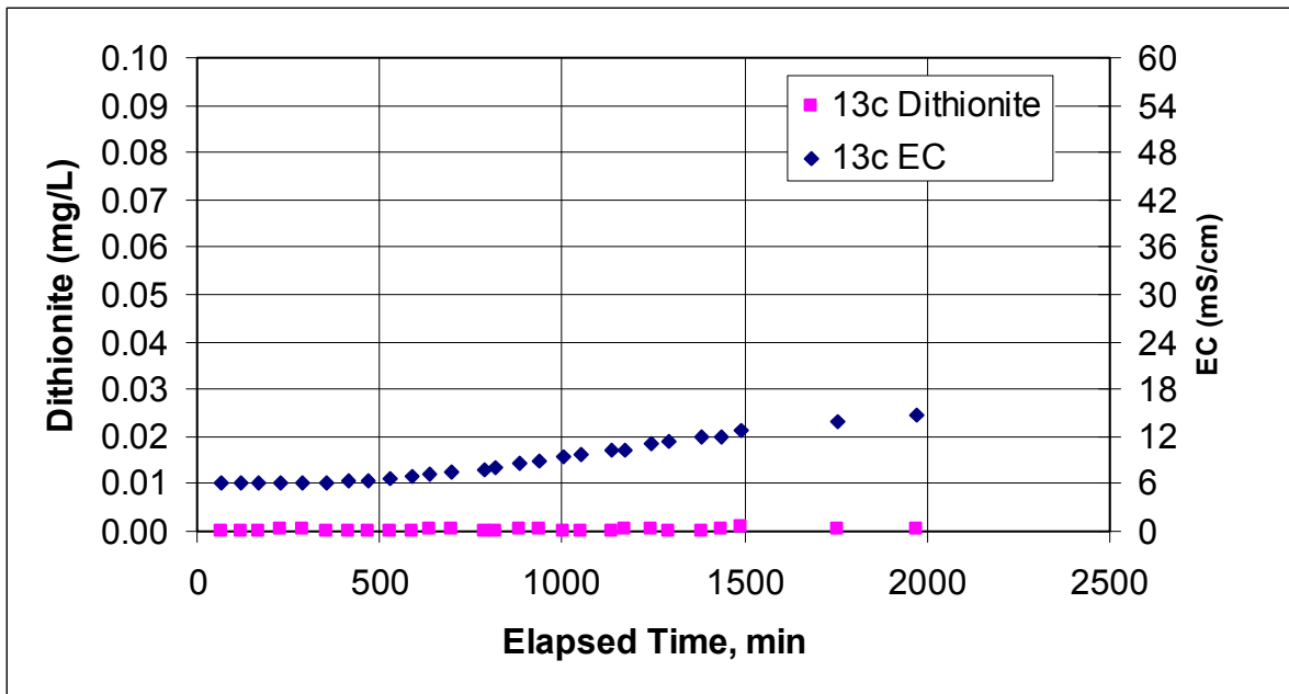
Figure E.23. Dithionite and EC Measurements at Well RA-MW-13c During the Dithionite Injection Test at the RA-IW-5a/5b Well Pair
