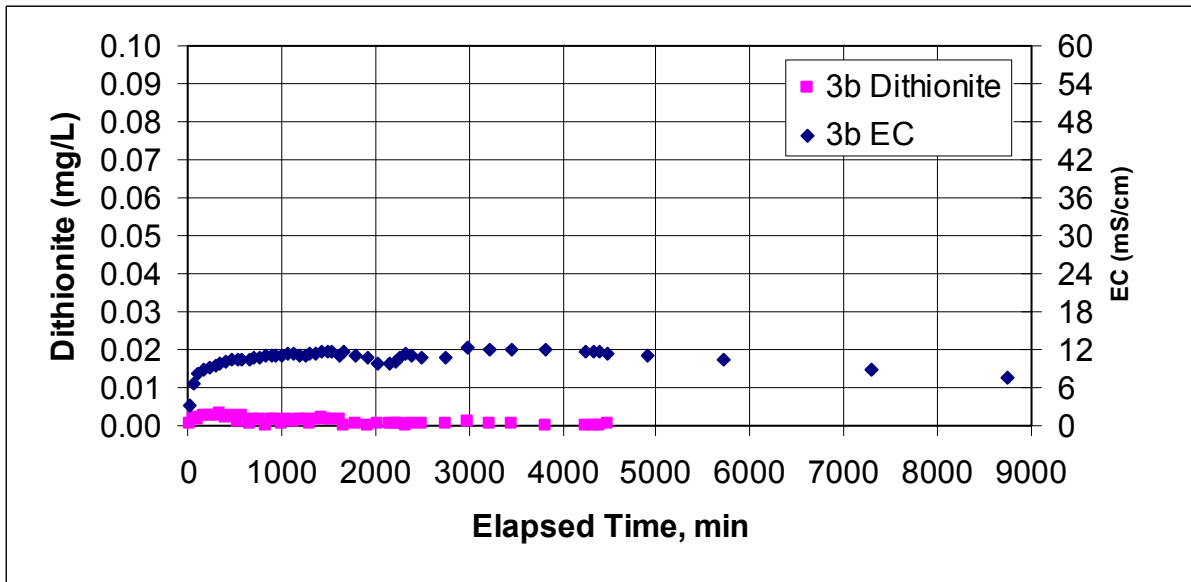
Figure E.5. Dithionite and EC Measurements at Well RA-IW-3b During the Dithionite Injection/Withdrawal Test at the RA-IW-2a/2b Well Pair
