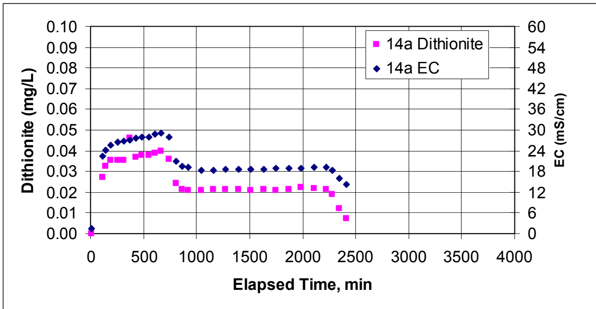
Figure E.29. Dithionite and EC Measurements at Well RA-MW-14a During the Dithionite Injection Test at the RA-IW-6a/6b Well Pair
