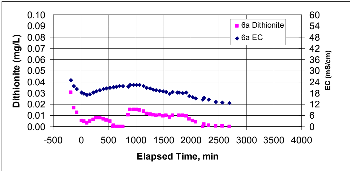
Figure E.36. Dithionite and EC Measurements at Well RA-IW-6a During the Dithionite Injection Test at the RA-IW-7a/7b Well Pair
