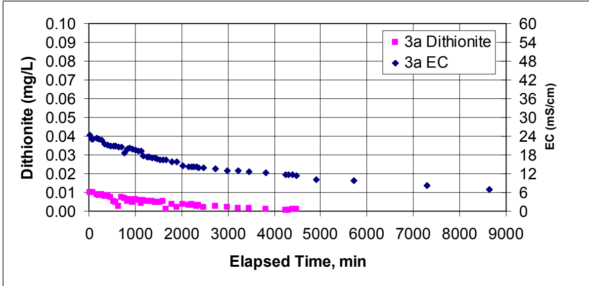
Figure E.4. Dithionite and EC Measurements at Well RA-IW-3a During the Dithionite Injection/Withdrawal Test at the RA-IW-2a/2b Well Pair
