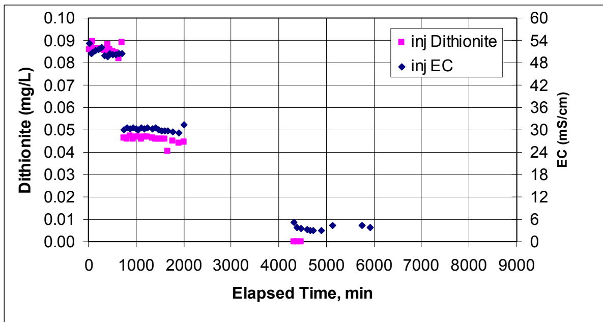
Figure E.1. Dithionite and EC Measurements of the Injection and Withdrawal Streams During the Dithionite Injection/Withdrawal Test at the RA-IW-2a/2b Well Pair
