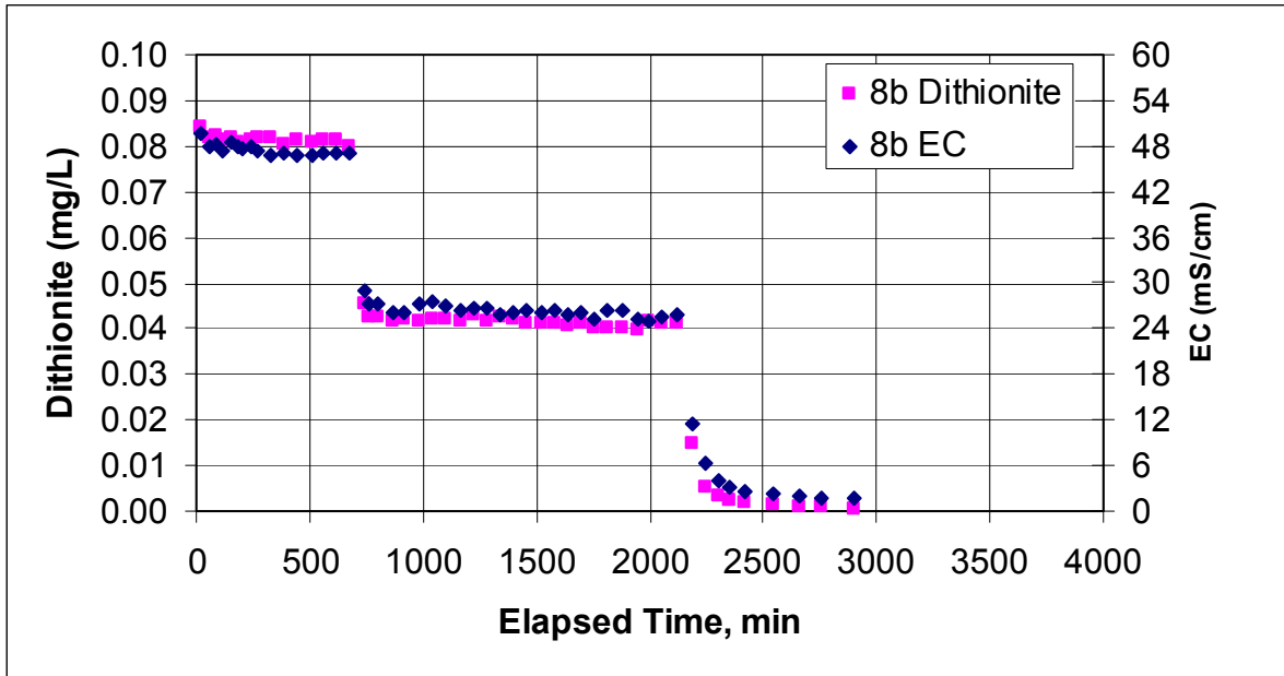
Figure E.42. Dithionite and EC Measurements at Well RA-IW-8b and Injection Stream During the Dithionite Injection Test at the RA-IW-8a/8b Well Pair
