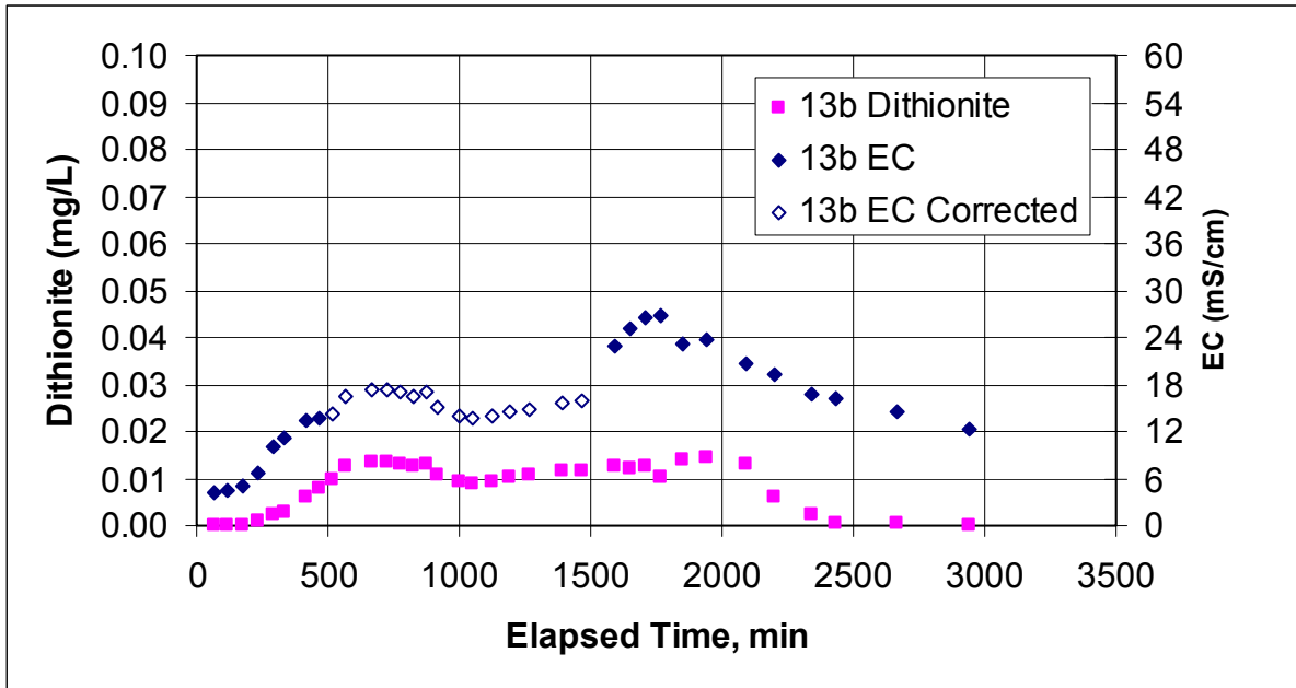
Figure E.50. Dithionite and EC Measurements at Well RA-MW-13b During Dithionite Injection Test at Well Pair INJ1/INJ2
