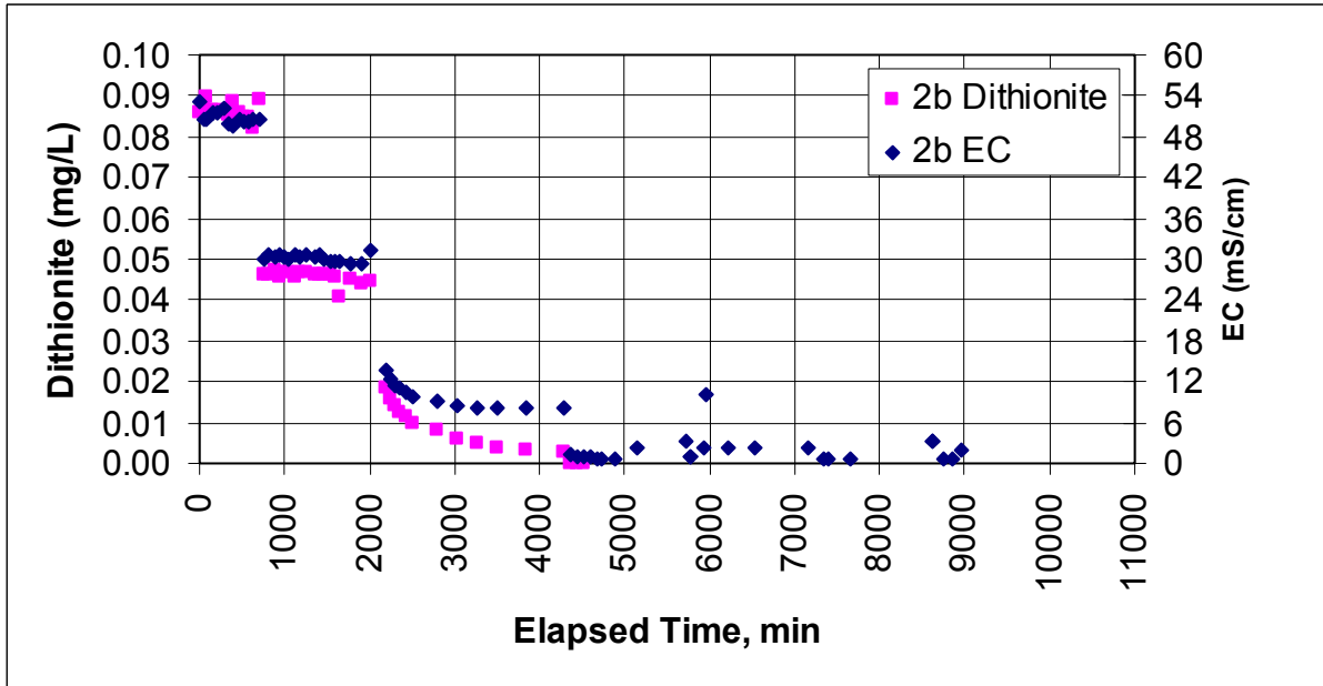
Figure E.3. Dithionite and EC Measurements at Well RA-IW-2b During the Dithionite Injection/Withdrawal Test at the RA-IW-2a/2b Well Pair
