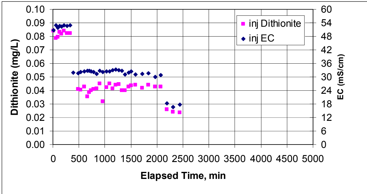
Figure E.8. Dithionite and EC Measurements of the Injection Stream During the Dithionite Injection Test at the RA-IW-4a/4b Well Pair
