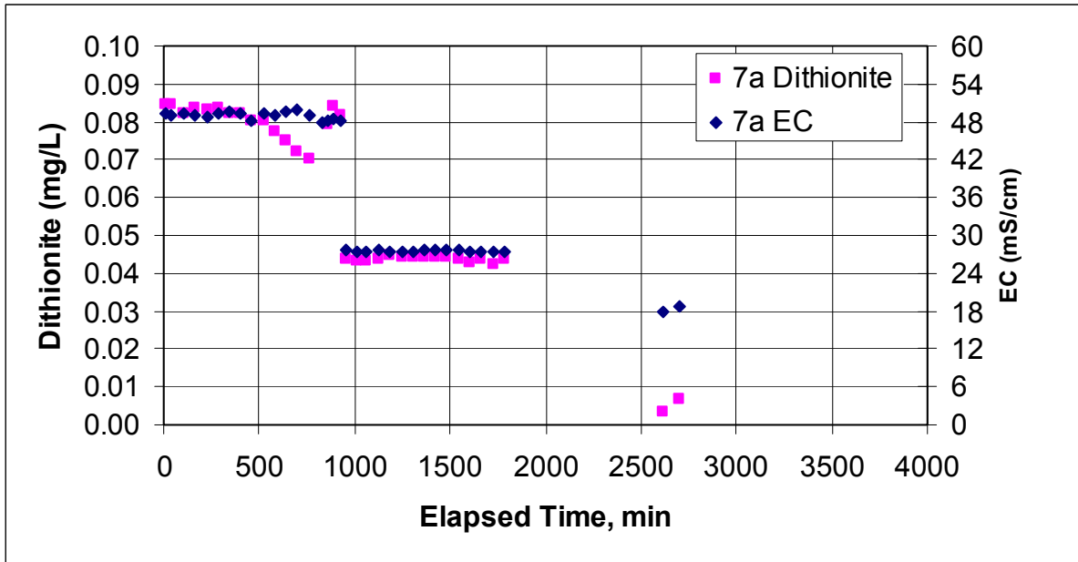
Figure E.34. Dithionite and EC Measurements at Well RA-IW-7a and Injection Stream During the Dithionite Injection Test at the RA-IW-7a/7b Well Pair
