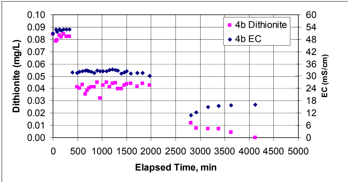
Figure E.10. Dithionite and EC Measurements at Well RA-IW-4b and Injection Stream During the Dithionite Injection Test at the RA-IW-4a/4b Well Pair
