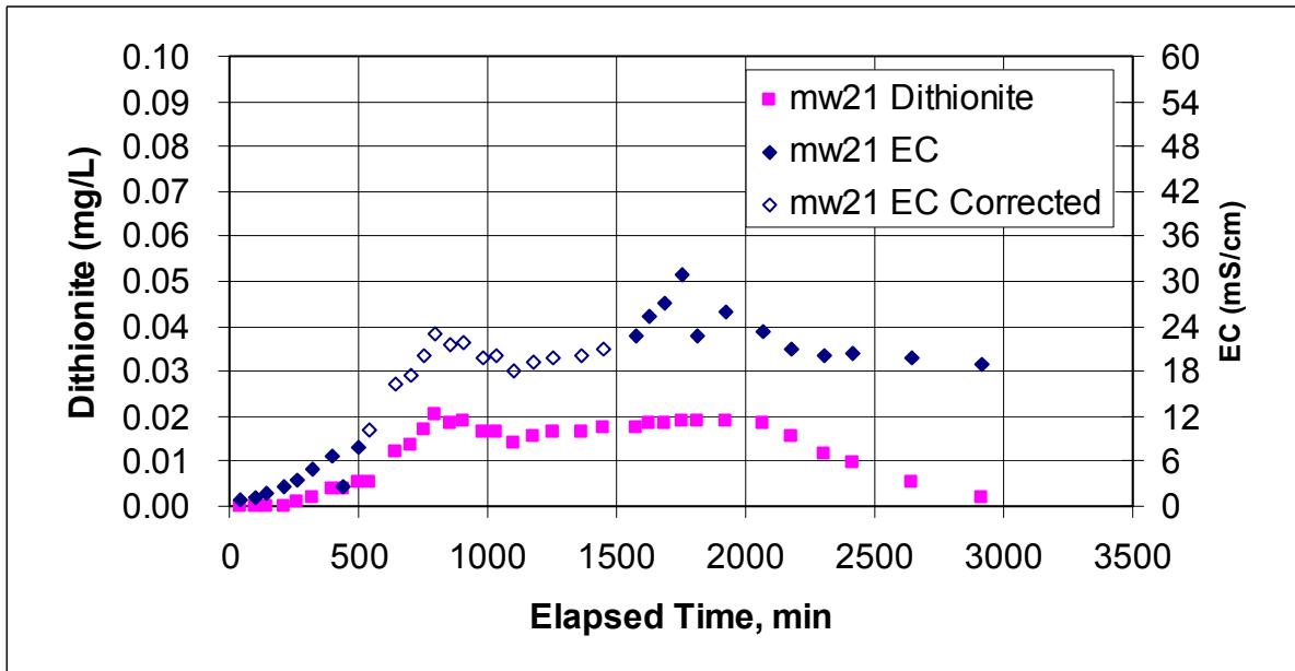
Figure E.47. Dithionite and EC Measurements at Well MW-21 During the Dithionite Injection Test at Well Pair INJ1/INJ2
