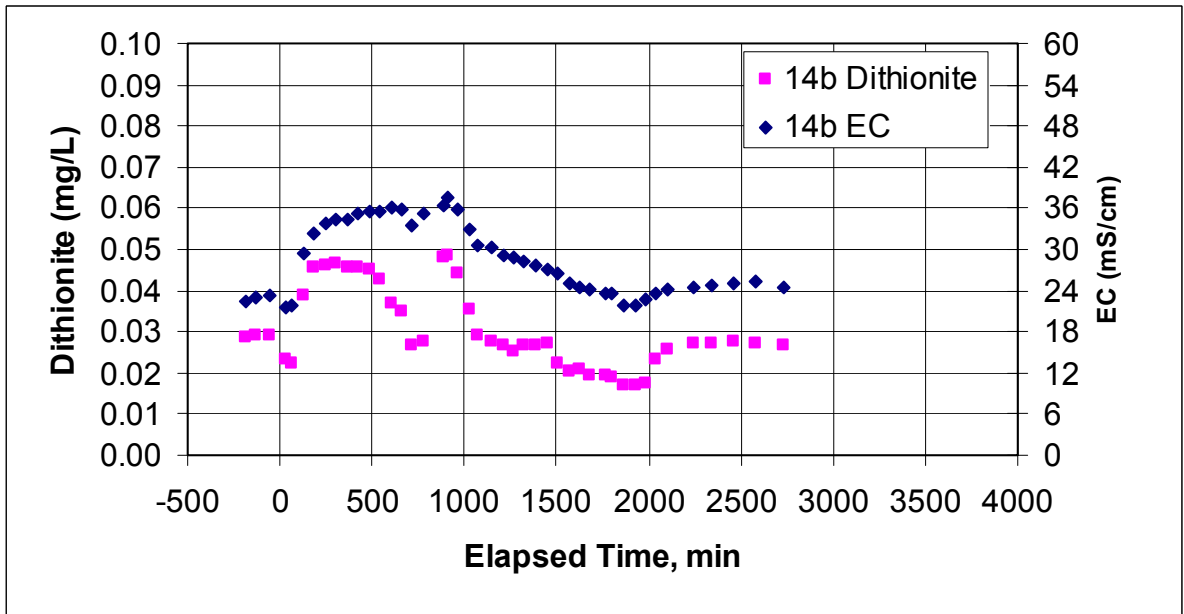
Figure E.39. Dithionite and EC Measurements at Well RA-MW-14b During the Dithionite Injection Test at the RA-IW-7a/7b Well Pair
