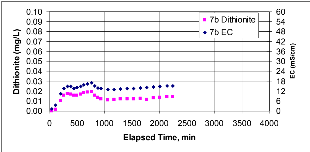
Figure E.28. Dithionite and EC Measurements at Well RA-IW-7b During the Dithionite Injection Test at the RA-IW-6a/6b Well Pair
