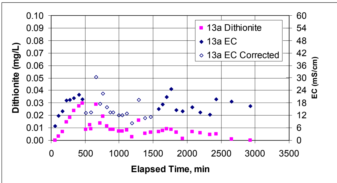
Figure E.49. Dithionite and EC Measurements at Well RA-MW-13a During Dithionite Injection Test at Well Pair INJ1/INJ2
