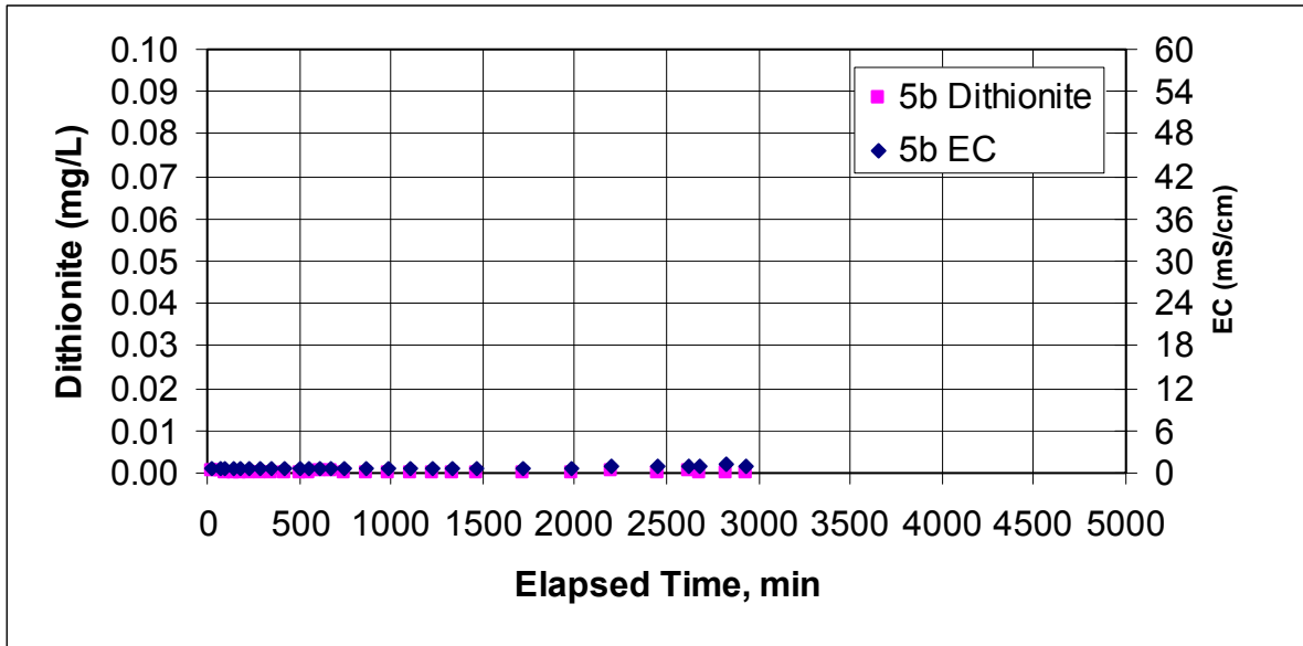
Figure E.12. Dithionite and EC Measurements at Well RA-IW-5b During the Dithionite Injection Test at the RA-IW-4a/4b Well Pair
