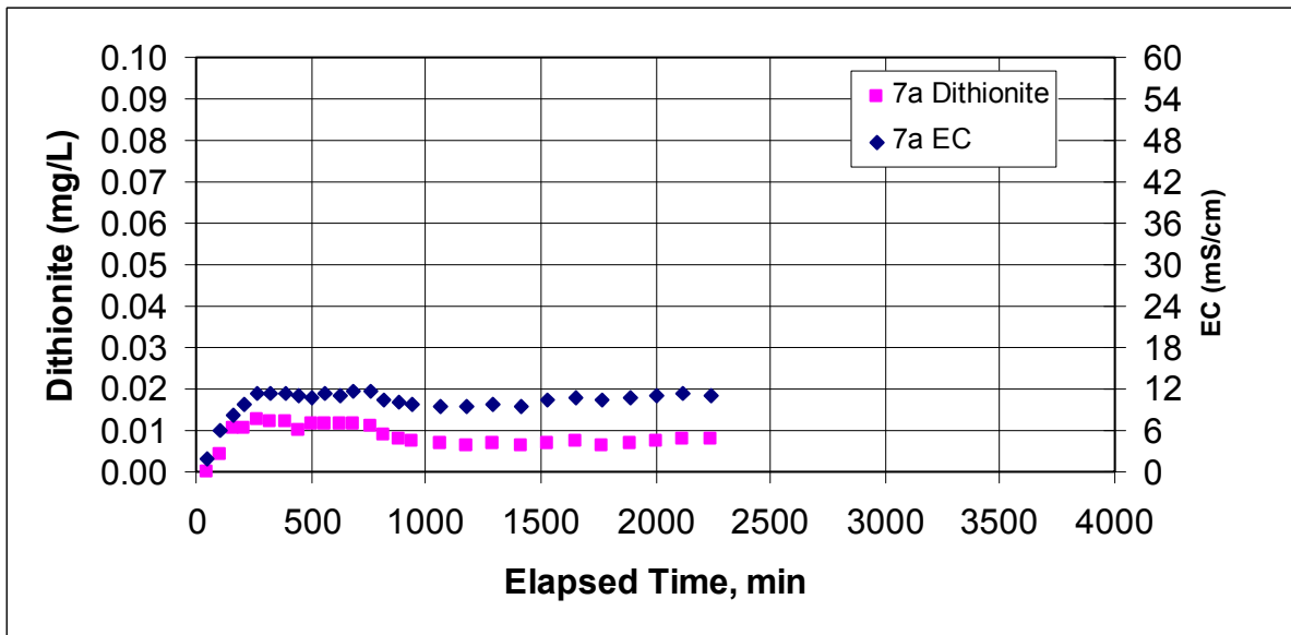
Figure E.27. Dithionite and EC Measurements at Well RA-IW-7a During the Dithionite Injection Test at the RA-IW-6a/6b Well Pair
