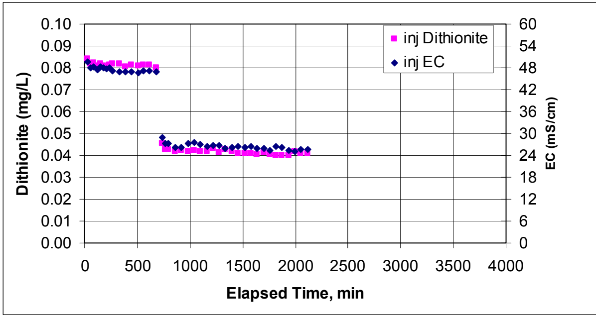
Figure E.40. Dithionite and EC Measurements of the Injection Stream During the Dithionite Injection Test at the RA-IW-8a/8b Well Pair
