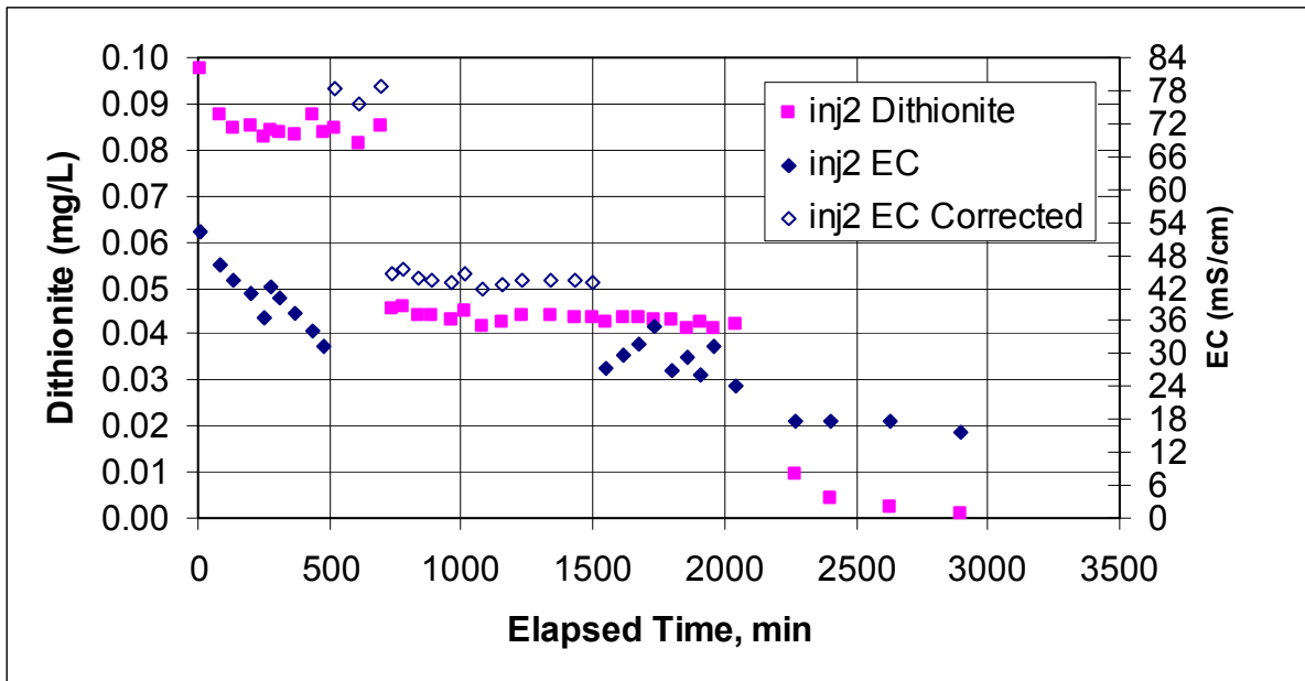
Figure E.45. Dithionite and EC Measurements at Well INJ2 and Injection Stream During Dithionite Injection Test at Well Pair INJ1/INJ2
