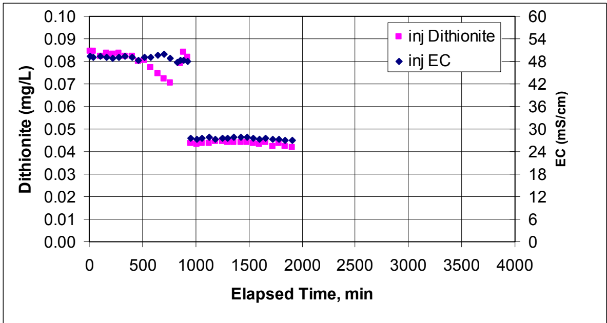
Figure E.33. Dithionite and EC Measurements of the Injection Stream During the Dithionite Injection Test at the RA-IW-7a/7b Well Pair
