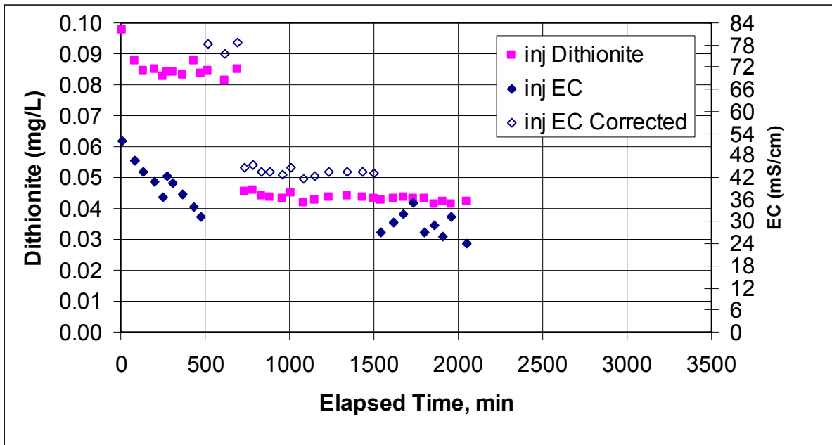
Figure E.43. Dithionite and EC Measurements of the Injection Stream During the Dithionite Injection Test at Well Pair INJ1/INJ2
