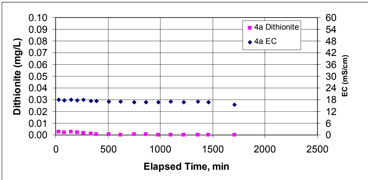
Figure E.19. Dithionite and EC Measurements at Well RA-IW-4a During the Dithionite Injection Test at the RA-IW-5a/5b Well Pair
