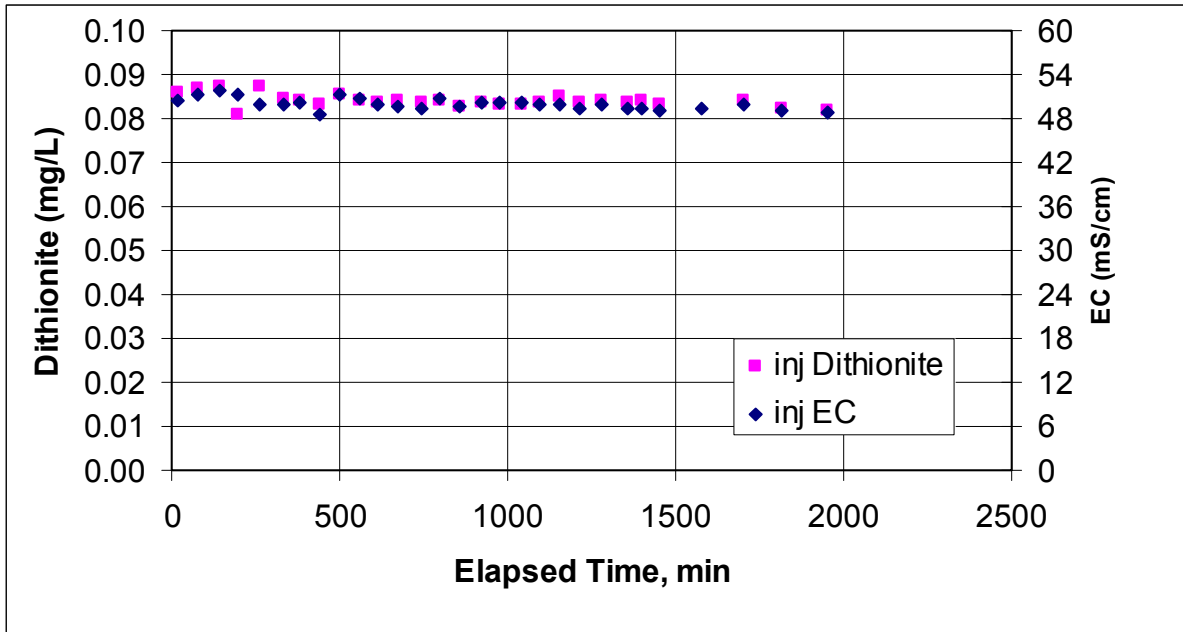
Figure E.16. Dithionite and EC Measurements of the Injection Stream During the Dithionite Injection Test at the RA-IW-5a/5b Well Pair
