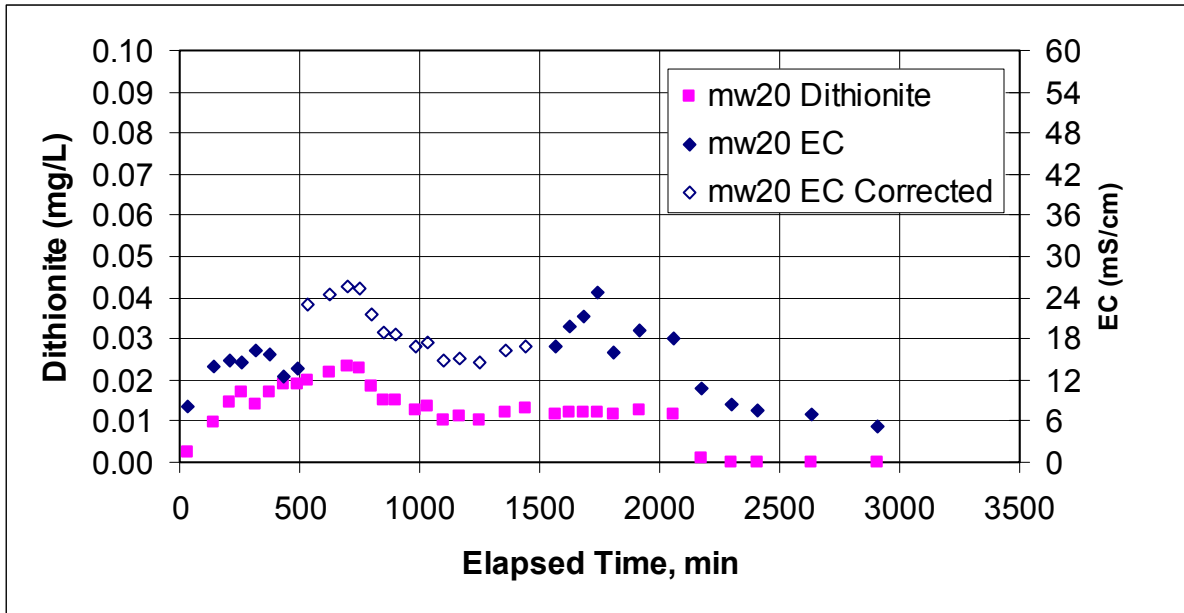
Figure E.46. Dithionite and EC Measurements at Well MW-20 During the Dithionite Injection Test at Well Pair INJ1/INJ2
