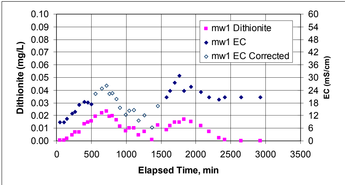
Figure E.48. Dithionite and EC Measurements at Well MW-1 During the Dithionite Injection Test at Well Pair INJ1/INJ2
