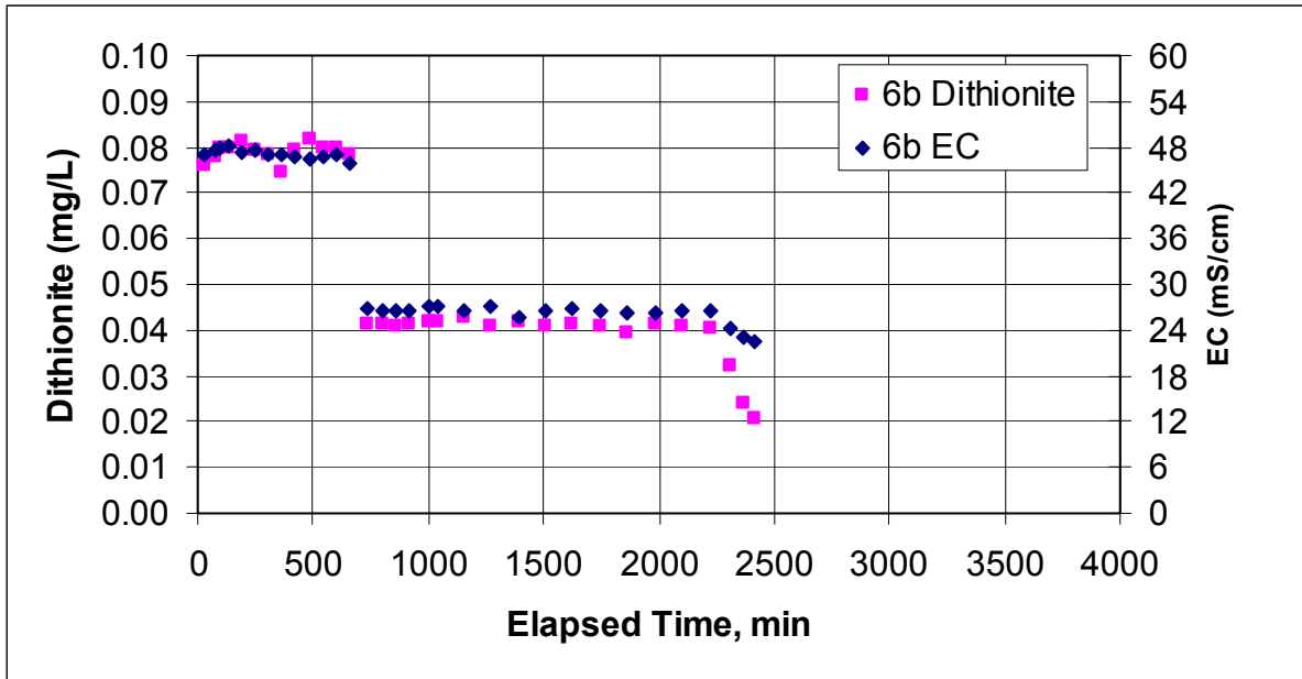
Figure E.26. Dithionite and EC Measurements at Well RA-IW-6b and Injection Stream During the Dithionite Injection Test at the RA-IW-6a/6b Well Pair
