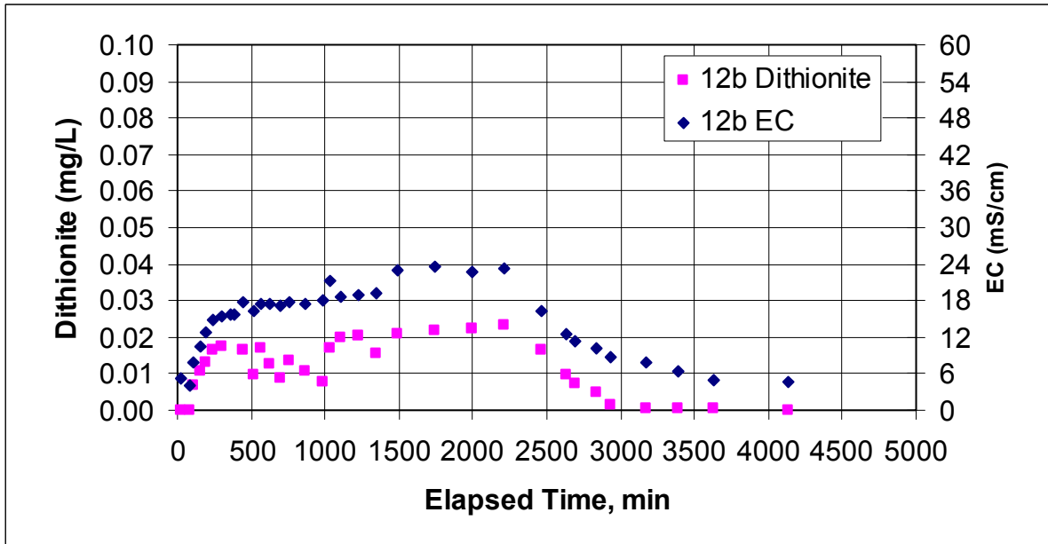
Figure E.14. Dithionite and EC Measurements at Well RA-MW-12b During the Dithionite Injection Test at the RA-IW-4a/4b Well Pair
