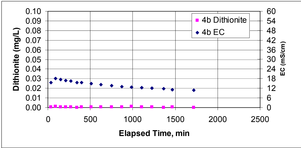
Figure E.20. Dithionite and EC Measurements at Well RA-IW-4b During the Dithionite Injection Test at the RA-IW-5a/5b Well Pair
