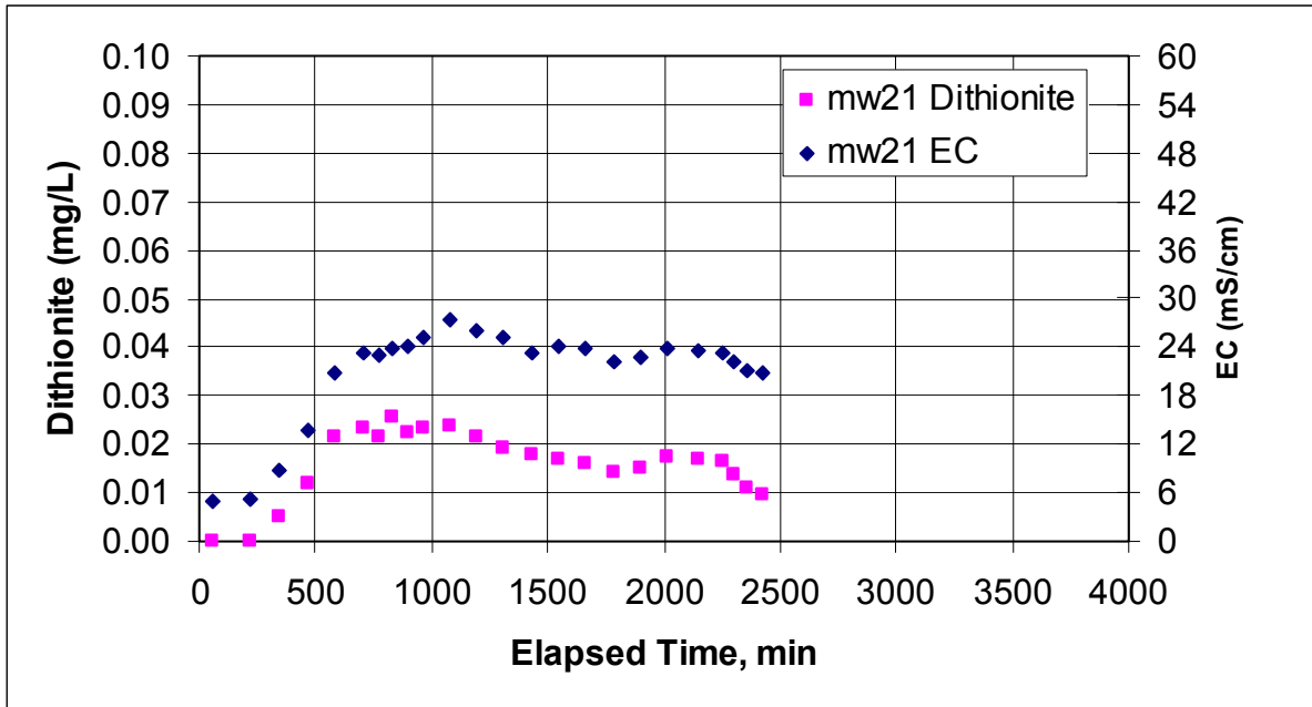
Figure E.32. Dithionite and EC Measurements at Well MW-21 During the Dithionite Injection Test at the RA-IW-6a/6b Well Pair
