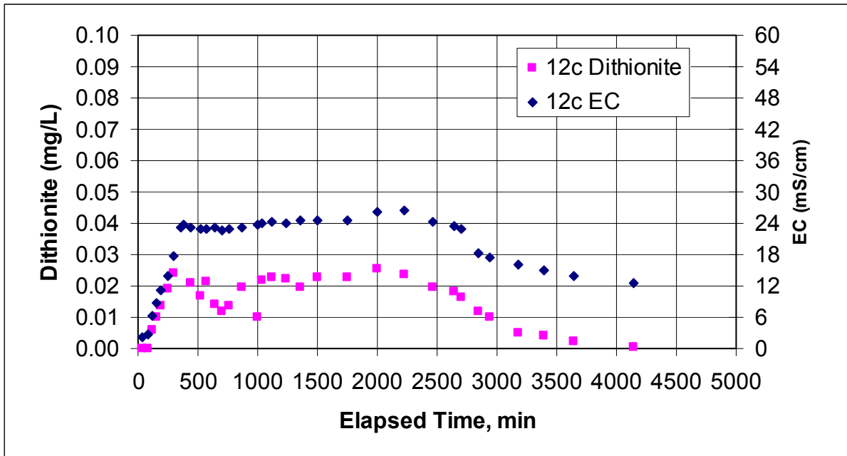
Figure E.15. Dithionite and EC Measurements at Well RA-MW-12c During the Dithionite Injection Test at the RA-IW-4a/4b Well Pair
