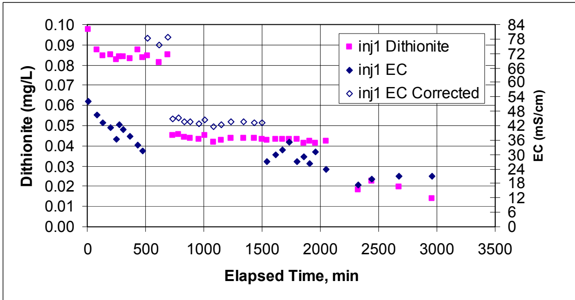
Figure E.44. Dithionite and EC Measurements at Well INJ1 and Injection Stream During the Dithionite Injection Test at Well Pair INJ1/INJ2
