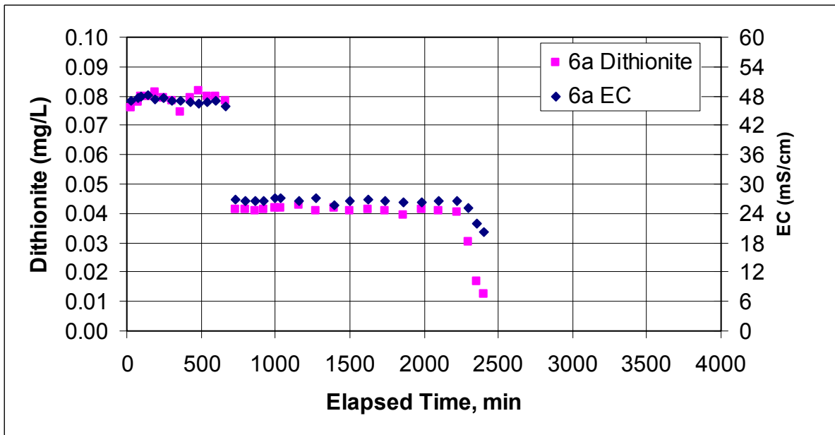
Figure E.25. Dithionite and EC Measurements at Well RA-IW-6a and Injection Stream During the Dithionite Injection Test at the RA-IW-6a/6b Well Pair
