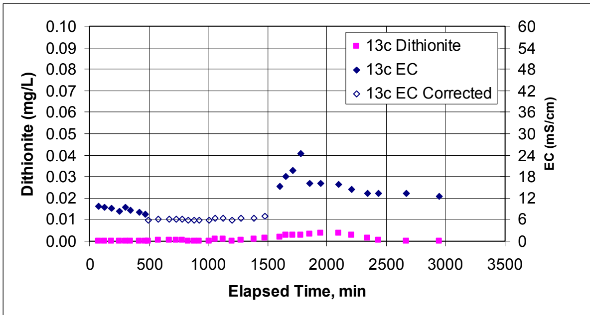
Figure E.51. Dithionite and EC Measurements at Well RA-MW-13c During Dithionite Injection Test at Well Pair INJ1/INJ2
