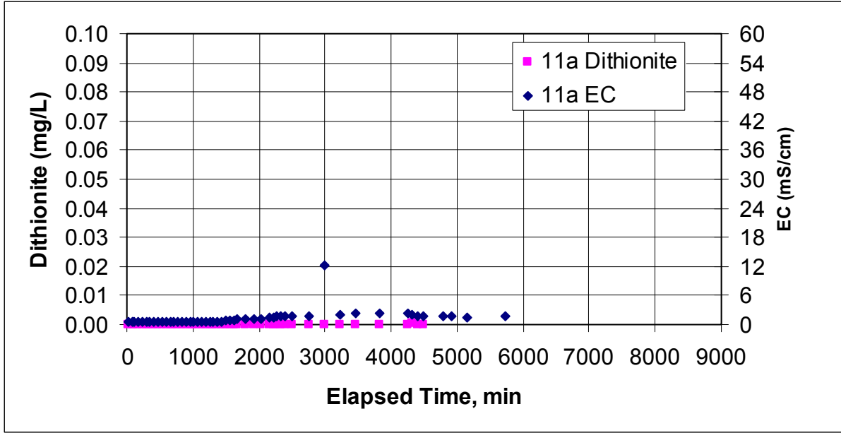
Figure E.6. Dithionite and EC Measurements at Well RA-MW-11a During the Dithionite Injection/Withdrawal Test at the RA-IW-2a/2b Well Pair
