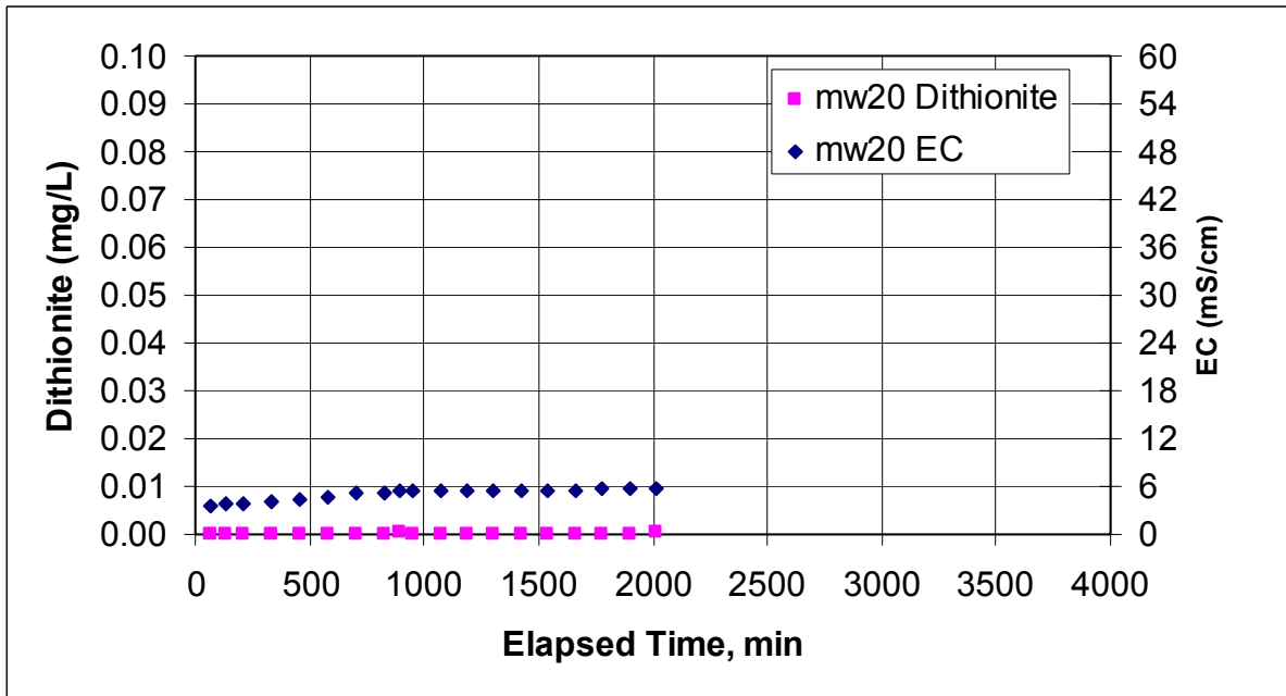
Figure E.31. Dithionite and EC Measurements at Well MW-20 During the Dithionite Injection Test at the RA-IW-6a/6b Well Pair
