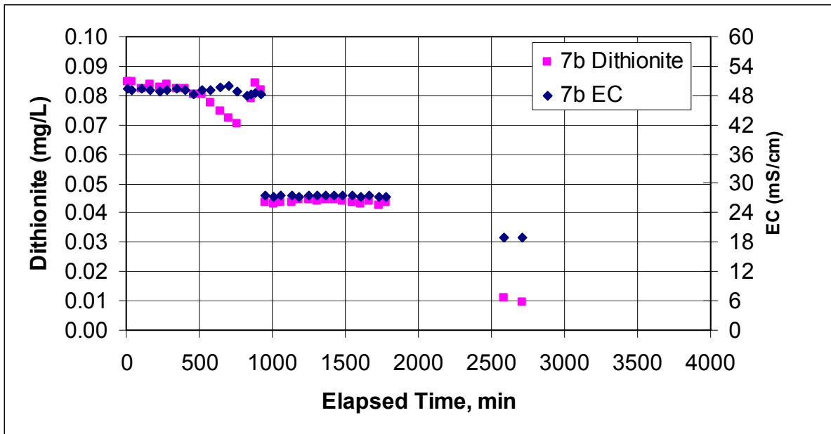
Figure E.35. Dithionite and EC Measurements at Well RA-IW-7b and Injection Stream During the Dithionite Injection Test at the RA-IW-7a/7b Well Pair
