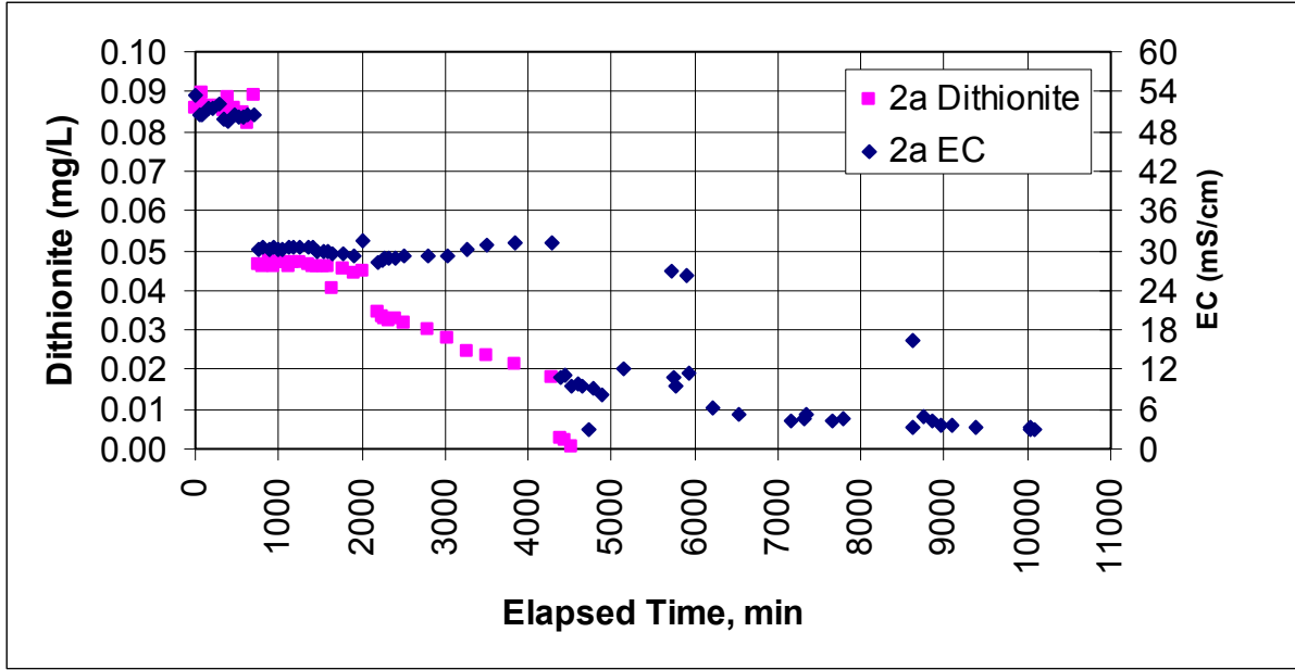
Figure E.2. Dithionite and EC Measurements at Well RA-IW-2a During the Dithionite Injection/Withdrawal Test at the RA-IW-2a/2b Well Pair
