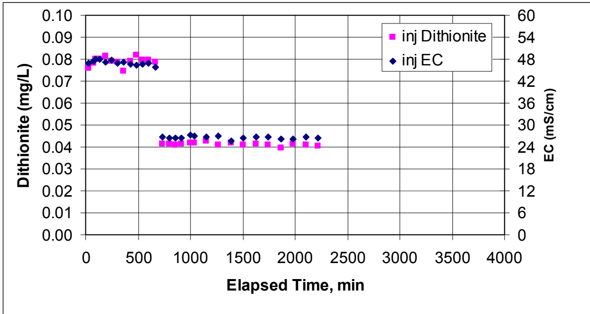
Figure E.24. Dithionite and EC Measurements of the Injection Stream During the Dithionite Injection Test at the RA-IW-6a/6b Well Pair
