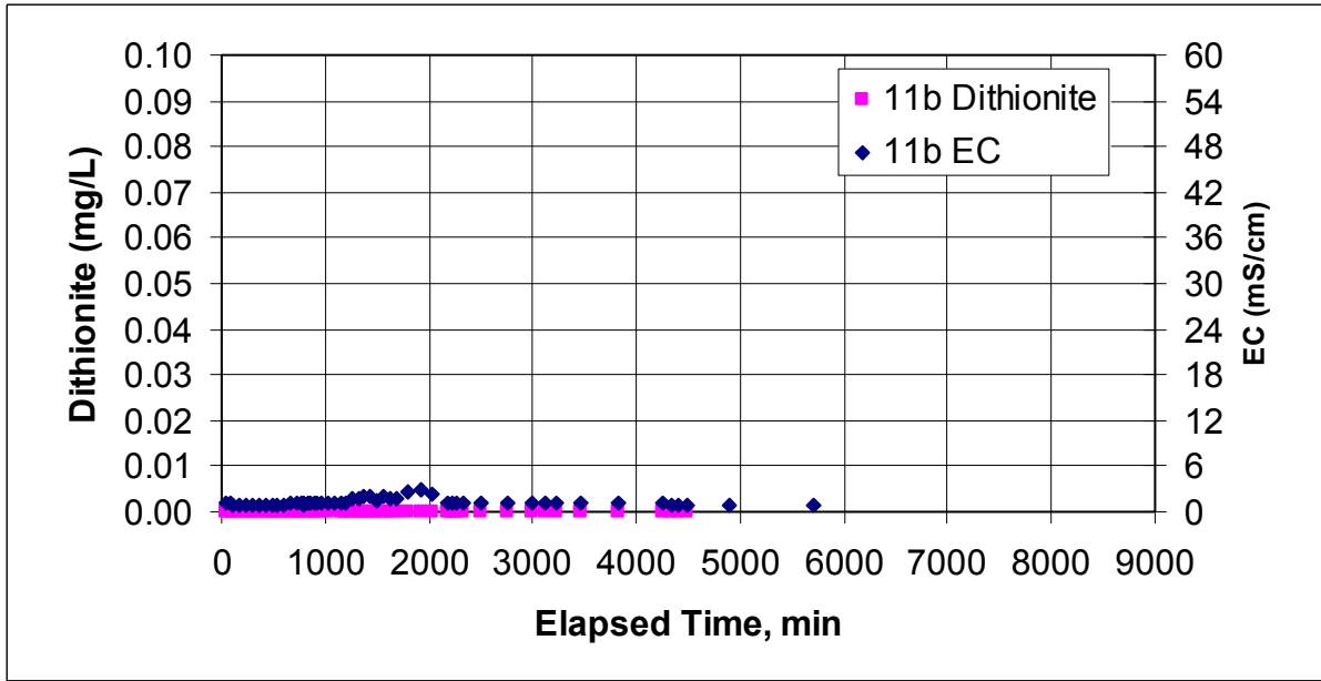
Figure E.7. Dithionite and EC Measurements at Well RA-MW-11b During the Dithionite Injection/Withdrawal Test at the RA-IW-2a/2b Well Pair
