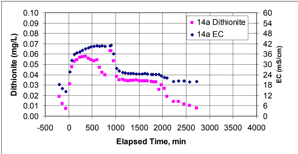
Figure E.38. Dithionite and EC Measurements at Well RA-MW-14a During Dithionite Injection Test at the RA-IW-7a/7b Well Pair
