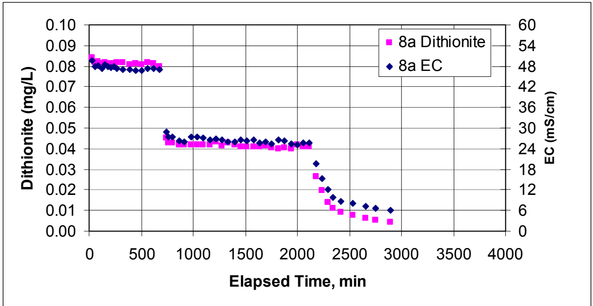
Figure E.41. Dithionite and EC Measurements at Well RA-IW-8a and Injection Stream During the Dithionite Injection Test at the RA-IW-8a/8b Well Pair
