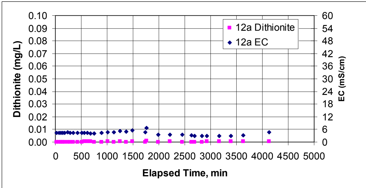
Figure E.13. Dithionite and EC Measurements at Well RA-MW-12a During the Dithionite Injection Test at the RA-IW-4a/4b Well Pair
