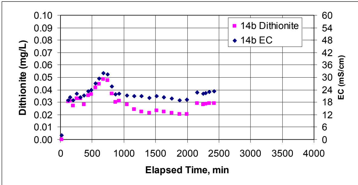
Figure E.30. Dithionite and EC Measurements at Well RA-MW-14b During the Dithionite Injection Test at the RA-IW-6a/6b Well Pair
