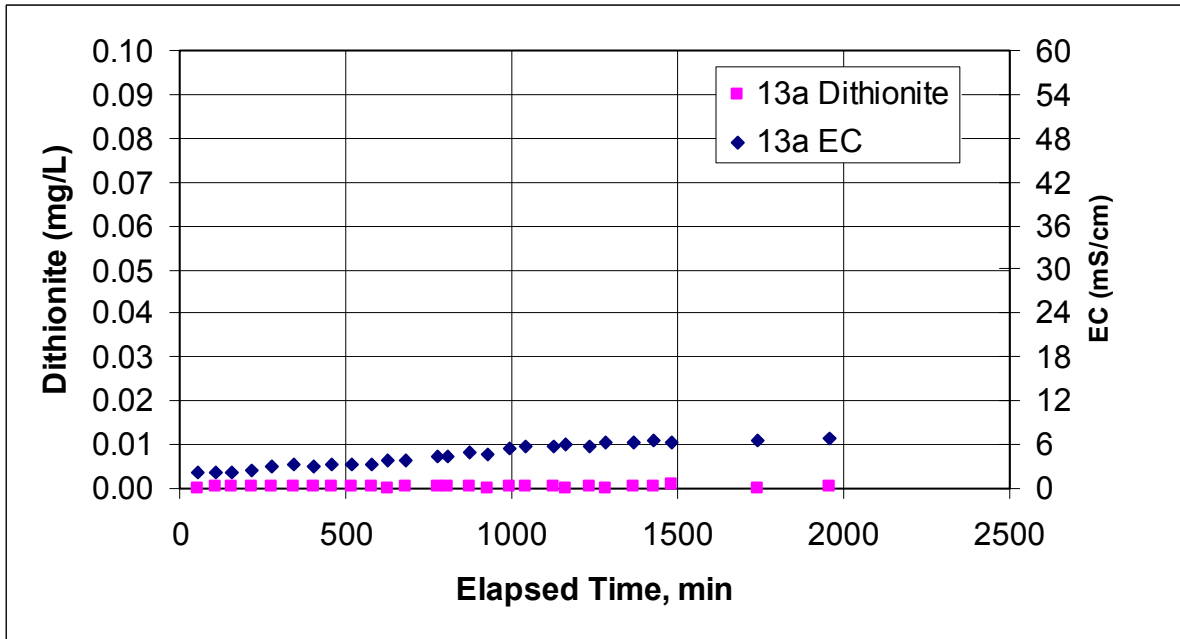
Figure E.21. Dithionite and EC Measurements at Well RA-MW-13a During the Dithionite Injection Test at the RA-IW-5a/5b Well Pair
