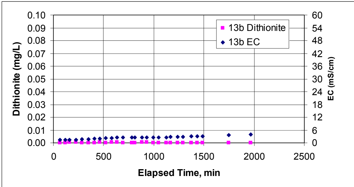
Figure E.22. Dithionite and EC Measurements at Well RA-MW-13b During the Dithionite Injection Test at the RA-IW-5a/5b Well Pair
