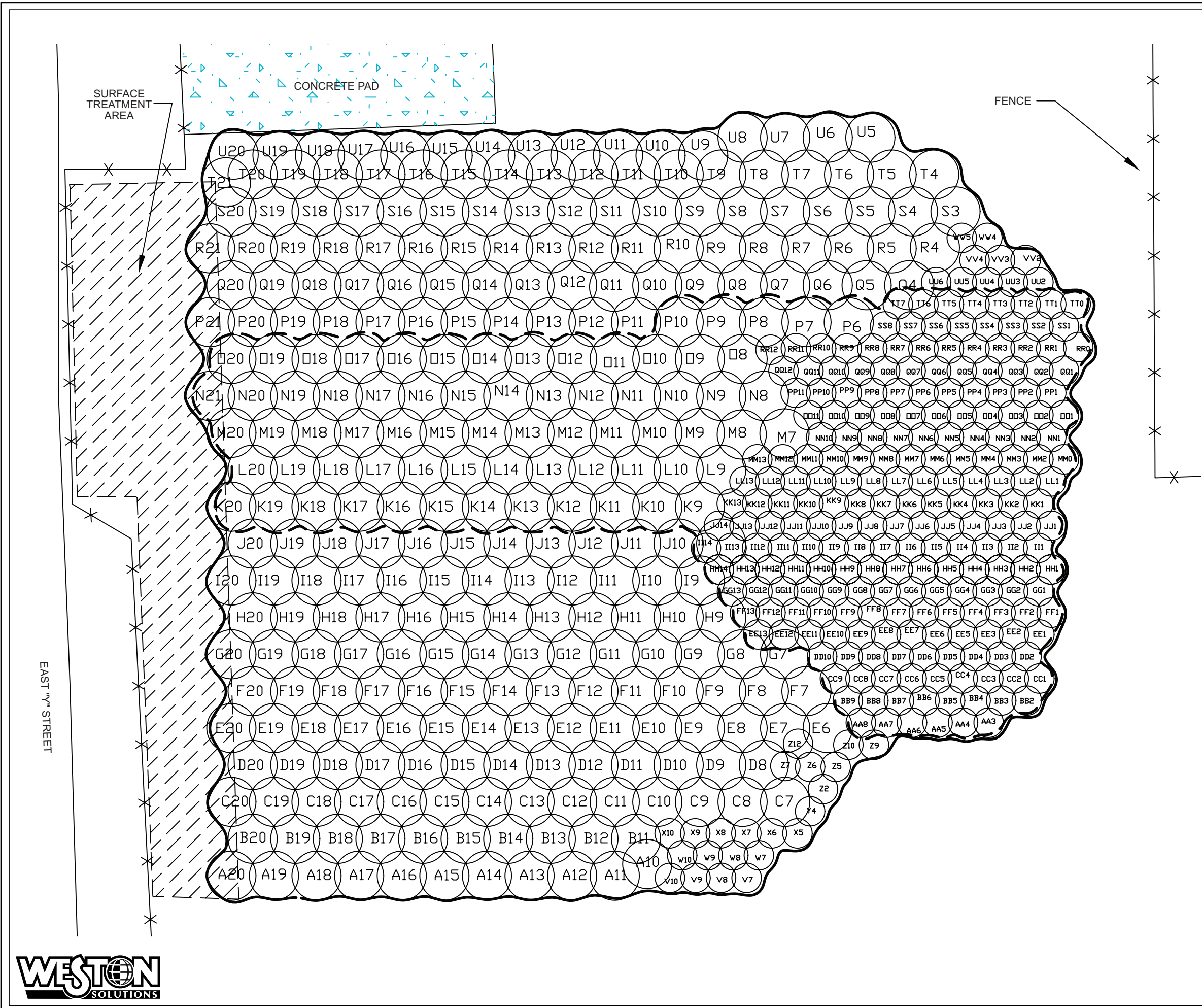
Frontier Hard Chrome Soil Treatment Column Locations
