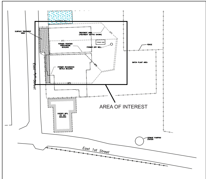
Frontier Hard Chrome Soil Treatment Column Locations
