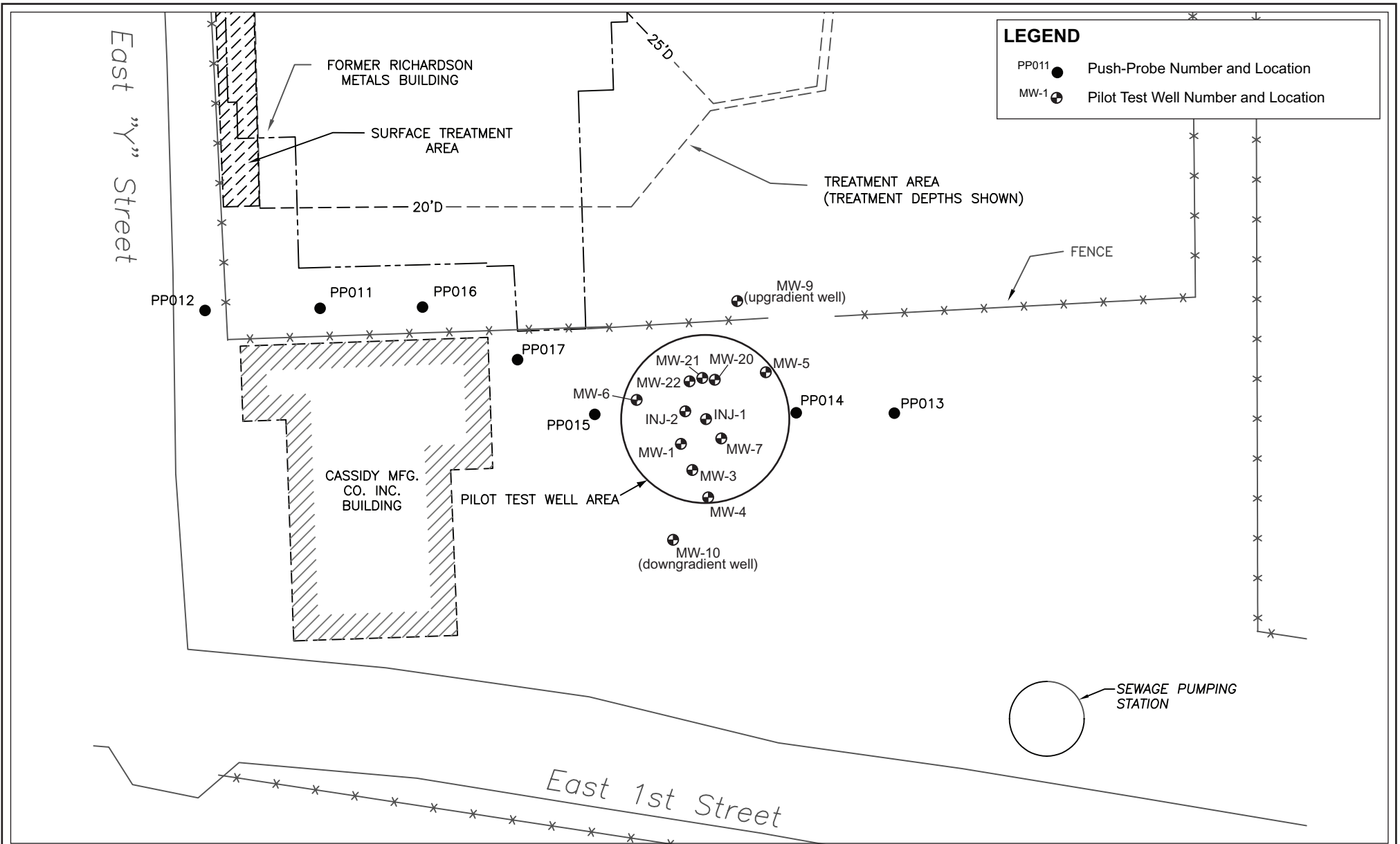
Frontier Hard Chrome ISRM Wall Alignment Characterization Push-Probe Locations
