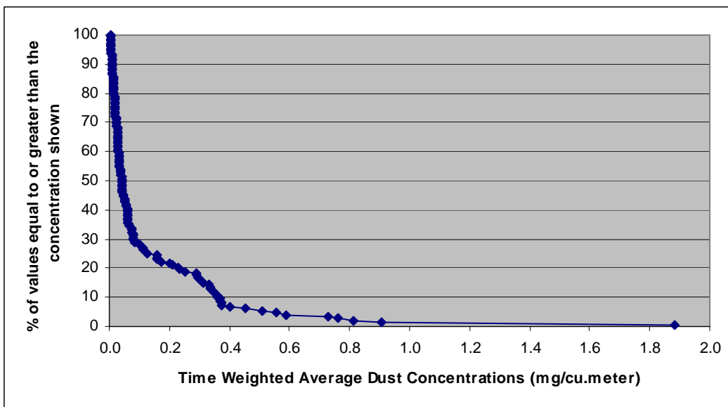
Figure 12 – Perimeter Air Dust Concentrations
