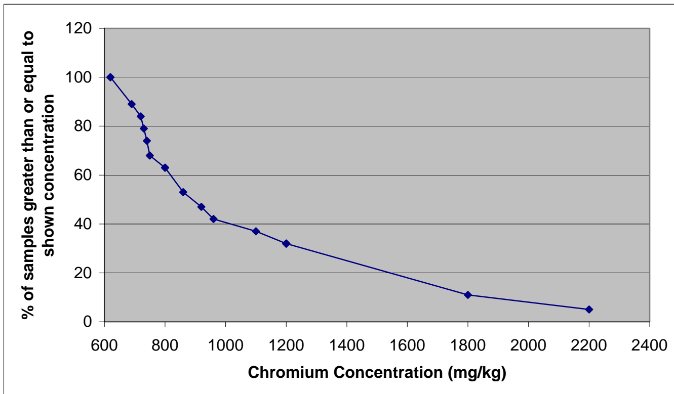
Figure 7 – Fluff Soil Total Chromium Concentrations (Weston subcontracted lab)
