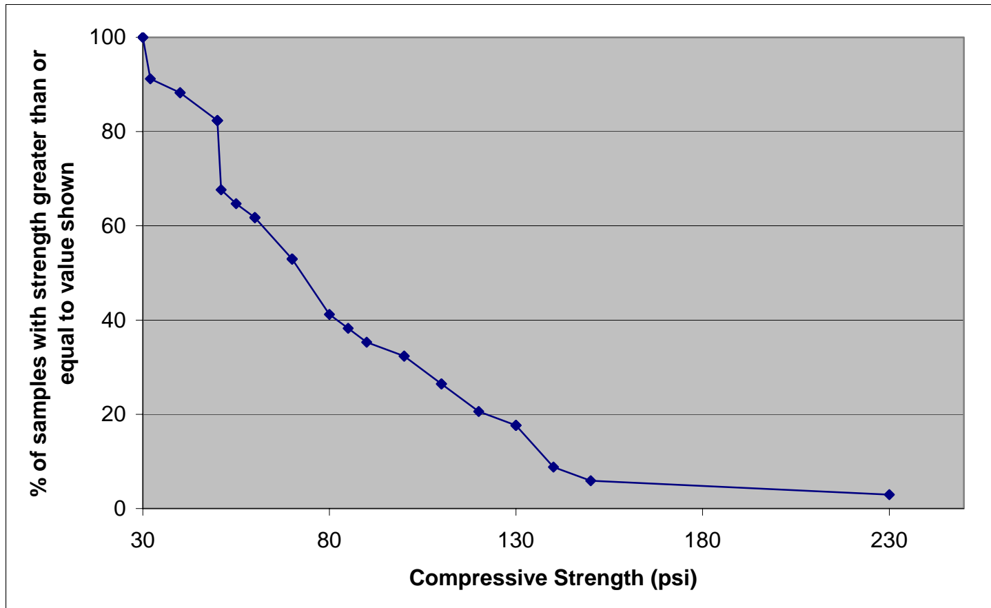
Figure 11 – Treated Soil Compressive Strength
