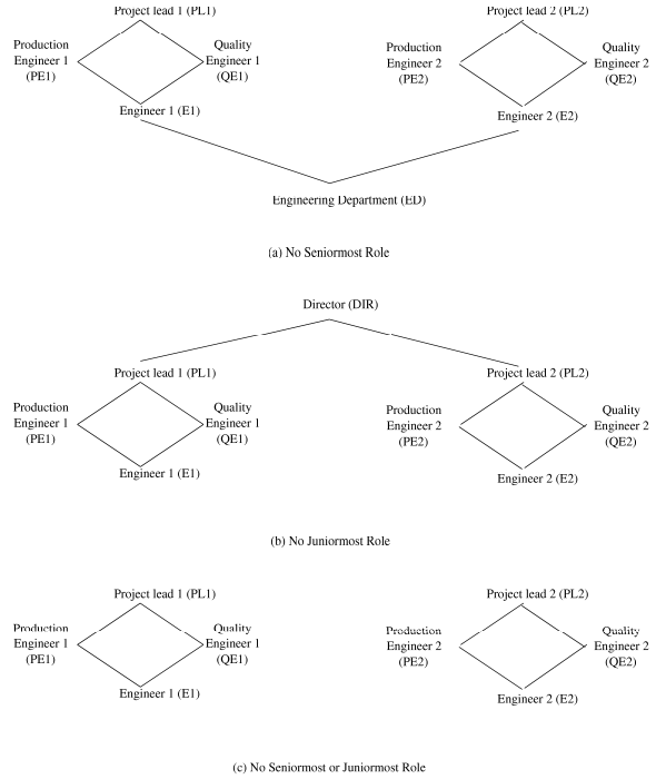
Figure 4: Example Role Hierarchies Without Seniors or Juniors Roles
