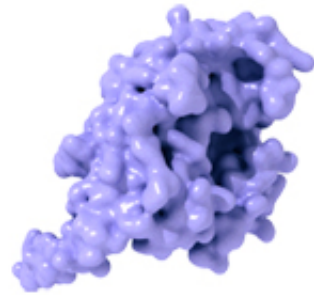
Single phenylalanine hydroxylase subunit
