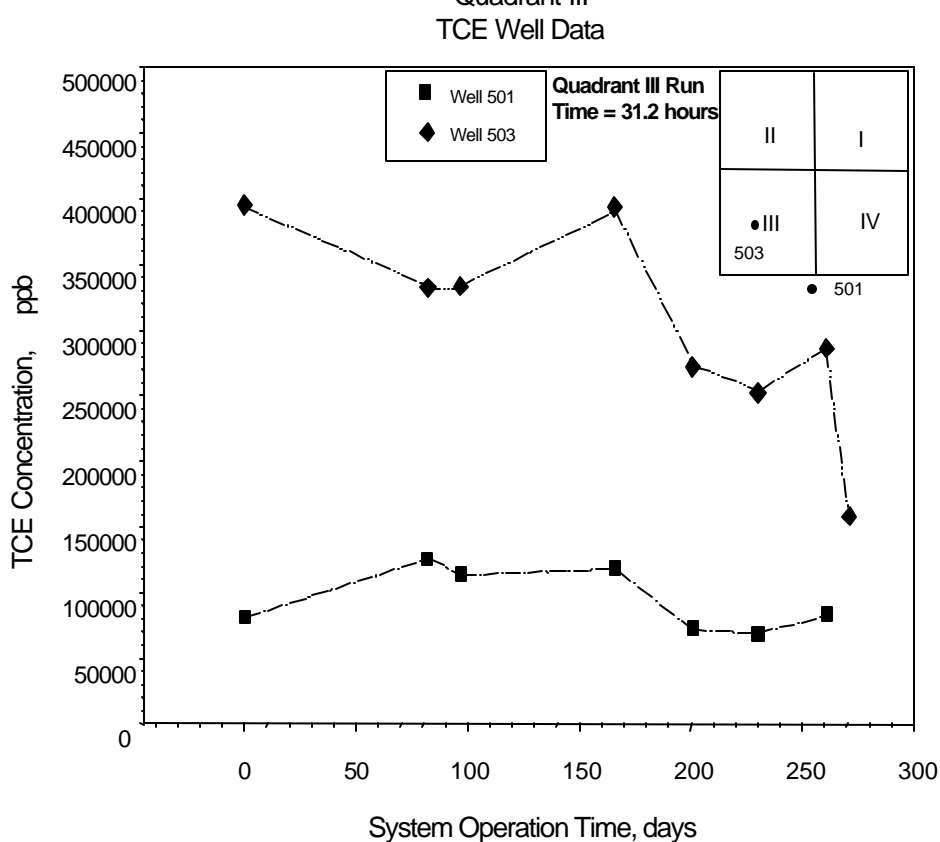
Figure 7. Quadrant 3 monitoring well results.
