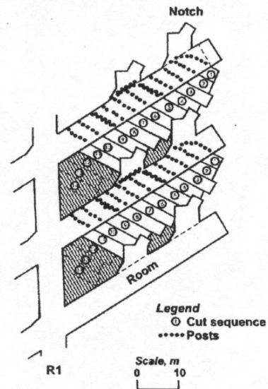
Figure 14. Pillaring plan in E19 that was changed because of floor heave
