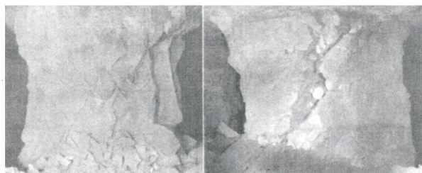
Fig. 9 Left pillar has multiple sets of discontinuities that dip at 50–70°; right pillar has two prominent discontinuities that dip at approximately 60°
