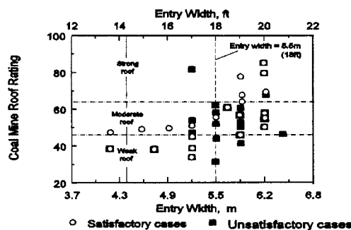
Figure 1. Relationship Between CMRR and Width at U.S. Longwall Mines (after Mark and Chase, 1994).
