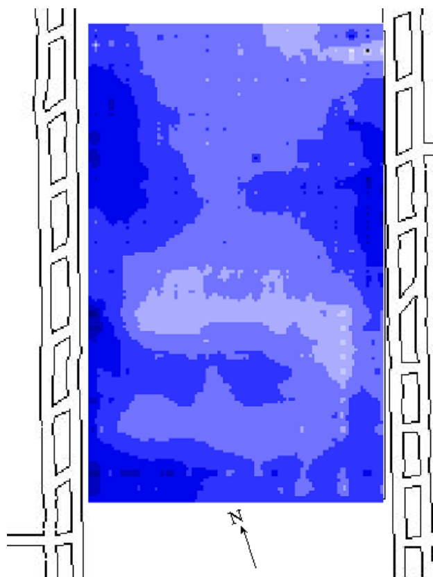
Figure 6. Shield-leg pressure distribution for six-week data set. Lighter areas indicated relatively higher loading than darker areas. Panel width is 160 m.
