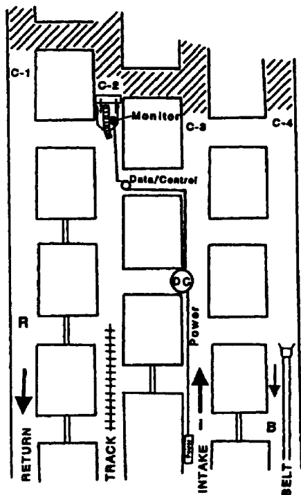
Figure 3. Location of MCRDM sensor (Monitor) and auxiliary electronics (DC) during phase one evaluation.
