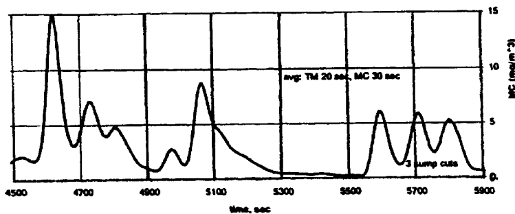
Figure 4. Dust concentrations measured by the MCRDM on 21 August 1995.
