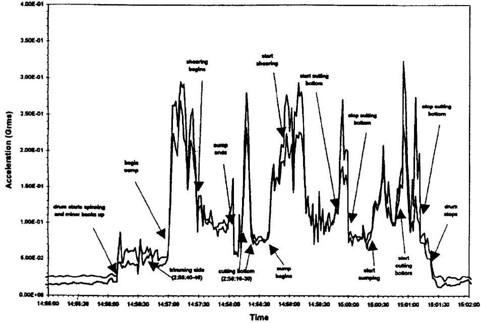
Figure 5. Vibration measured at the MMCRDM on 21 August 1995.
