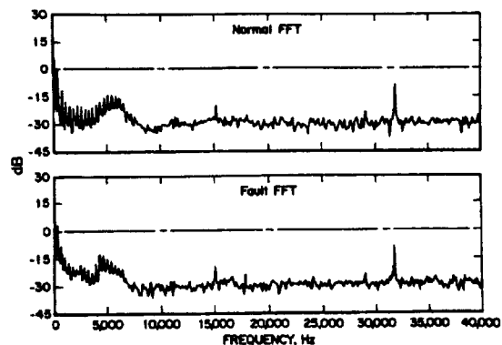
Figure 6. Comparison of normal and faulted Fast Fourier Transforms, dc to 40 kHz.
